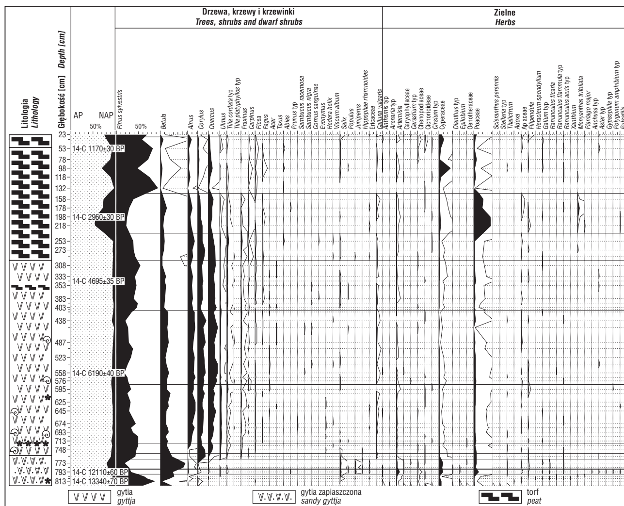
Ryc. 4. Bysławek-2. Diagram palinologiczny Fig. 4. Bysławek-2. Palinological diagram
