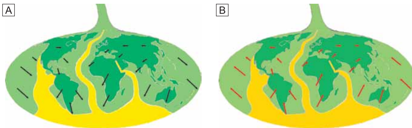
Fig. 38. A. Motion of the expanding mantle relative to the megaplate. B. Apparent motion of parts of the megaplate relative to the expanding mantle
