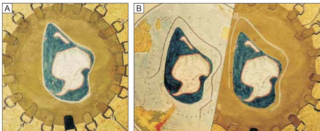
Fig. 40. Modelling of the expansion of the Antarctic plate (explanation in text)
