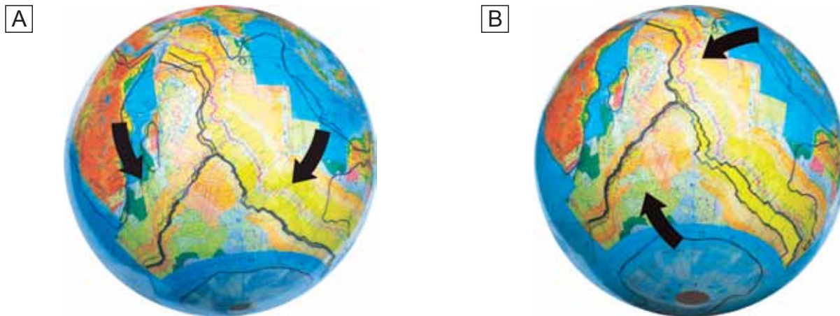
Fig. 19. A. Northwest Indian Ocean gaping gore. B. Southeast Indian Ocean gaping gore
