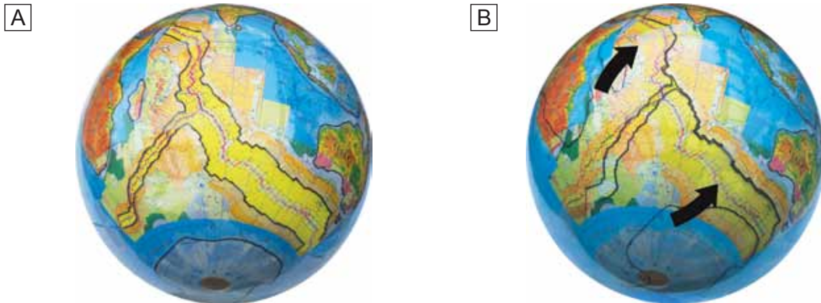
Fig. 7. Appearance of an artificial gaping gore between the African and Antarctic plates on a non-expanding Earth (explanation in text)
