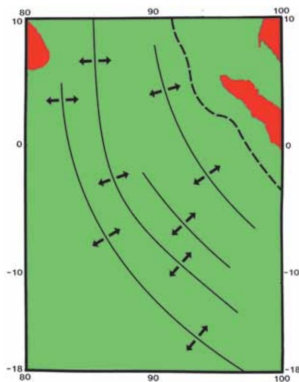
Fig. 24. Lines of tension perpendicular to Sumatra-Nicobar trench – broken line in figure (explanation in text)
