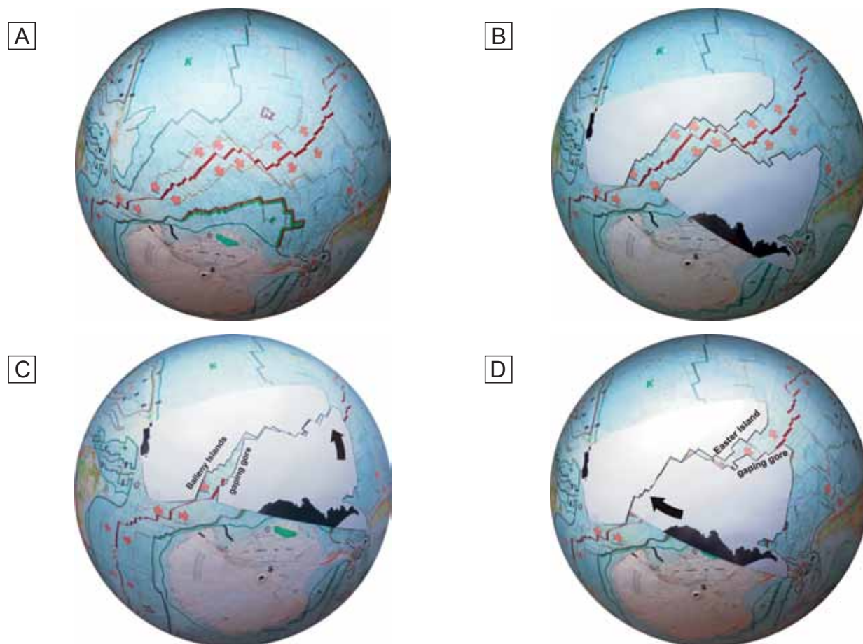
Fig. 12. Gaping gores in the southwest Pacific (explanation in text)
