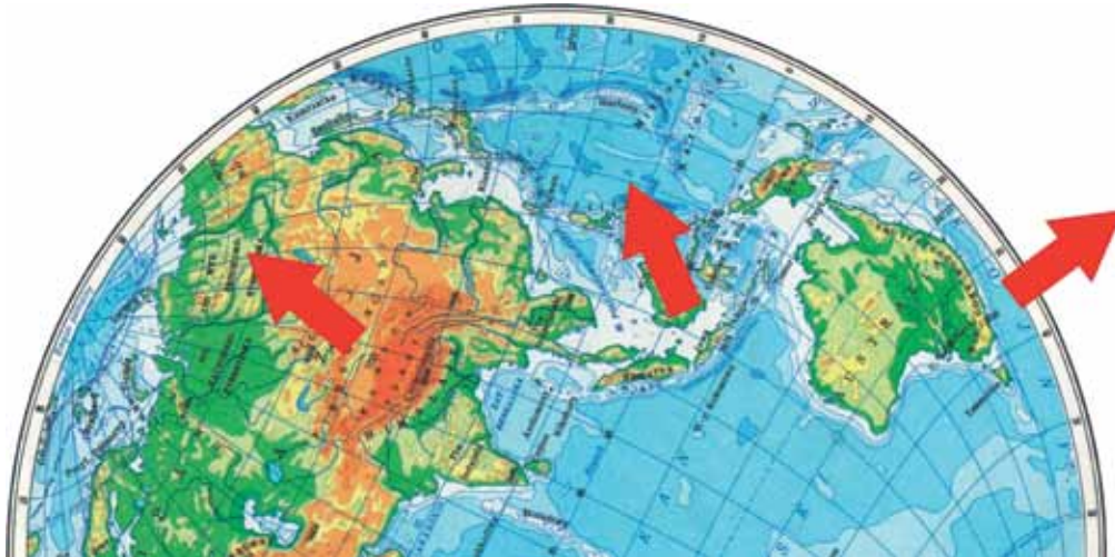
Fig. 43. Expanding Indo-Australian plate (explanation in text)
