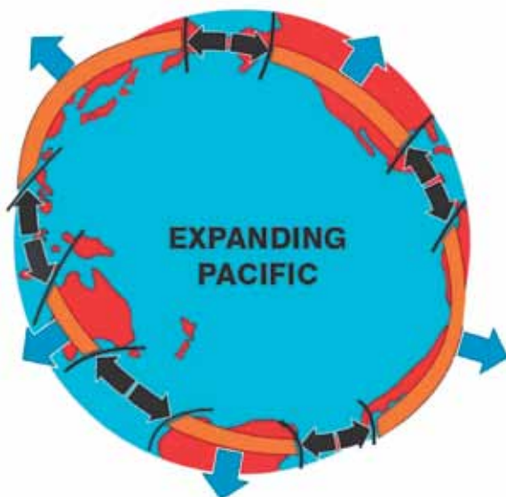
Fig. 44. Expanding Pacific after Koziar (1993) – www.wrocgeolab.pl/Pacific
