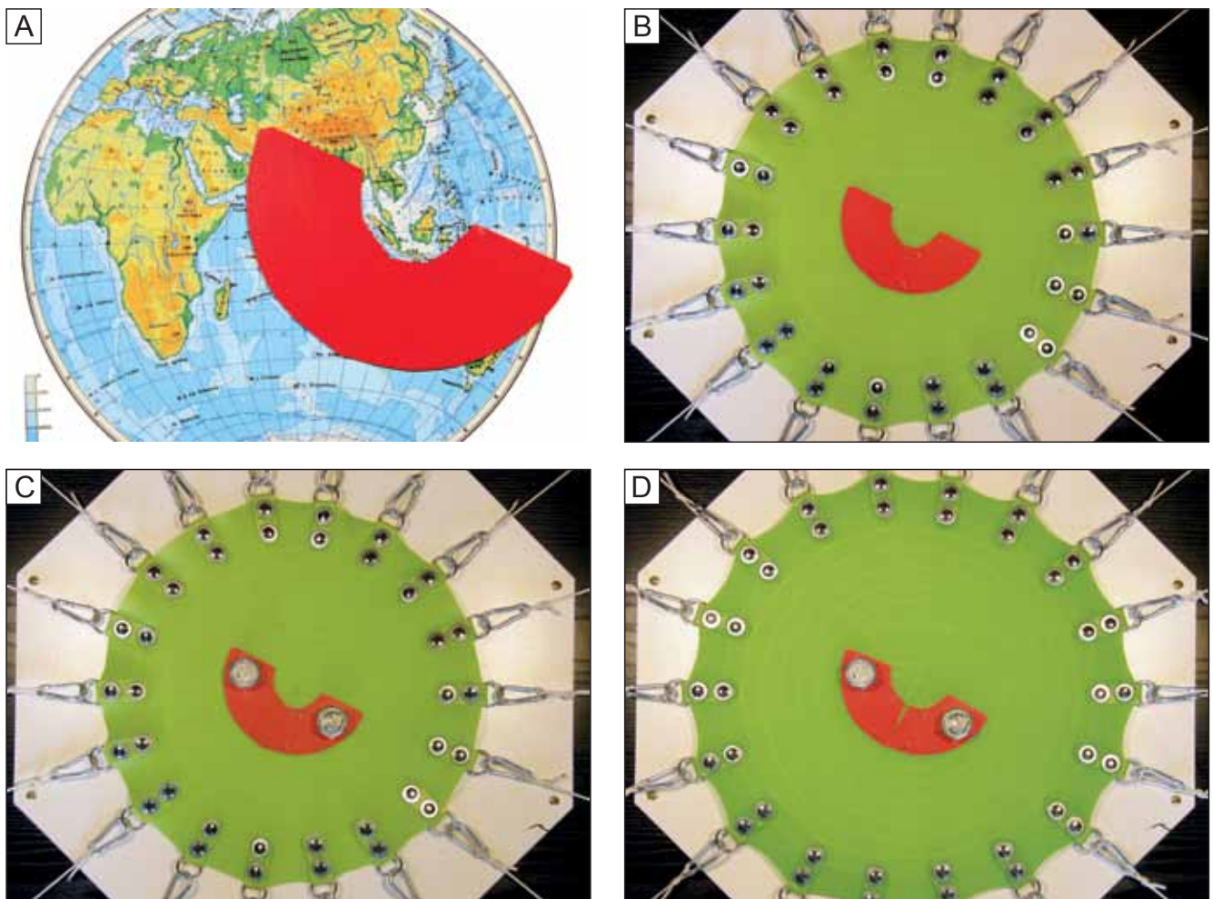
Fig. 26. Modeling of bending-out of the Indo-Australian plate on the expanding basement (explanation in text)
