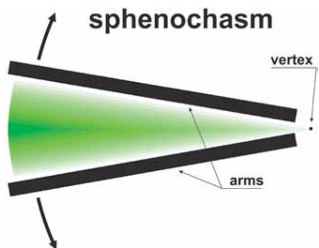
Fig. 48. Carey's sphenochasm (explanation in text)
