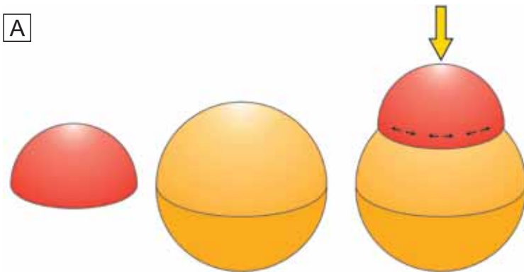
Fig. 18. A. Own model illustrating artificial stretching of the peripheral parts of Wegener’s Pangaea (explanation in the text). B. Carey’s model illustrating the origin of artificial Tethys “Ocean” as an extreme gaping gore (explanation in the text)
