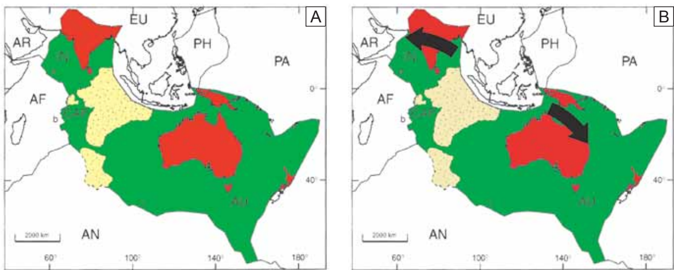
Fig. 27. Bending-out of Indo-Australian plate (explanation in text)
