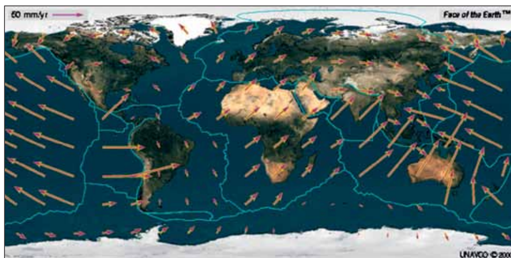
Fig. 31. Present global plate motion in NNR absolute reference frame based on geophysical data (DeMets et al. , 1994)
