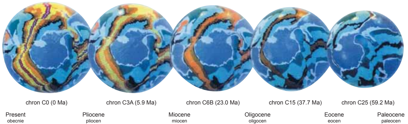
Fig. 13. Maxlow's (1995) reconstruction of Antarctic region on the expanding Earth
