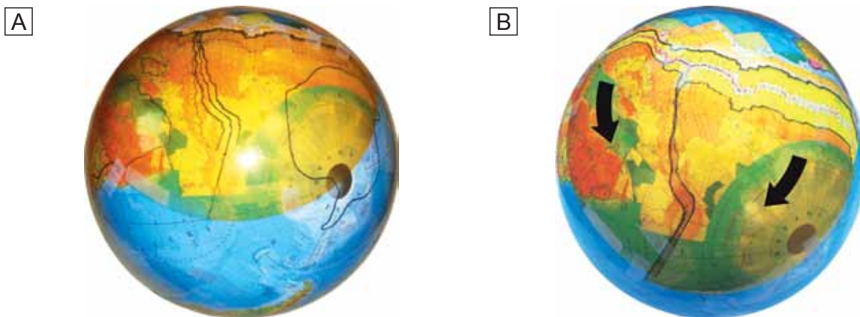
Fig. 8. Artificial convergence between the African and Antarctic plates on a non-expanding Earth (explanation in text)
