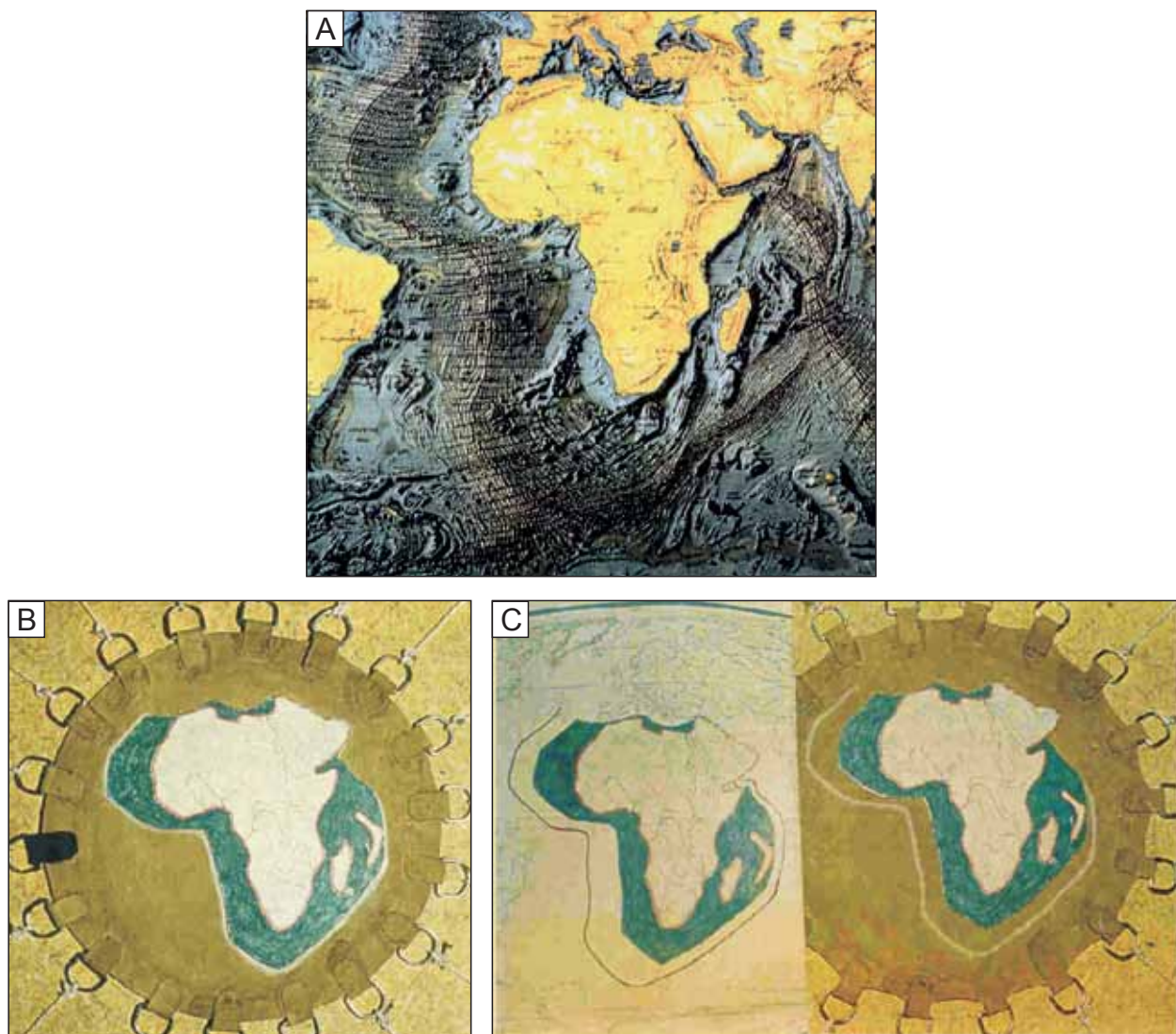
Fig. 39. Modelling of the expansion of the African plate (explanation in text)
