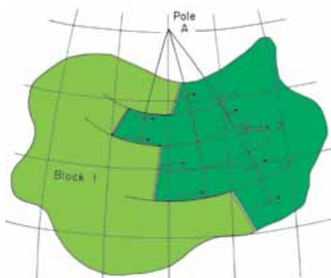
Fig. 3. Pole of rotation determined as an intersection point of great circles perpendicular to transform faults (after Morgan, 1968)
