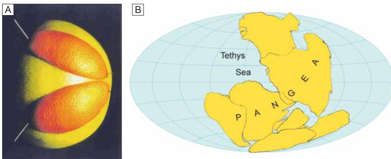
Fig. 16. A. Another possible arrangement of orange peels in style presented in Figure 14.
