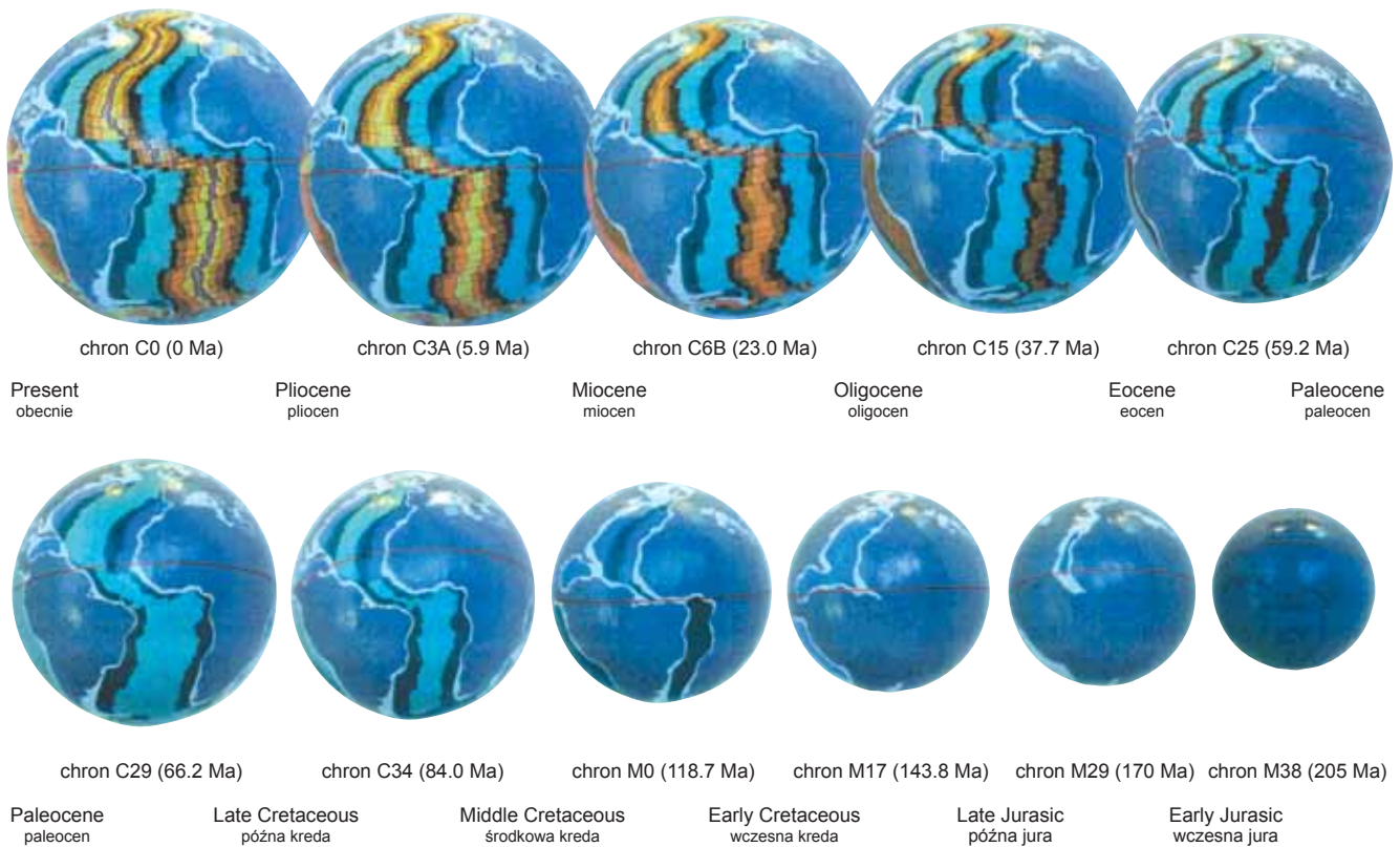
Fig. 10. Maxlow's (1995) reconstruction of the Atlantic Ocean on the expanding Earth, without gaping gores
