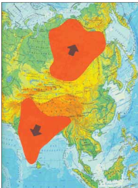
Fig. 41. Mutal moving apart of India craton and Angara shield (Koziar, 2005)
