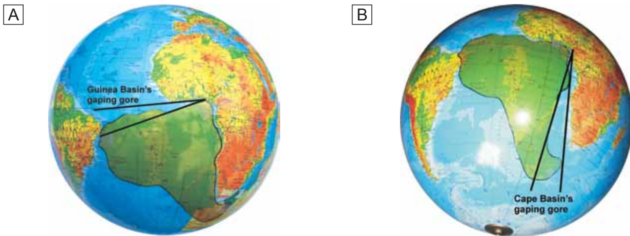
Fig. 9. Gaping gores on a non-expanding Earth
