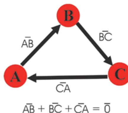
Fig. 4. Circuit built of three vectors of relative angular speeds of three plates (explanation in text)
