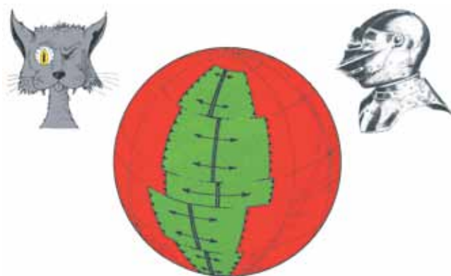
Fig. 47. Eulerian model of rifting on a non-expanding Earth – centre (Dietz, Holden, 1973)
