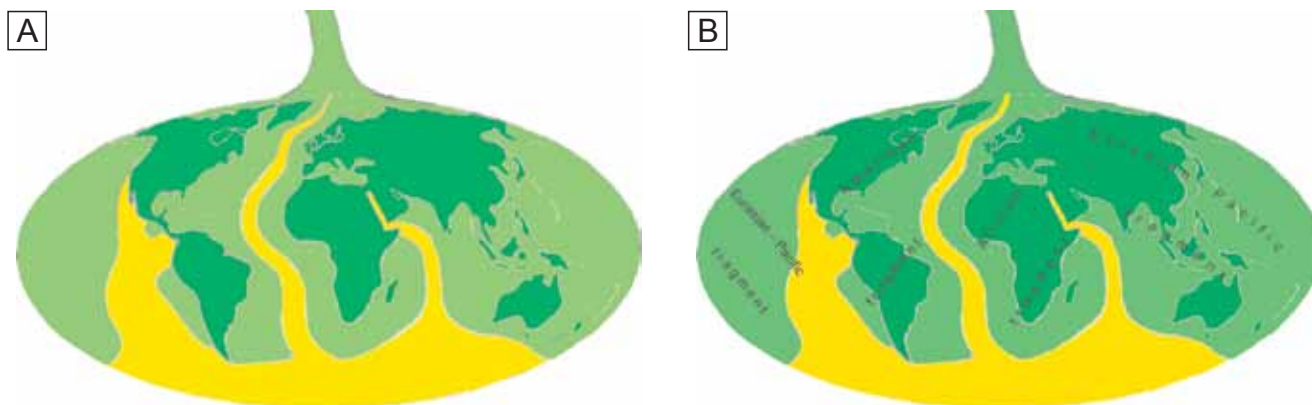
Fig. 37. A. Own model of the Arctic Paradox based on real geometry of continents and plates. B. division of the northern megaplate into three big fragments
