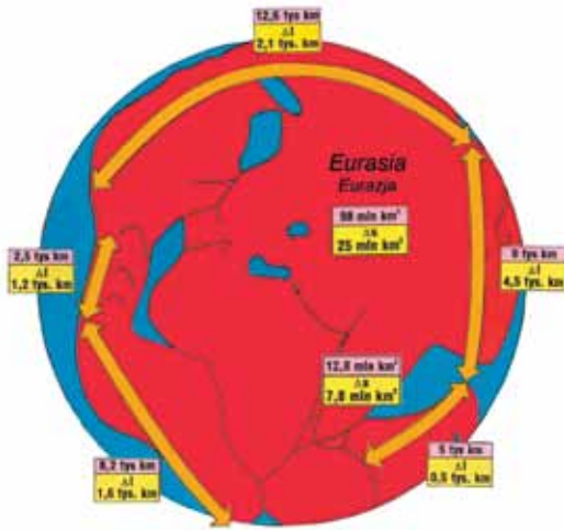
Fig. 17. Artificial stretching of the peripheral parts of Wegener’s Pangaea.
