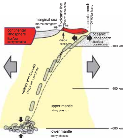
Fig. 42. Tensional development of island arc (Koziar, 2003)
