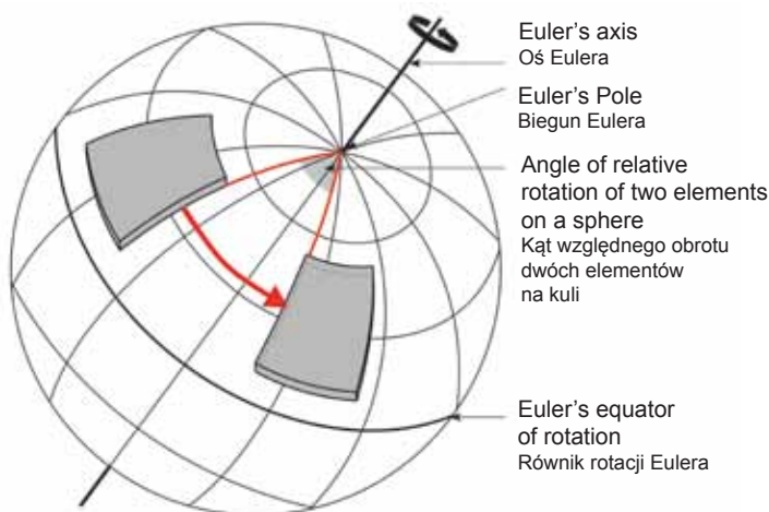
Fig. 1. Axis and pole of relative rotation of two elements on a sphere (after Kearey & Vine, 1996)
