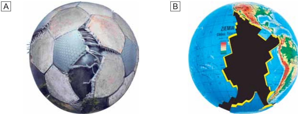
Fig. 46. A. Shabby soccer ball model of rifting on the expanding Earth. B. Pacific with removed post-Paleogene lithosphere
