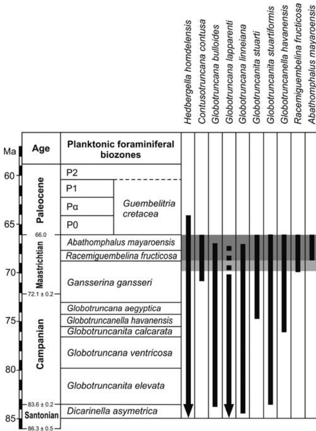
Fig. 14. Biostratigraphical ranges of the planktonic index taxa studied (modified after Gasiński and Uchman, 2009). Biozoozon combined after Robaszynski et al. (1984), Caron (1985), Robaszynski and Caron (1995), Premoli-Silva and Rettori (2002) and Premoli-Silva and Verga (2004). Time scale after Cohen et al. (2013; updated). Biozones recognized in the samples studied are marked grey.
