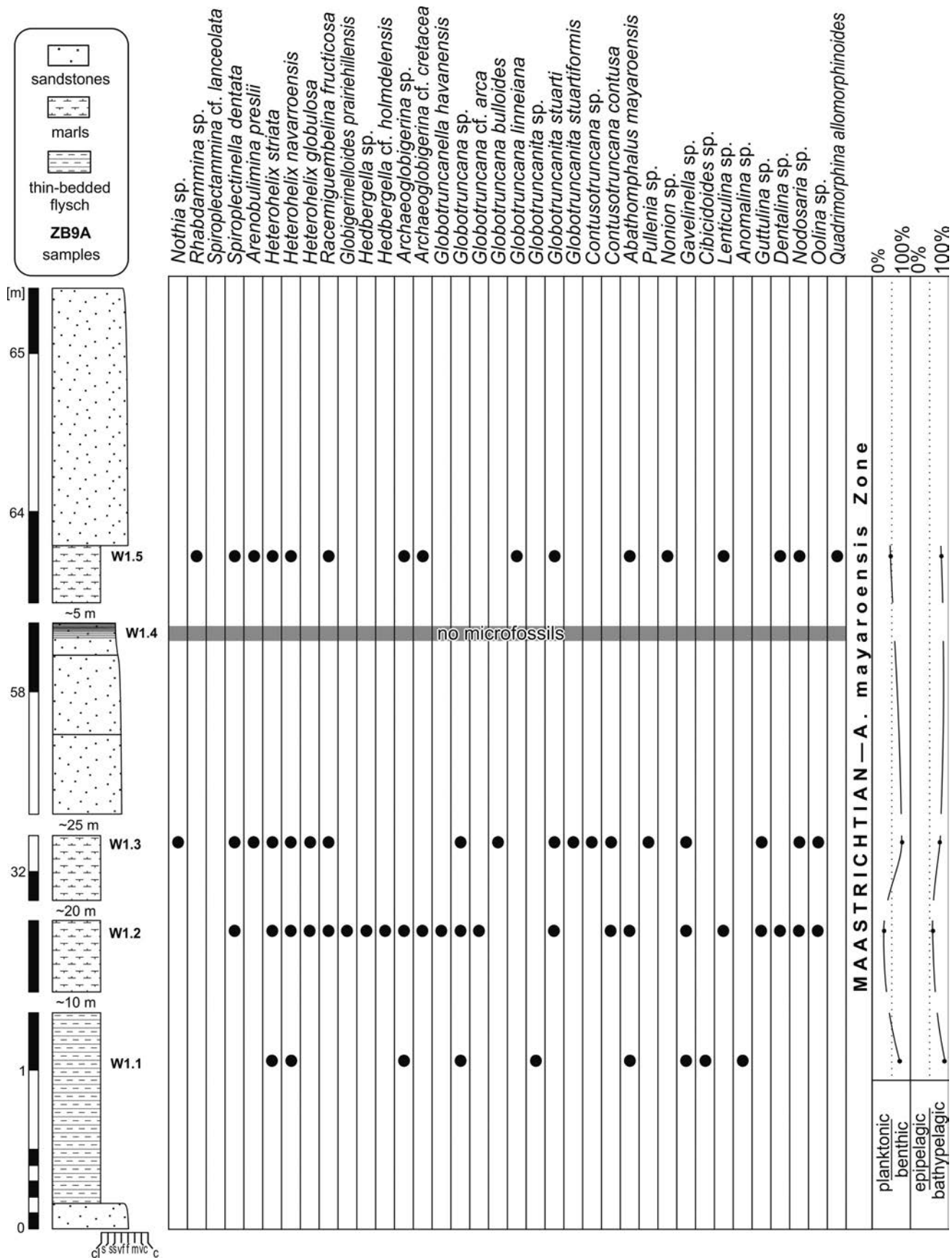
Fig. 9. Species occurrence, standard foraminiferal biozonation and quantitative analysis of foraminiferal assemblages of the samples studied from the Strug Stream.
