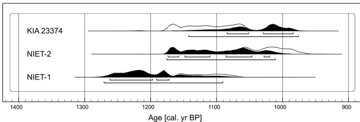
Fig. 4. Results of radiocarbon data calibration using sequence model; black-coloured distributions take into account stratigraphical order of analyzed samples in the section
