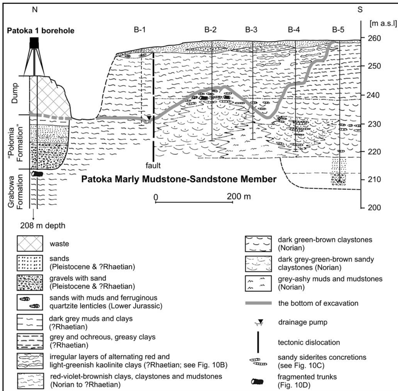
Fig. 9. Geological cross-section of the clay pit of the Patoka Brickyard, based mostly on the Patoka 1 well profile (Fig. 11) and reserve drill holes (B1–B5; after Bardziński and Chybiors, 2013)
