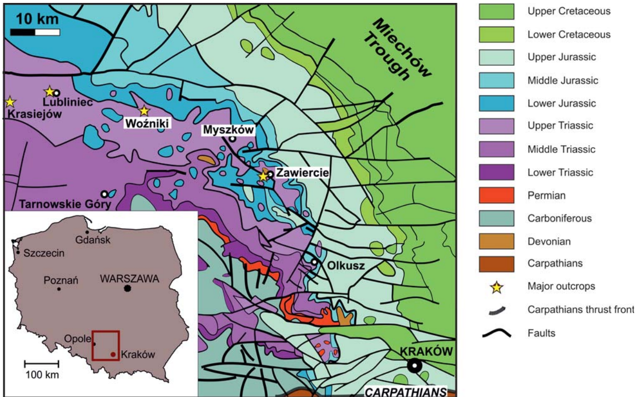
Fig. 1. Geological map of the area studied (after Marks et al. , 2006, modified; see Fig. 2 for the location details of the sections studied).
