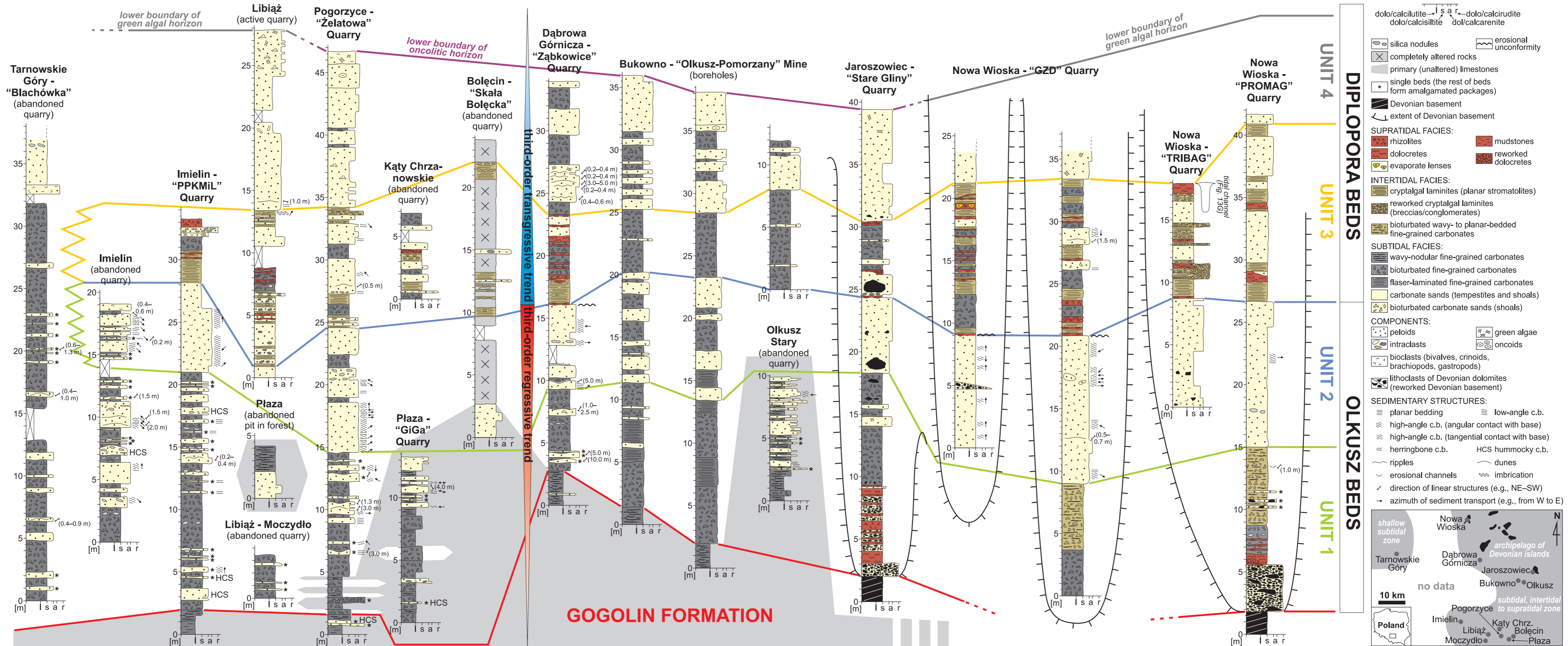
Fig. 2. Correlation of measured lithostratigraphic logs, illustrating vertical and horizontal facies changes within the “ore-bearing dolomite” succession of the Kraków-Silesia region. Unit 1 displays a marked lateral variability of lithofacies, whereas the other units are relatively uniform on a regional scale. Unit 2 and Unit 3 pinch out to the west and are absent in Tarnowskie Góry. On the right side of each log, sedimentary structures and directions of sediment transport are presented. In many sections, the lower limit of epigenetic dolomitization follows the upper boundary of the Gogolin Formation (red solid line). However, locally this limit occurs higher in the succession.
