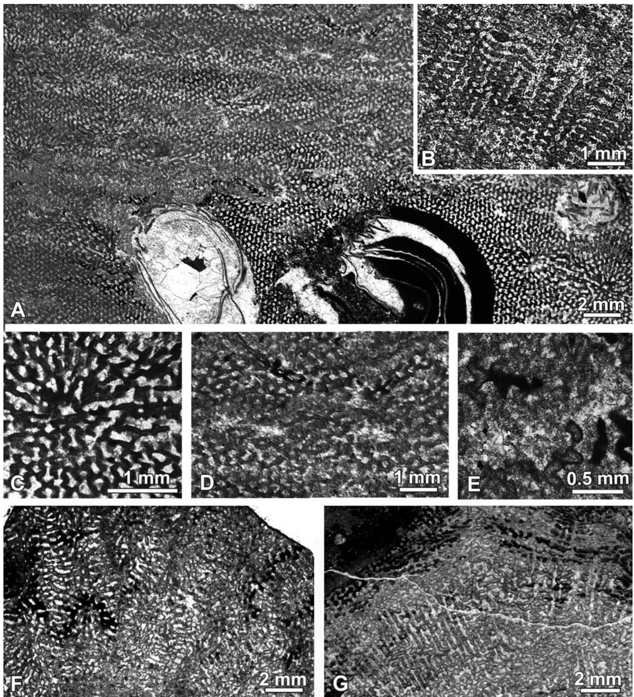
Fig. 19. A–D – Comoseris sp.: A – transverse thin section (No. 45a) of colony fragment showing corallites arranged in straight, mainly monilinear narrow series, only in places varying in width; B – longitudinal thin section (No. 45b) presenting pennular radial elements and the course of the menianes; C – detail from Fig. A, note a small columella and presence of a valley septum; D – enlarged corallite series from Fig. A. E – fragment of septo-synaptic wall occurring in places between series (thin section No. 45A). F, G – Comoseris cf. interrupta Koby: F – transverse thin section (No. 31/2a) of peripheral colony part with short corallite series arranged subradially; G – longitudinal thin section (No. 31/2b) presenting regular porous radial elements
