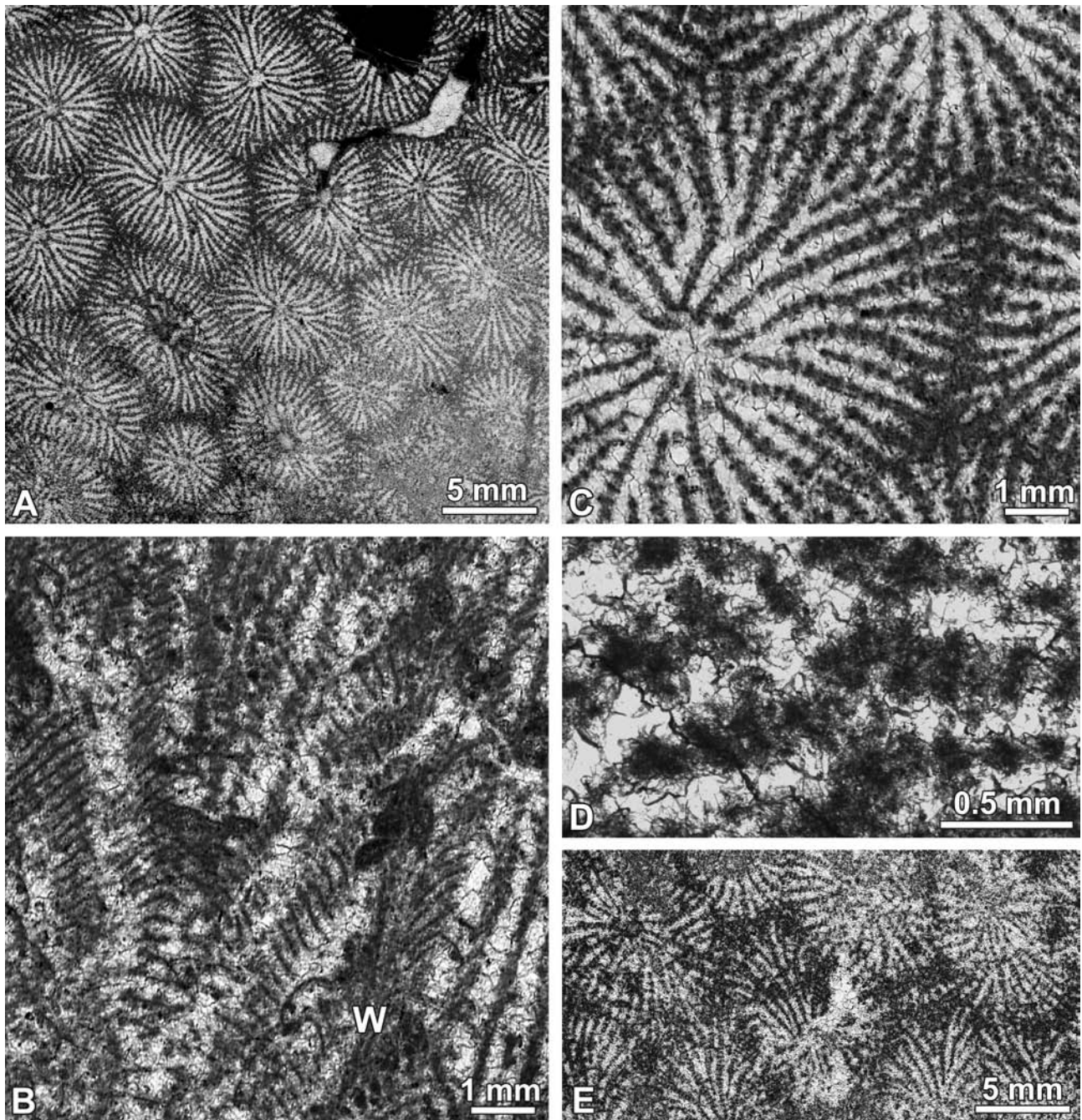
Fig. 13. A–D – Isastraea bernensis Etallon: A – transverse thin section of colony fragment (No. 34/2a); B – longitudinal-tangential thin section (No. 34/2b) showing the arrangement of trabeculae in radial elements and vesicular dissepiments in wall region (w); C – enlarged fragment from Fig. A, showing arrangement of septa and intercoralite septal parts; D – detail from thin section No. 34/2a, presented on Fig. A. Traces of septal trabeculae (black forms) and septo-paratheca well visibles. E – transverse thin section (No. 5/1a) of the same species
