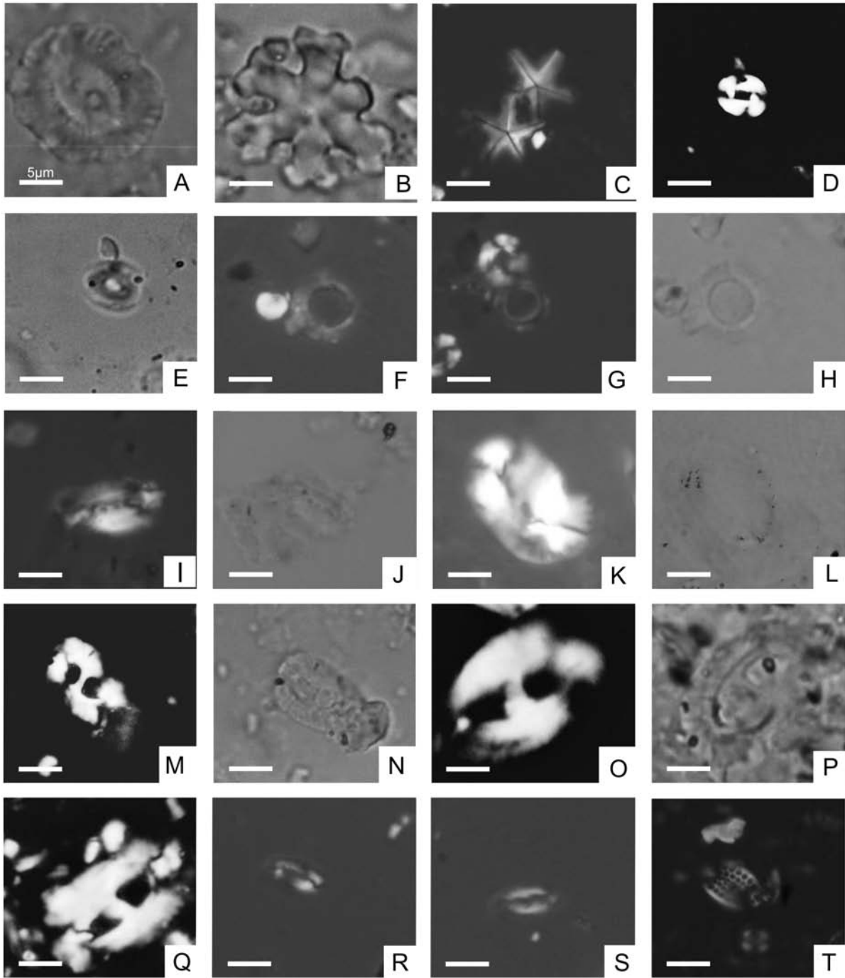
Fig. 8. Calcareous nannoplankton of the Krakowiec beds (SE Poland) and Kosiv Formation (West Ukraine). Scale bar is 5 \mu m. A – Coccolithus pelagicus (Wallich) Schiller, Krakowiec beds, Biszczka 1, depth 510.0–514.0 m; B – Discoaster deflandrei Bramlette et Riedel, Krakowiec beds, Biszczka 1, 630.0–634.0 m; C – Micrantholithus sp., Krakowiec beds, Biszczka 1, depth 540.0–544.0 m; F–H – Umbilicosphaera rotula (Kamptner) Varol, Kosiv Formation, Voloscha 1, depth 2,070.0–2,080.0 m; I, J – Helicosphaera burkei Black, Kosiv Formation, Voloscha 1, depth 2,050.0–2,060.0 m; K, L – Helicosphaera kamptneri Hay et Mohler, Kosiv Formation, Voloscha 1, depth 2,050.0–2,060.0 m; M, N – Helicosphaera mediterranea Müller, Kosiv Formation, Voloscha 1, depth 2,050.0–2,060.0 m; O–Q – Helicosphaera sellii Bukry et Bramlette, Kosiv Formation, Voloscha 1, depth 2,050.0–2,060.0 m; R, S – Helicosphaera walbersdorfensis Müller, Kosiv Formation, Voloscha 1, depth 2,050.0–2,060.0 m; T – Pontosphaera multipora (Kamptner) Roth, Kosiv Formation, Makuniv 1, depth 1,681.0–1,688.6 m
