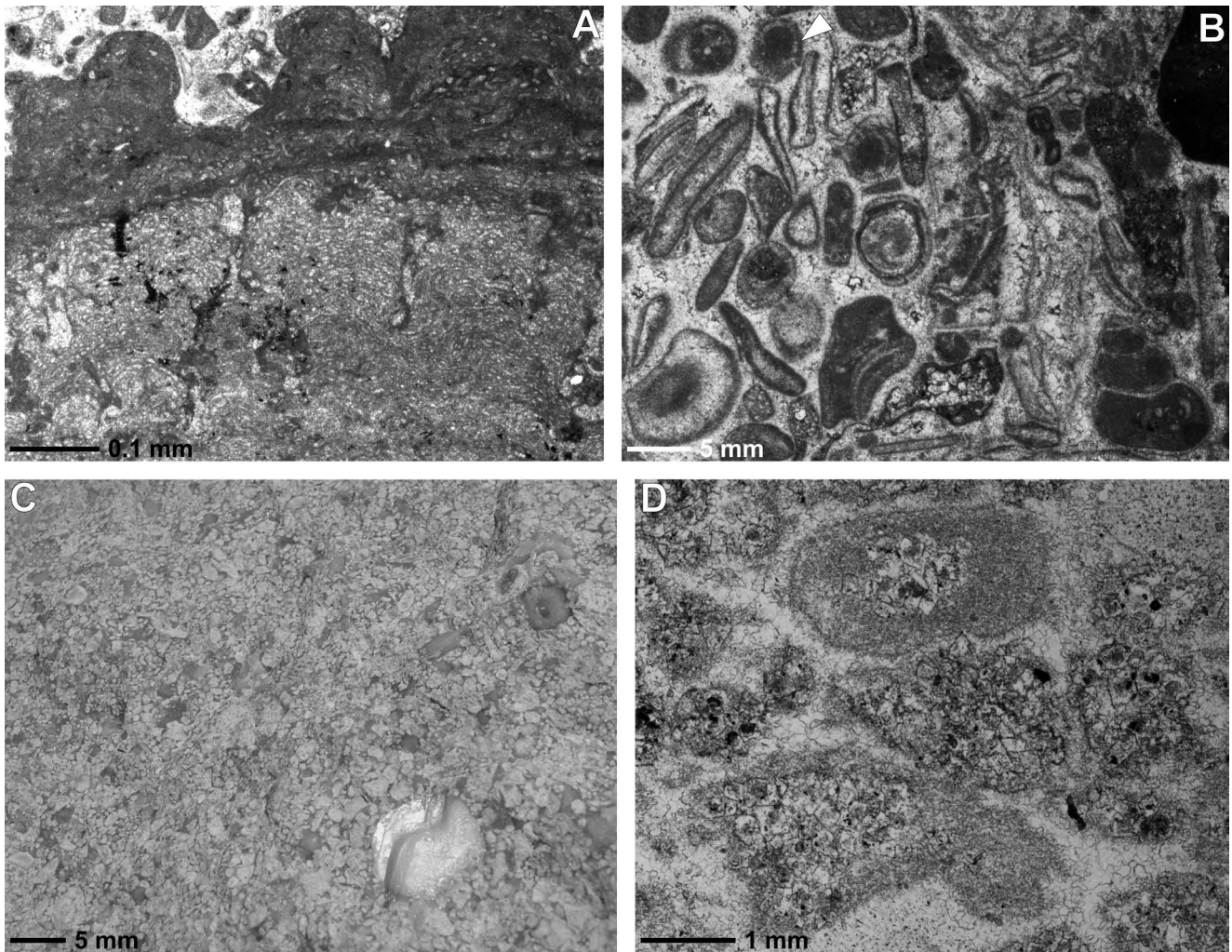
Fig. 14. Extremely shallow-water deposits, capping reefs in the western area. A. Thin section of Girvanella oncooid. Tarnów Opolski; B. Skeletal grainstone with dispersed ooids (white arrow) and gastropods. Thin section. Tarnów Opolski; C. Peloidal grainstone with scarce crinoids. Kamień Śląski; D. Detail of C. Partly dolomitized peloids. Thin section
