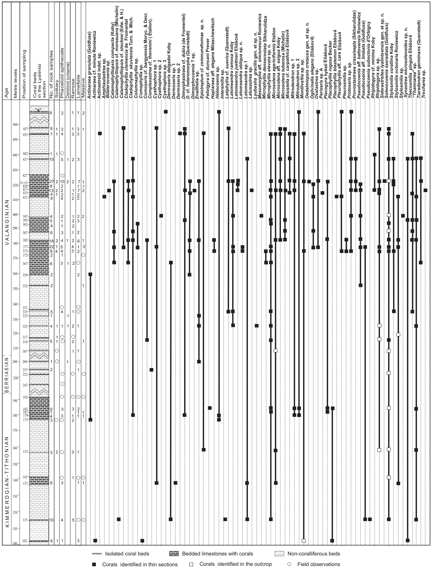
Fig. 2. Distribution of corals in the Lyalintsi section, Kimmeridgian–Valanginian. Details of the numbers of coral taxa in respective growth form categories, and sample are given in the left-hand columns
