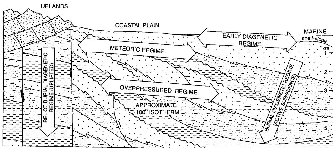
Fig. 2. Generalized distribution of diagenetic regimes in a continental margin, terrigenous clastic sedimentary basin such as the Beaufort–Mackenzie Basin. Coarsely stippled areas represent coarse clastic sediments; darker patterns represent finer grained mudstones and shales
