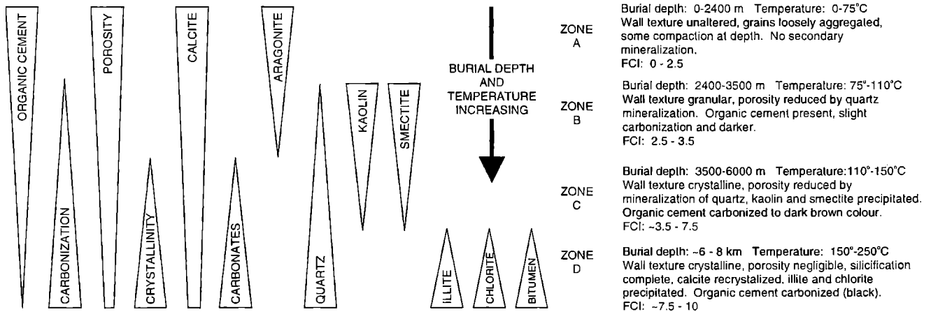
Fig. 7. Zonation of burial diagenetic trends in foraminifers related to approximate temperatures, burial depths, and Foraminiferal Colouration Index (FCI) (modified from McNeil et al. , 1996)
