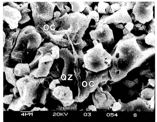
Fig. 5. Quartz grains (QZ) with remnants of organic cement (OC) in the wall of Bathysiphon , GSC 109545, after etching in dilute hydrofluoric acid
