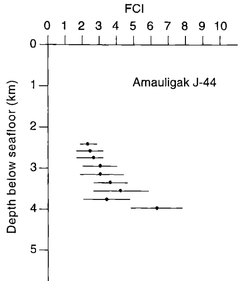
Fig. 6. Plot of FCI data versus depth in the Amauligak J-44 well, see Table 2 for raw data. (from McNeil et al. , 1996) Note: sample at 3797 m with anomalously low FCI average value of 3.28 represents caved well cuttings
