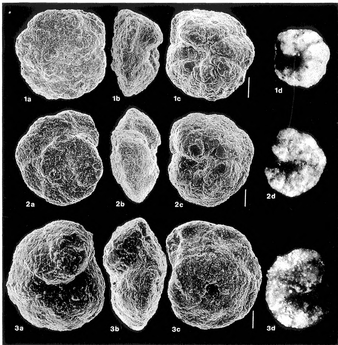
Fig. 7. SEM and reflected light photographs (magnifications as on original). 1a-d – Ammonoanites ingerlisae Gradstein & Kaminski, n.sp., holotype, Conoco 211/19-1 at 5840 ft (1d x 140); 2a-d – Ammonoanites ingerlisae Gradstein & Kaminski, n.sp., Conoco 211/19-1 at 5840 ft (2d x 140); 3a-d – Ammonoanites ingerlisae Gradstein & Kaminski, n.sp., Lizard Springs, Trinidad (3d x 140). Length of scale bar – 50 \mu m
