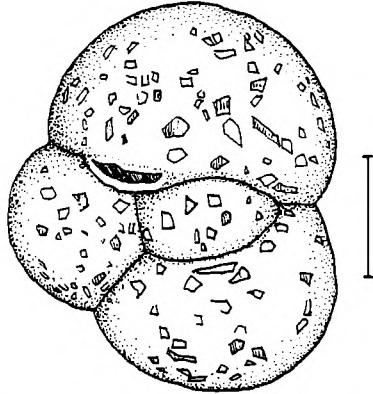
Fig. 11. Paratype of Praecystamina sveni n.sp.: ODP Hole 643A, Vøring Slope. Sample 643A-56X-3, 56–61 cm. Length of scale bar – 100 \mu m. Redrawn after Kaminski et al. (1990)
