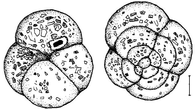
Fig. 9. Paratype of Conotrochammina voeringensis Gradstein and Kaminski, n.sp.; ODP Hole 643A, Vøring slope. Sample 643A-52X-1, 83–88 cm. Length of scale bar – 40 \mu m. Redrawn after Kaminski et al. (1990)
