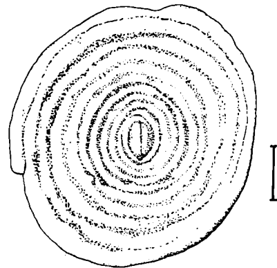
Fig. 2. Holotype of Annectina biedai Gradstein and Kaminski, n.sp.; Saga 2/2-4 well at 1900 m. Length of scale bar – 100 \mu m
