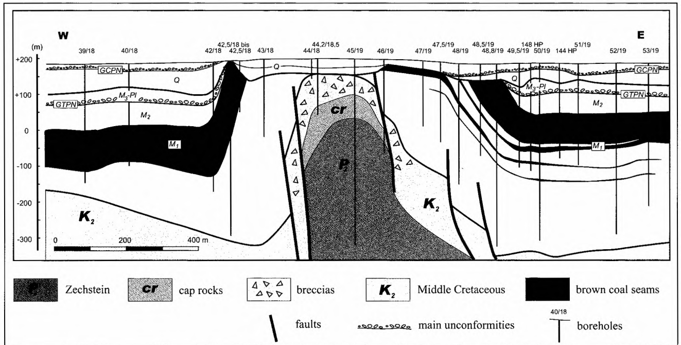
Fig. 3. Geological section across the Dębina Salt Dome area, two times exaggerated. Q – Quaternary; M 3 -Pli – Late Miocene to Pliocene; M 2 – Middle Miocene; M 1 – Early Miocene; GCPN – main Quaternary unconformity; GTPN – main Tertiary unconformity
