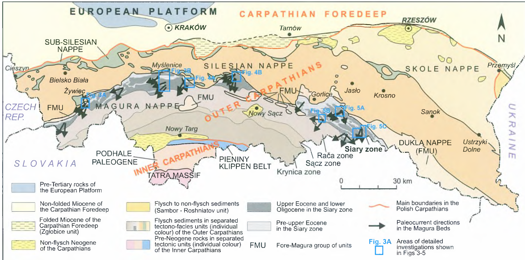
Fig. 1. Regional and structural context of the study area according to the Tectonic Map of Poland (Znosko, ed., 1998) with Leszczyński's modifications for the southern boundary of the Siary zone
