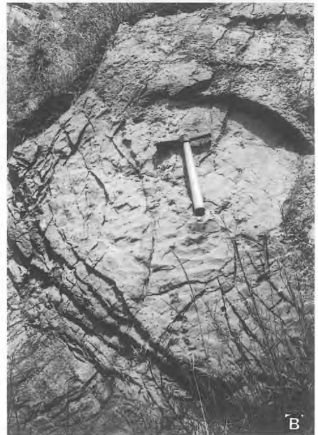
Fig. 6. A. Bioheroglyphs (a – Tiggilites sp.; b – Planolites sp.); B – interference ripplemarks on bedding planes of the Kleczańów Sandstone Member of the scale IV
