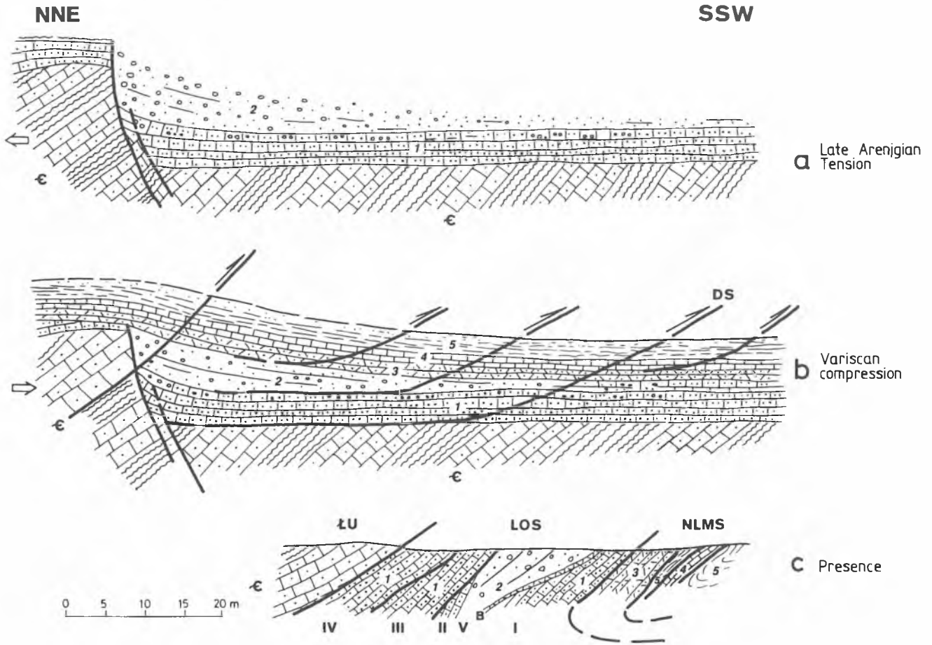
Fig. 12. Tectonic evolution of the Międzygórz area. a. Formation of the Chełm Conglomerate as results of the Lower Ordovician tectonic movements; b. Development of scales of the Lower Ordovician sequence as a results of Variscan compression; c. Tectonic position of the Lower Ordovician scales. \epsilon – Cambrian sandstones and shales; I to IV scales; 1 – The Kleczanów Sandstone; 2 – the Chełm Conglomerate; 3 – the Dyminy Orthid Sandstone; 4 – the Mójcza Limestones; 5 – Silurian shales; B – tectonic breccia; DS – Decollement surface; ŁU – Łysogóry Unit; LOS – Lower Ordovician Scales; NLMS – Northern Limb of the Międzygórz Syncline
