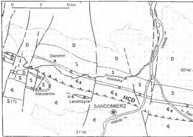
Fig. 1. Geological map of the eastern part of the Holy Cross Mountains (After Pożaryski and Tomczyk, 1993, generalized). HCD – Holy Cross Dislocation; \epsilon – Cambrian; \epsilon_3 – Upper Cambrian; O – Ordovician; S – Silurian; D – Devonian; uninterrupted and interrupted thick lines – faults; dotted lines and dotted area – extent of Tertiary of the Opatówka River; big black circle – borehole
