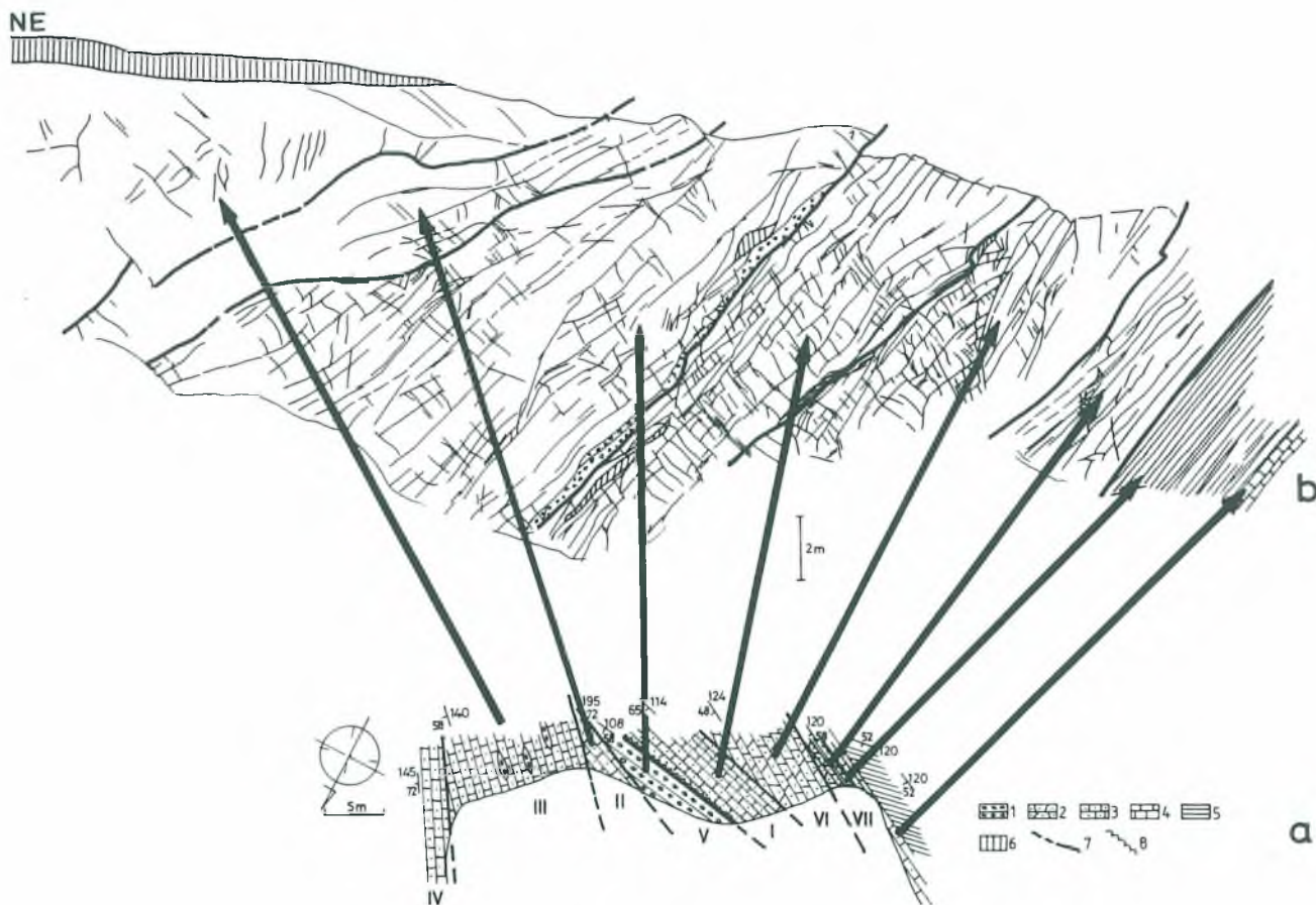
Fig. 3. General view of the main wall of the Międzygórz quarry based on photographic images (b) and the present author's sketch-plan (a). 1 – Chełm Conglomerate Member; 2 – Dyminy Orthids Sandstone Member; 3 – Kleczanów Sandstone Member; 4 – Mokradle Dolomite Member; 5 – Lower Silurian shales; 6 – loes; 7 – fault; 8 – overlapping zone; I–IV – scales of the Kleczanów Sandstone Member; V – scale of the Chełm Conglomerate Member; VI – scale of the Dyminy Orthid Sandstone Member; VII – scale of the Mójcza Limestones Formation
