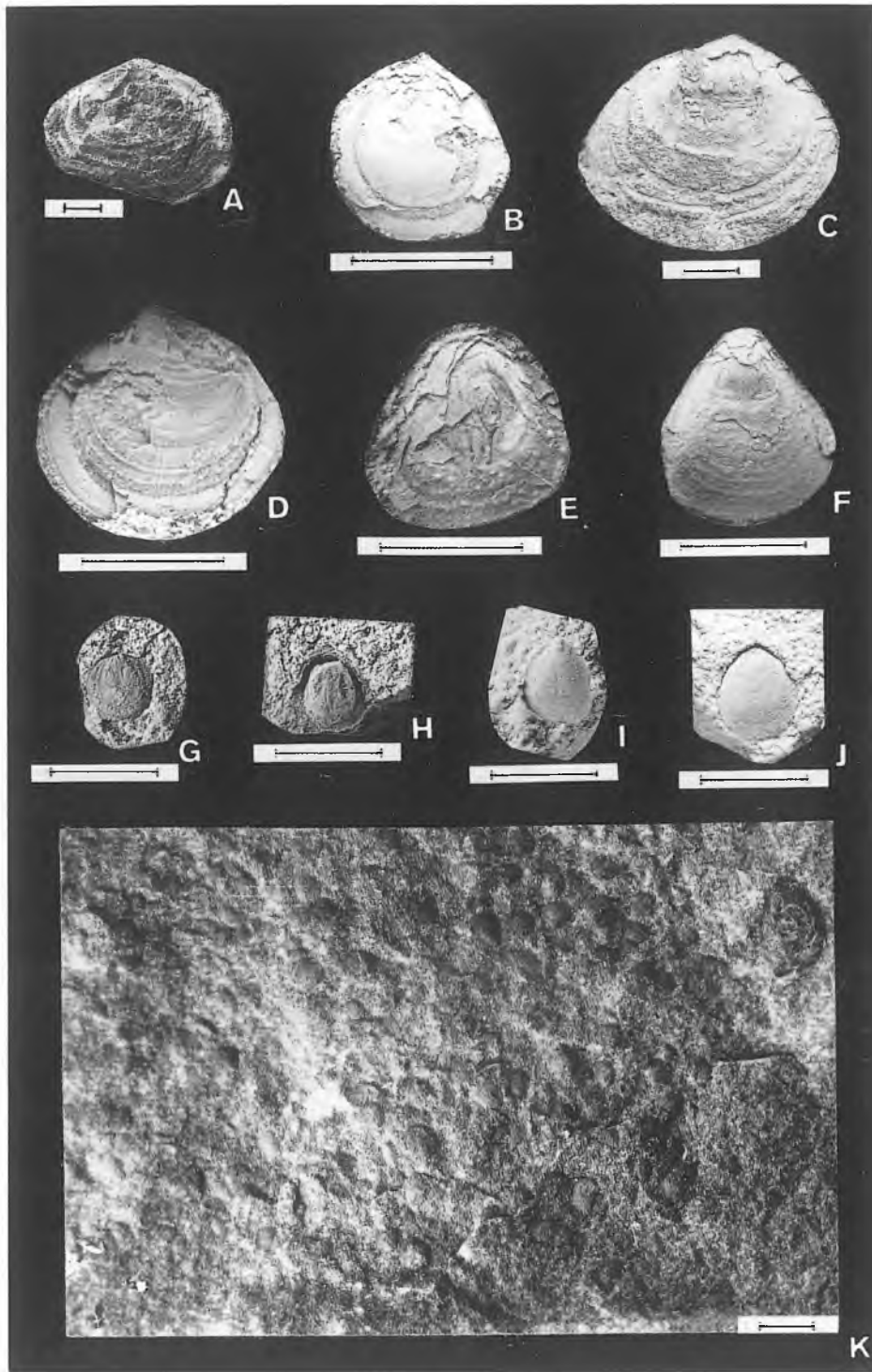
Fig. 9. Brachiopods from the Kleczanów Sandstone Member of the Międzygórz quarry and from the Zbilutka Siltstone and Chalcodonite and the Koziel Conotreta Siltstone members of the Bardo Syncline. Thysanotos siluricus (Eichwald, 1840): A, C – moulds of ventral valve, Międzygórz quarry. Rosobolus robertinus (Havlicek, 1982): B, D – partly peeled ventral valves, Międzygórz quarry. E, F – moulds of ventral valves, Szumsko. Celdobolus mirandus (Barrande, 1879): G – mould of ventral valve, Koziel; H – mould of dorsal valve, Koziel; K – moulds and casts of ventral and dorsal valves, Międzygórz. ? Pidiobolus cf. minimus Mergl, 1995: moulds of ventral valves, I – mould of ventral valve, Koziel; J – mould of ventral valve, Szumsko. Scale bars 5 mm
