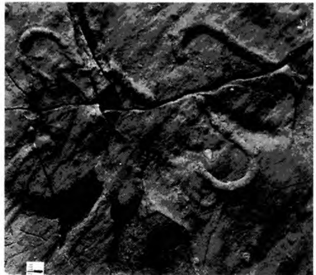
Fig. 82. Helminthopsis abeli Książkiewicz on sole of turbiditic sandstone bed. UJ TF 255, Inoceranian beds (Senonian–Paleocene), Łodzinka. Scale in mm
