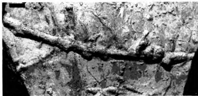
Fig. 14. Strobilorhaphic glandifer Książkiewicz. Sole of turbiditic sandstone bed. UJ TF 1510, Tylmanowa (lithostratigraphic unit unknown, label lost). Scale bar = 1 cm
