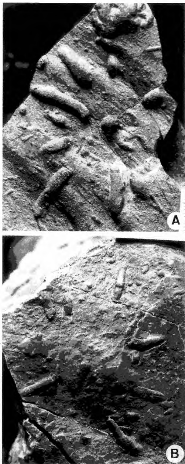
Fig. 42. Capodistria vettersi Vialov, soles of turbiditic sandstone beds. A. UJ TF 96, Lower Godula beds (Cenomanian), Jaroszewiec. B. UJ TF 958, Ropianka beds (Senonian–Paleocene), Kąclowa. Scales in mm
