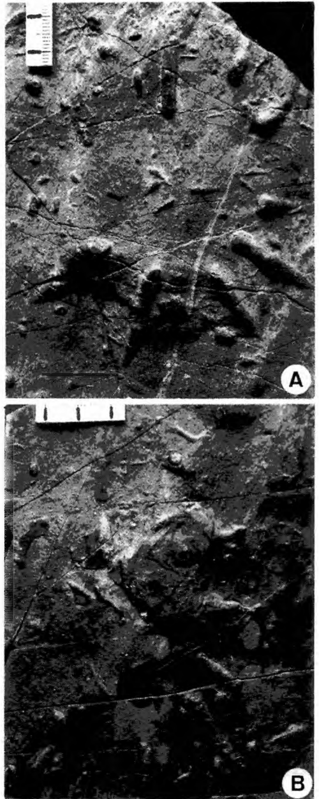
Fig. 40. Lorenzinia nowaki (Książkiewicz), soles of turbiditic sandstone beds. A. UJ TF 655, Ropianka beds (Senonian-Paleocene), Limanowa. B. UJ TF 1154, Inoceranian beds (Senonian-Paleocene), Szczawa. Scale in mm
