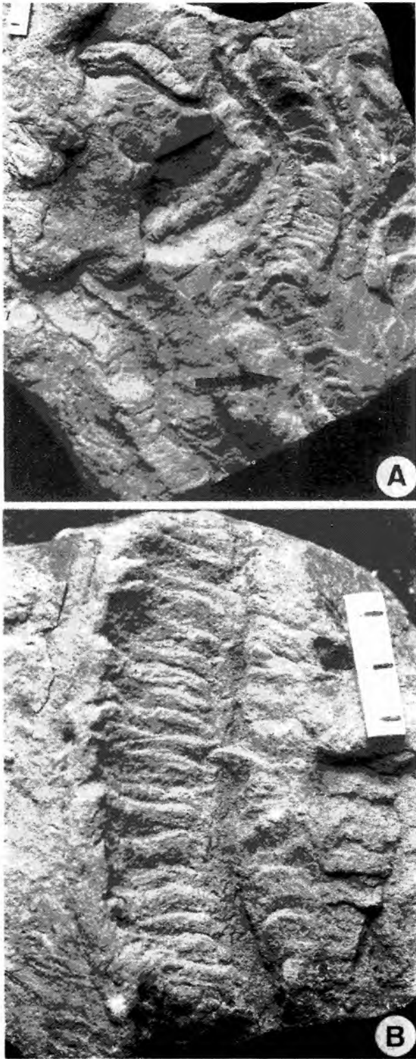
Fig. 58. Scolicia vertebralis Książkiewicz (= Scolicia ?prisca ) in turbiditic sandstone beds. A. UJ TF 1478, holotype, Inoceranian beds (Senonian–Paleocene), Bachów. Transition to S. prisca arrowed. B. UJ TF 624, Lower Istebna beds (Senonian), Czchów. Scales in mm
