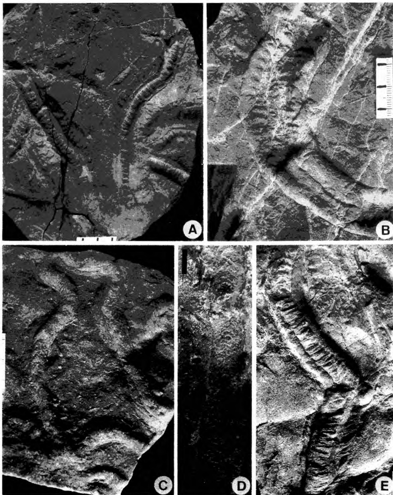
Fig. 57. Scolicia prisca de Quatrefages in turbiditic sandstone beds. A. UJ TF 626, Beloveža Formation (Eocene), Zubrzyca Górna. Epichnial view of ventral interior. B. UJ TF 1565, Hieroglyphic beds (Eocene), Zawoja, Końskie. Epichnial view of dorsal interior (upper part) and dorsal exterior (lower part). C-D. Hypichnial view of ventral exterior (slightly eroded). C. UJ TF 2548 (label lost). D. UJ TF 2546, Variegated Shale (Paleocene–Eocene), Kałowa. E. UJ TF 631, Hieroglyphic beds (Eocene), Juszczyń. Epichnial view of interior. Scale in A in cm, scales in B–C in mm, scale bar in D = 1 cm, scale bar in E = 16 mm
