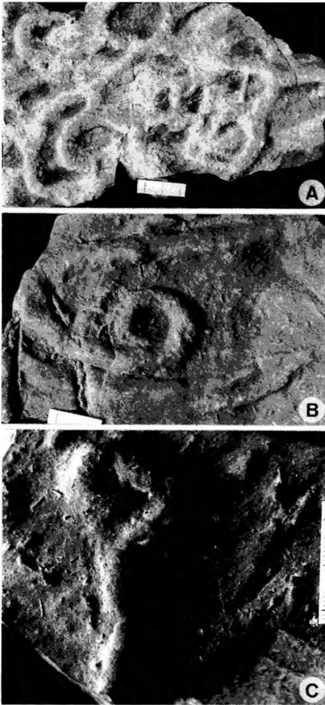
Fig. 86. “ Spirophyucus ” bicornis (Heer) on soles of turbiditic sandstone beds. A. UJ TF 590, Hieroglyphic beds (Eocene), Grzechynia (labelled as Spirophyucus convolutus ). B. UJ TF 1024 (labelled as Spirophyucus caprinus , part of label lost). C. UJ TF 796, Hieroglyphic beds (Eocene), Tokarnia (labelled as Spirophyucus caprinus ). Scales in mm
