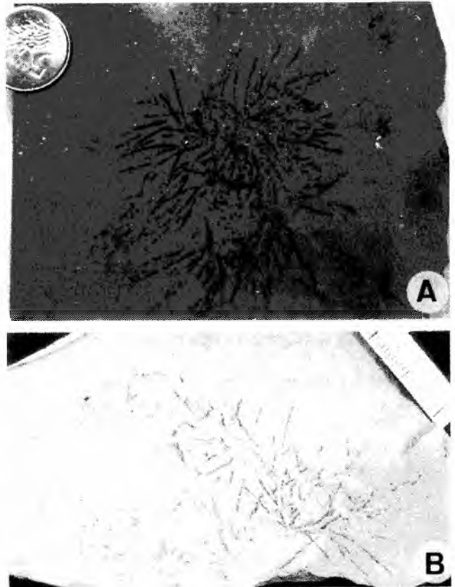
Fig. 19. Chondrites intricatus (Brongniart) with deformed filling. A. Specimen from the Gebhard's collection in the Naturhistorisches Hofmuseum in Vienna. Bisamberg near Langenersdorf. ?Cretaceous flysch of the Wienerwald. The coin is 19 mm in diameter. B. UJ TF 961, endichnial form, Ropianka beds (Senonian–Paleocene), Biała Wyżna (labelled as Bostricophyton pantanellii ). The coin in A is 19 mm in diameter, scale for B in mm
