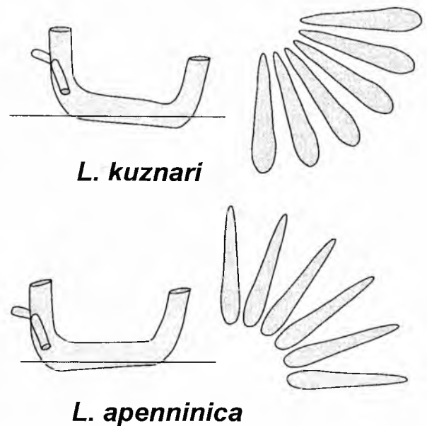
Fig. 33. Model of Lorenzina kuznari and L. apenninica in relation to inclination of the radiating elements of the burrow system
