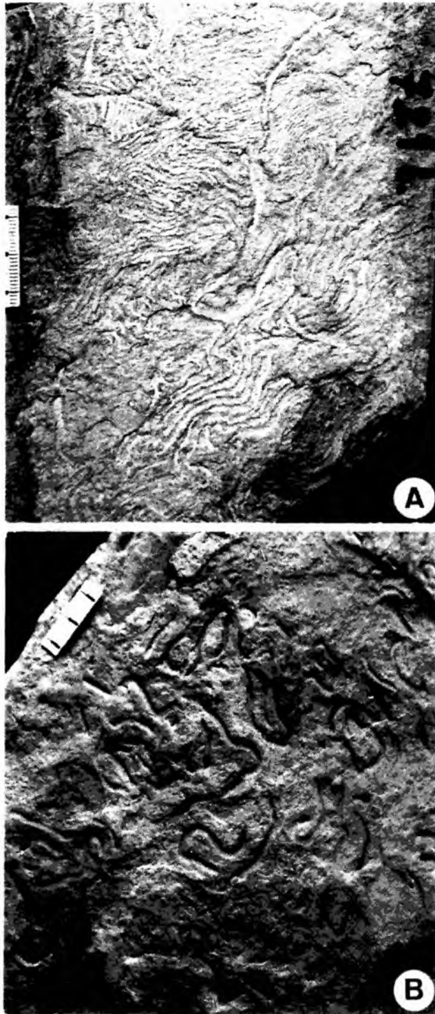
Fig. 56. Nereites irregularis (Schafhäütl), endichnial forms, epichnial view. A. UJ TF 721 (label lost). B. UJ TF 132. Sromowce beds (Senonian), Jaworki, Skalski stream. (Labelled as Helminthopsis irregularis ). Scales in mm
