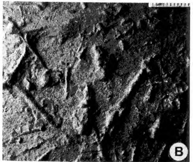
Fig. 4. Arthrophyucus strictus Książkiewicz (arrowed) and Arthrophyucus tenuis (Książkiewicz). Sole of a turbiditic sandstone bed. UJ TF 131, Lgota beds (Albian), Rzyki near Andrychów. More details are shown in Fig. 5. Scale in mm
