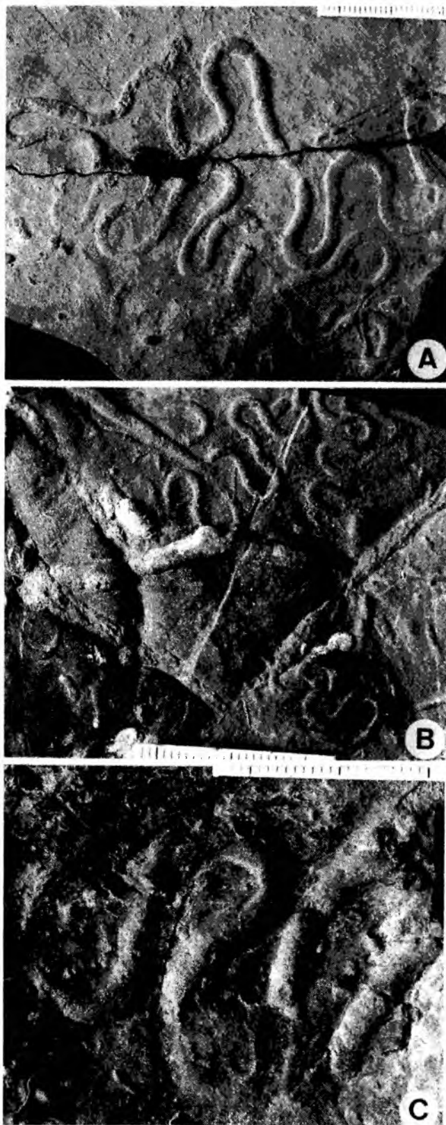
Fig. 75. Cosmorhaphes lobata Seilacher on soles of turbiditic sandstone beds (labelled as Cosmorhaphes sinuosa ). A. UJ TF 74, Variegated Shale (Paleocene–Eocene), Lipnica Wielka. B. UJ TF 75, Inoceranian beds (Senonian–Paleocene), Szczepanowice. C. (?) UJ TF 754, full relief, Pólrzeczeki (part of label lost). Scales in mm
