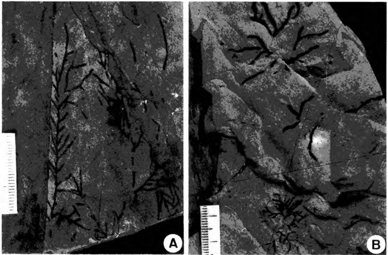
Fig. 21. Chondrites targionii (Brongniart). A. UJ TF 619, Inoceranian beds (Senonian–Paleocene), Lubomierz. Parallel laminated (Tb) turbiditic sandstone bed. B. UJ TF 1007, Siliceous marls (Turonian), Huwniki. Turbiditic marlstone bed (labelled as Chondrites flexilis ). Scale in mm
