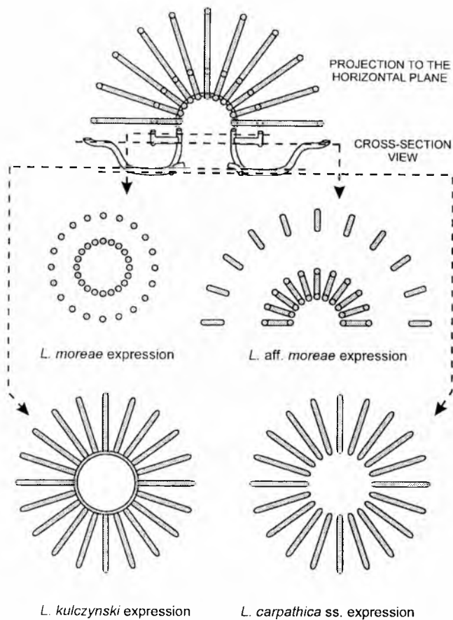
Fig. 32. Model of burrow system integrating Lorenzina carpathica , L. moreae , L. peralta , L. kulczynskii , and L. curticostata as morphological variants related to depth of erosion
