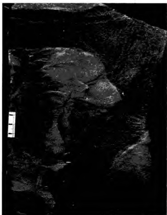
Fig. 54. Phycosiphon hamata (Fischer-Ooster), endichnial form in turbiditic sandstone bed, epichnial position. UJ TF 738, Ropianka beds (Senonian-Paleocene), Szczawa. Scale in mm
