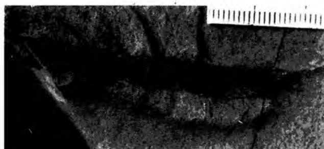
Fig. 16. Planolites heverleyensis Billings. Endichnial form in marlstone bed. UJ TF 999. Siliceous marls (Turonian), Huwniki (part of label lost). Scale in mm
