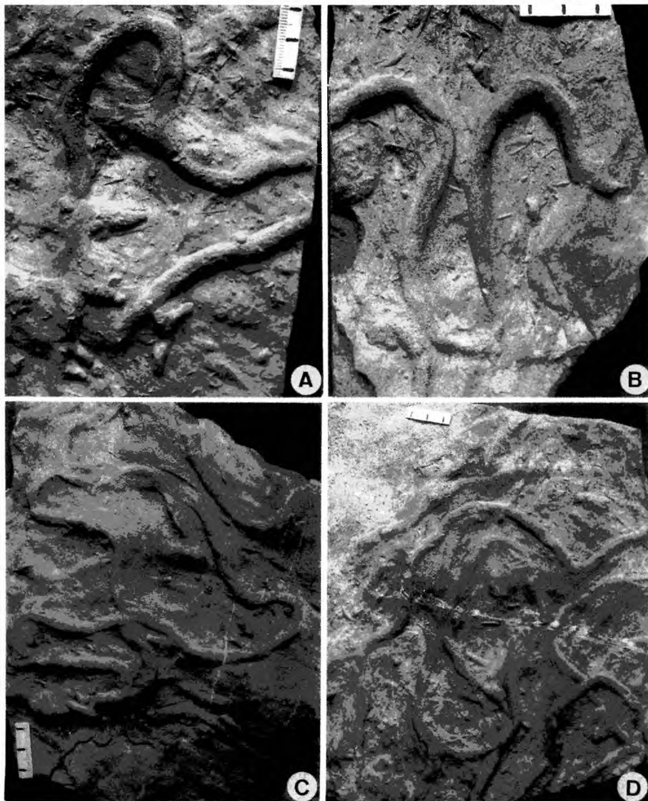
Fig. 84. " Helminthopsis granulata " Książkiewicz on soles of turbiditic sandstone beds. A. UJ TF 1373 (label lost). B. UJ TF 2578a, Cieszyn Limestone (Beriassian), Golezów quarry (labelled Helminthopsis aff. hieroglyphica ). C. UJ TF 1374 (label lost). D. UJ TF 2574 (label lost). Scales in mm
