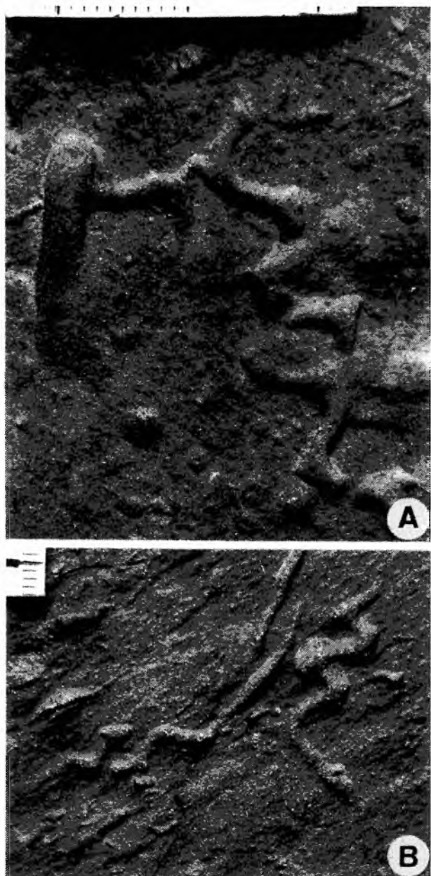
Fig. 91. Belorhaphé zickzack (Heer) on soles of turbiditic sandstone beds. A. UJ TF 1666, Beloveža beds (Eocene), Sidzina. B. UJ TF 2445, Jaworki (part of label lost). Scales in mm
