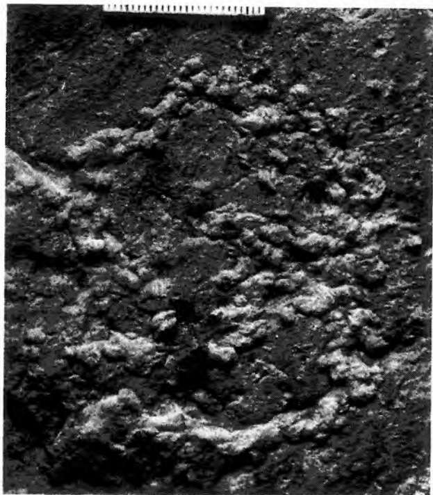
Fig. 109. Form C. Sole of a turbiditic sandstone bed. UJ TF 2029, Ciężkowice Sandstone (Eocene), Gródek (part of label lost). Scale in mm
