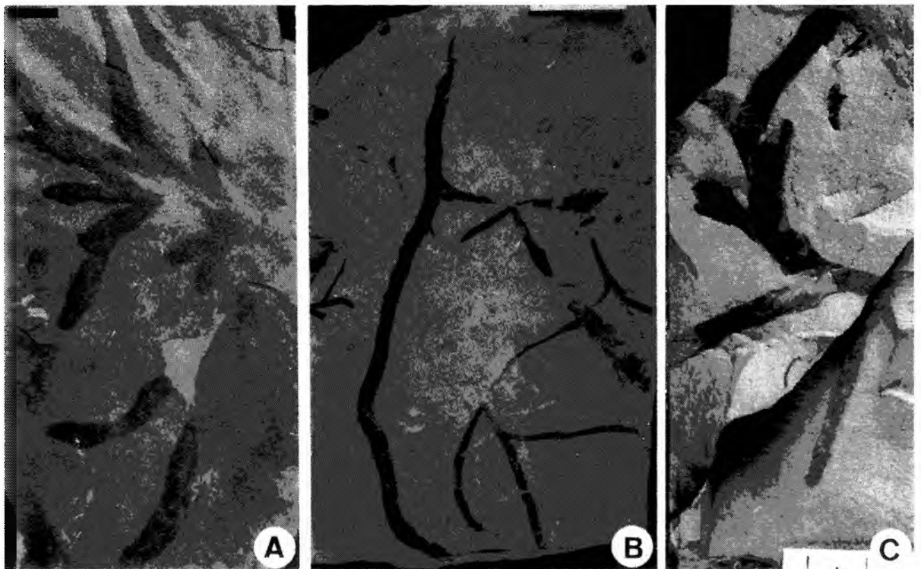
Fig. 22. A–B. Chondrites targionii (Brongniart), large forms. A. UJ TF 707, Variegated Shale (Paleocene–Lower Eocene), Szczawa. Turbiditic sandstone bed (labelled as Chondrites affinis ). B. UJ TF 1003, Siliceous marls (Turonian), Huwniki. Turbiditic marlstone bed (labelled as Chondrites affinis ). C. Chondrites recurvus (Brongniart), UJ TF 994. Siliceous marls (Turonian), Huwniki. Turbiditic marlstone bed. Scale bar in A = 1 cm, scales in B–C in cm
