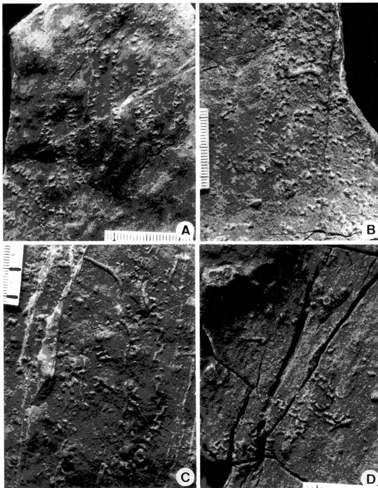
Fig. 93. Paleomeandron elegans Peruzzi on soles of turbiditic sandstone beds. A. UJ TF 221, Szczawa (part of label lost). B. UJ TF 1423, Osielec (part of label lost). C. UJ TF 219, Sidzina-Glaza stream (part of label lost, labelled as Paleomeandron intermedium ). D. UJ TF 1176, Wierzbanowa (part of label lost). Scales in mm
