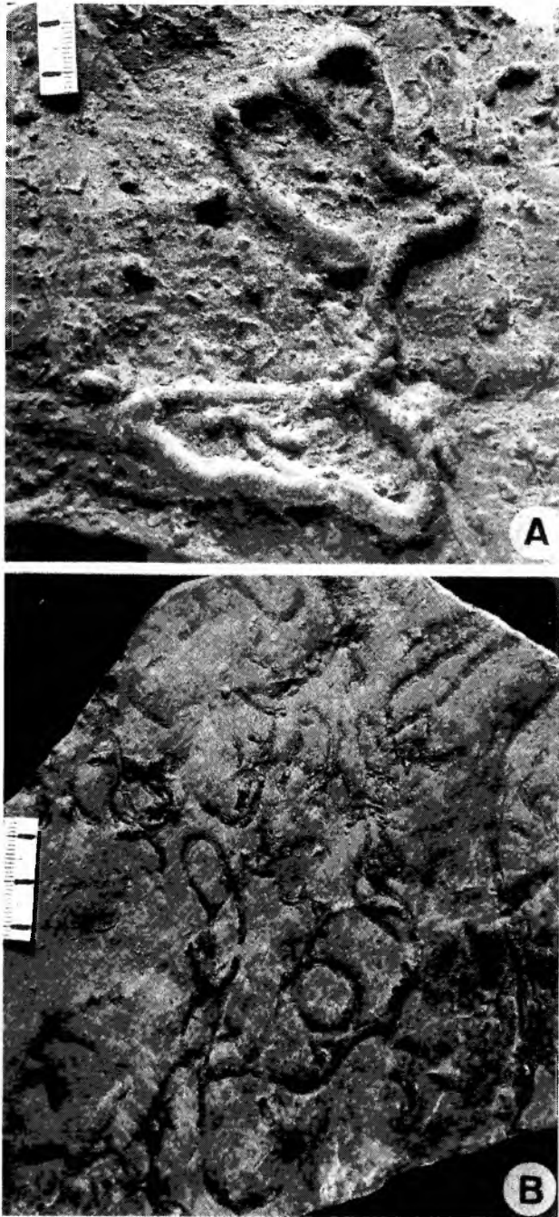
Fig. 73. Gordia marina Emmons. UJ TF 1082, sole of turbiditic sandstone bed, Sidzina, Beloveža beds (Eocene), Sidzina (labelled as Helminthopsis hieroglyphica ). B. UJ TF 1353, Krościenko (label lost). Scale in mm
