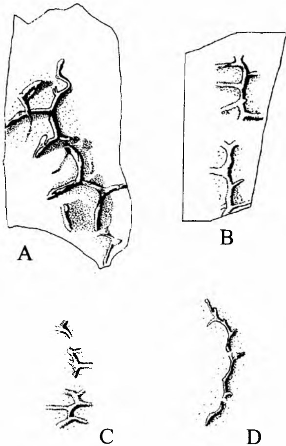
Fig. 102. Protospaleodictyon spinata (Geinitz). A. Redrawn from Geinitz (1867), pl. 6, fig. 4 (labelled as Palaeophycus spinatus ). Tentaculitenschiefer, Zederhügel near Schleiz, Germany. B. Redrawn from Richer (1927), pl. 1, fig. 5 (labelled as "Trugdoldig verzweigte Fährte"). Upper Devonian quartzit, Saalfeld, Thuringia, Germany. C. Redrawn from Pfeiffer (1968), pl. 6, fig. 4 (labelled as Spinorhapha spinata ), neotype, Kulm (Lower Carboniferous), Koselstein, Germany. D. Redrawn from Pfeiffer (1968), pl. 6, fig. 6 (labelled as Spinorhapha rubra ), Kulm (Lower Carboniferous), Koselstein, Germany
