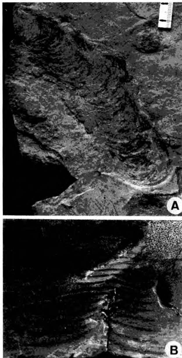
Fig. 51. Zoophycos spp. A. Zoophycos insignis Squinabol, endichnial form in turbiditic sandstone bed. UJ TF 2572, Ropianka beds (Senonian–Paleocene, Wola Brzezińska. B. Zoophycos isp. ( Spirophyton -type), endichnial form in cross-section of turbiditic mudstone bed. UJ TF 13, Magura beds (Eocene), Zabrzeż. Scale in A in mm, scale bar in B = 1 cm
