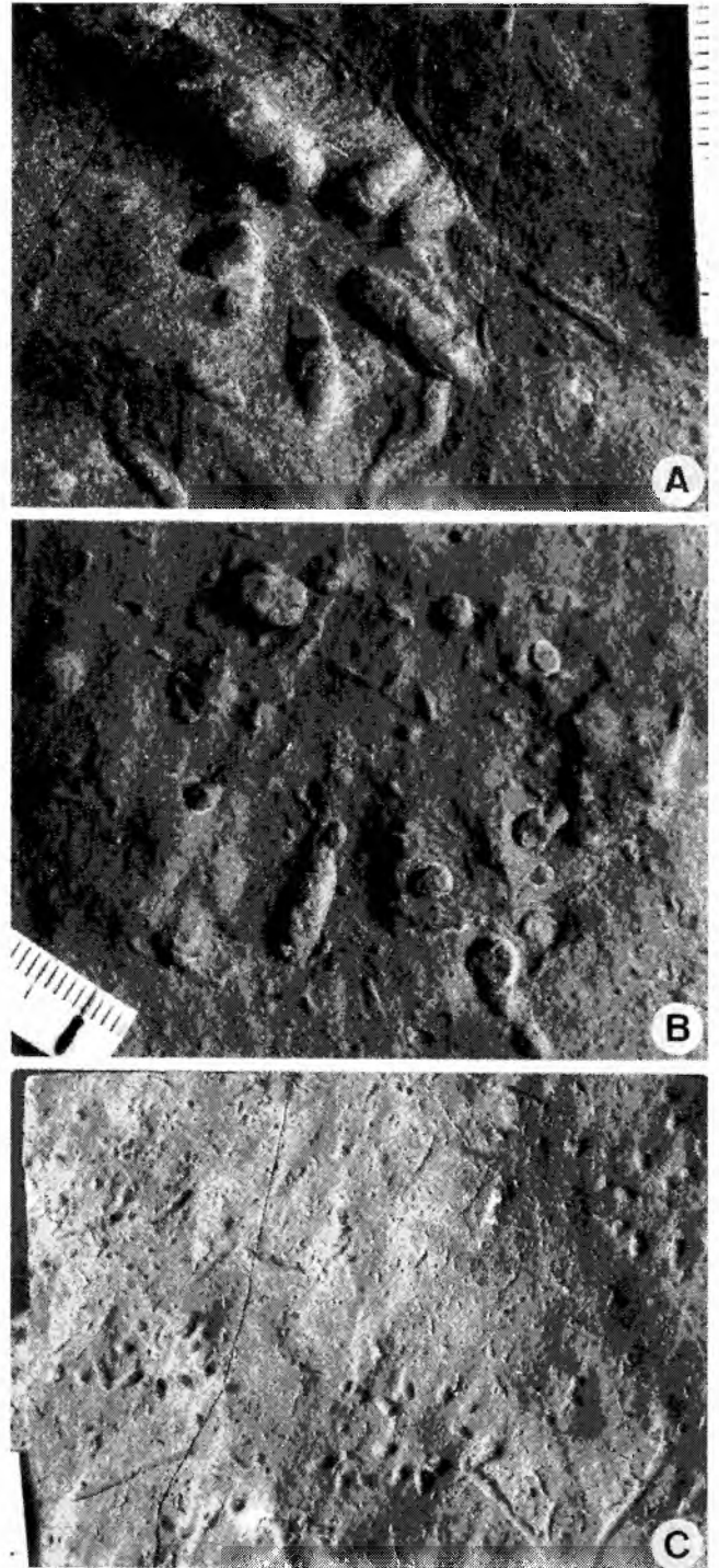
Fig. 37. Lorenzium plana (Książkiewicz), soles of turbiditic sandstone beds. A. UJ TF 137, Middle Godula beds (Turonian), Ponikiew. B. UJ TF 198, Beloveža Formation (Eocene), Sidzina (labelled as Sublorenzium aff. pustulosa ). C. UJ TF 98, Cieszyn Limestone (Beriasian), Goleszów. Scale in mm
