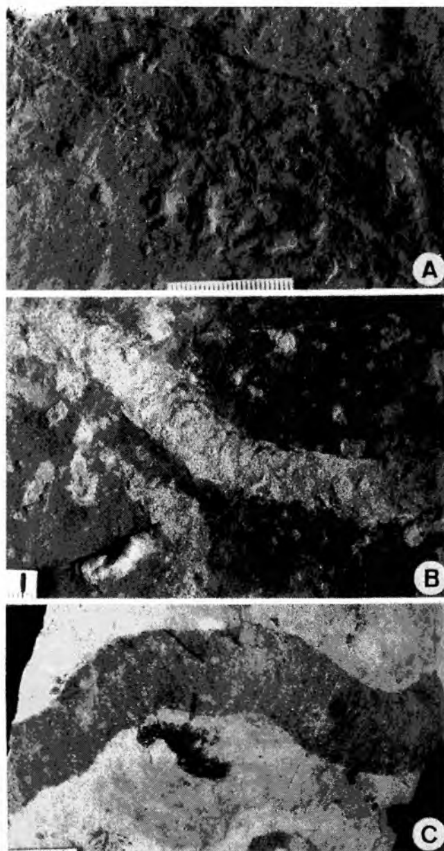
Fig. 66. Taenidium ispp. A. UJ TF 833, hypichnial form in mudstone. Ropianka beds (Senonian-Palaeocene), Limanowa-Marciszówka (labelled as Keckia aff. hoessii ). B. UJ TF 1002, endichnial form in a marlstone bed. Siliceous marls (Turonian), Huhniki (labelled as Muensteria geniculata ). C. ? Taenidium ispp., endichnial form in a marlstone bed. UJ TF 1004. Siliceous marls (Turonian), Huhniki (labelled as Muensteria geniculata ). Scales in mm
