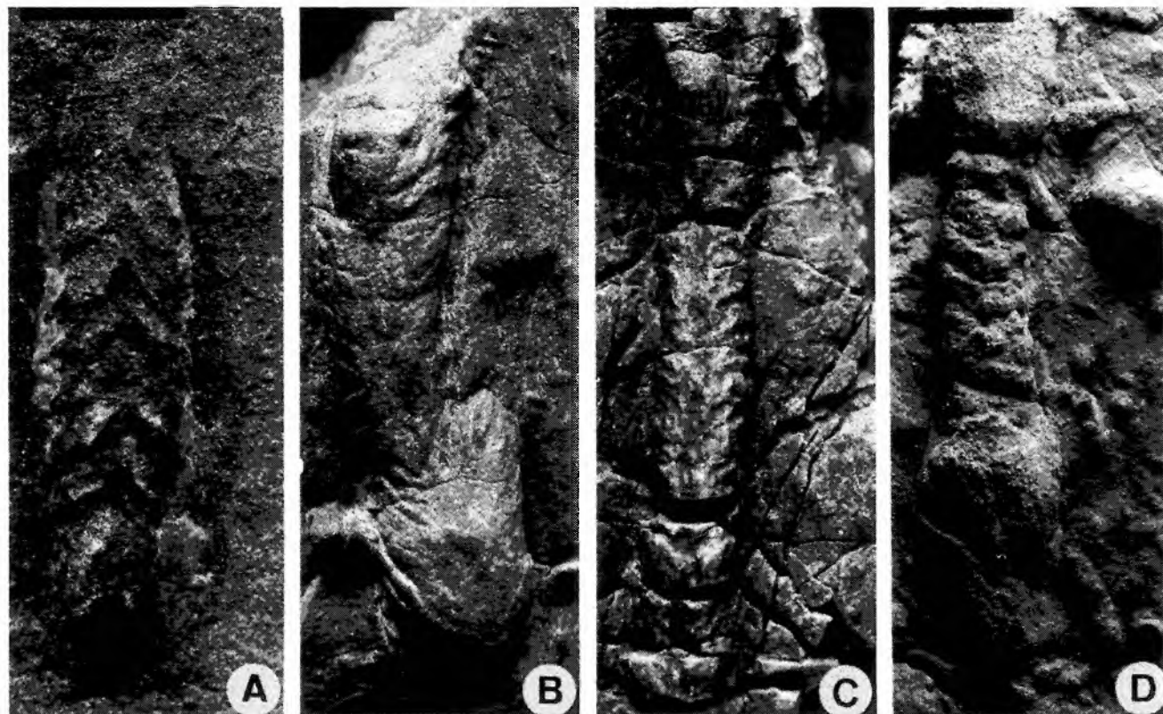
Fig. 68. Protovirgularia ispp. Soles of turbiditic sandstone beds. A. Protovirgularia ?longespicata (De Stefani). UJ TF 679, Grodziszcze beds (Hauterivian), Lipnik (labelled as Gyrochorte burtani ). B. P. rugosa Miller & Dyer. UJ TF 936, Inoceramian beds (Senonian–Paleocene), Wierzbanowa (labelled as Gyrochorte burtani ). C. P. obliterated (Książkiewicz) UJ TF 1169, Verovice beds (Barremian–Aptian), Wiśniowa (labelled as Gyrochorte burtani ). D. P. rugosa . UJ TF 178, Sromowce Formation (Senonian), Szaflary (labelled as Rhabdoglyphus bisculdatus ). Scale bars = 1 cm
