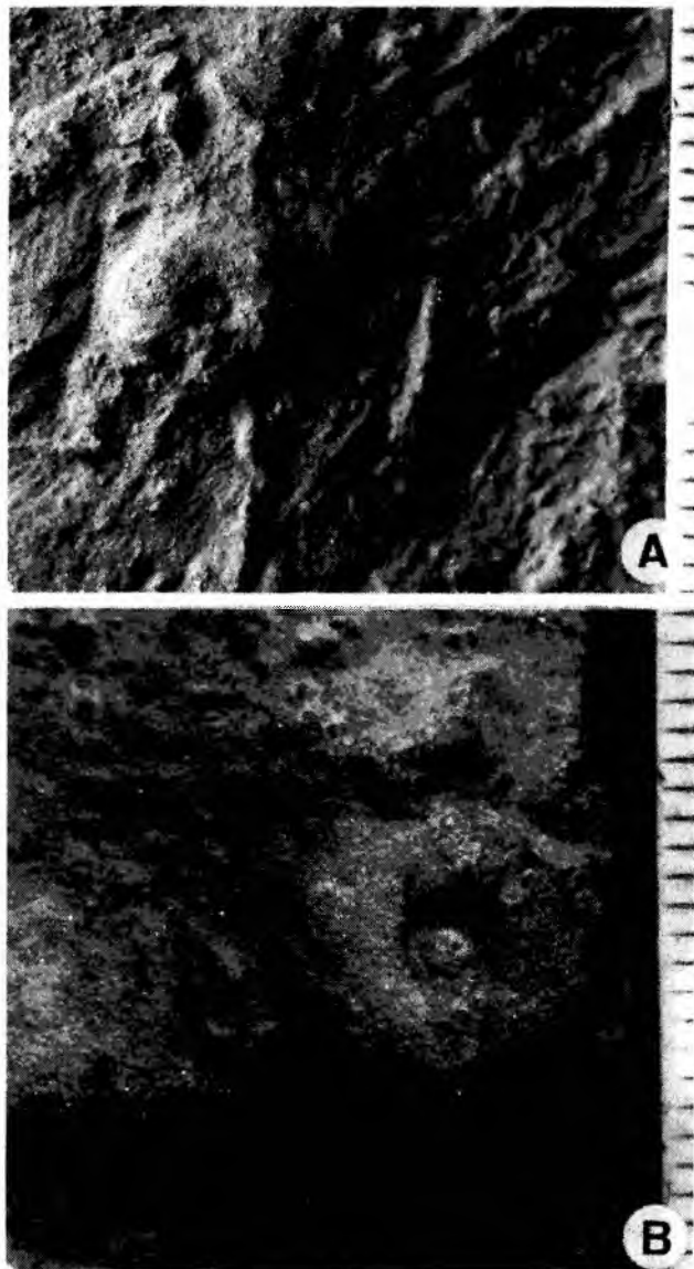
Fig. 1. Mammillichnis aggeris Chamberlain, soles of turbiditic sandstone beds. A. UJ TF 1649, Krosno beds (Oligocene), Stonne Góry range near Załuż. B. UJ TF 2501, Krosno beds (Oligocene), Wujskie. Scales in mm
