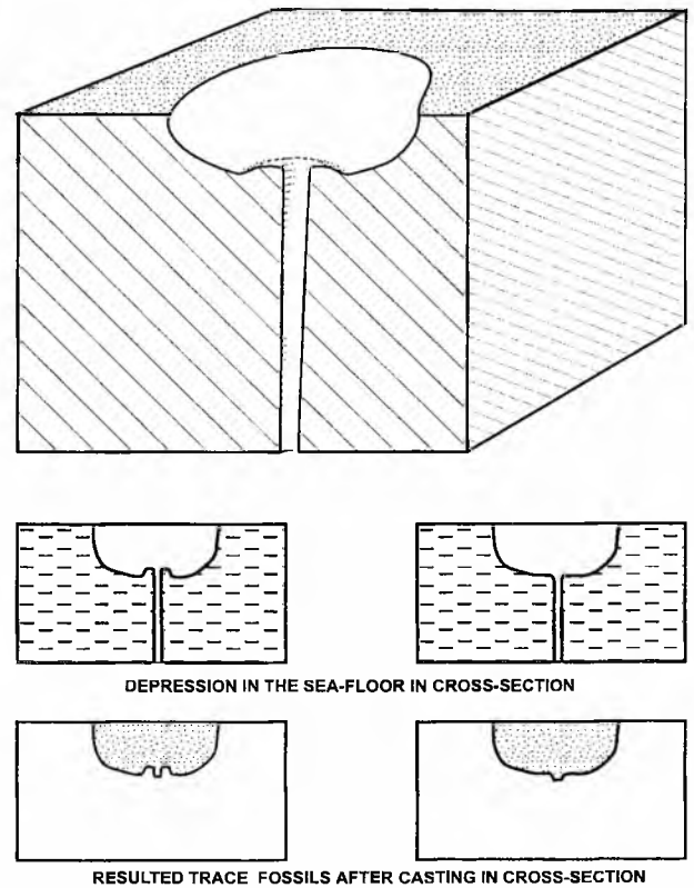
Fig. 2. General model (top) and morphological variations (below) of Mammillichnis . The morphological variants depend on the shape of the depression in the sea floor
