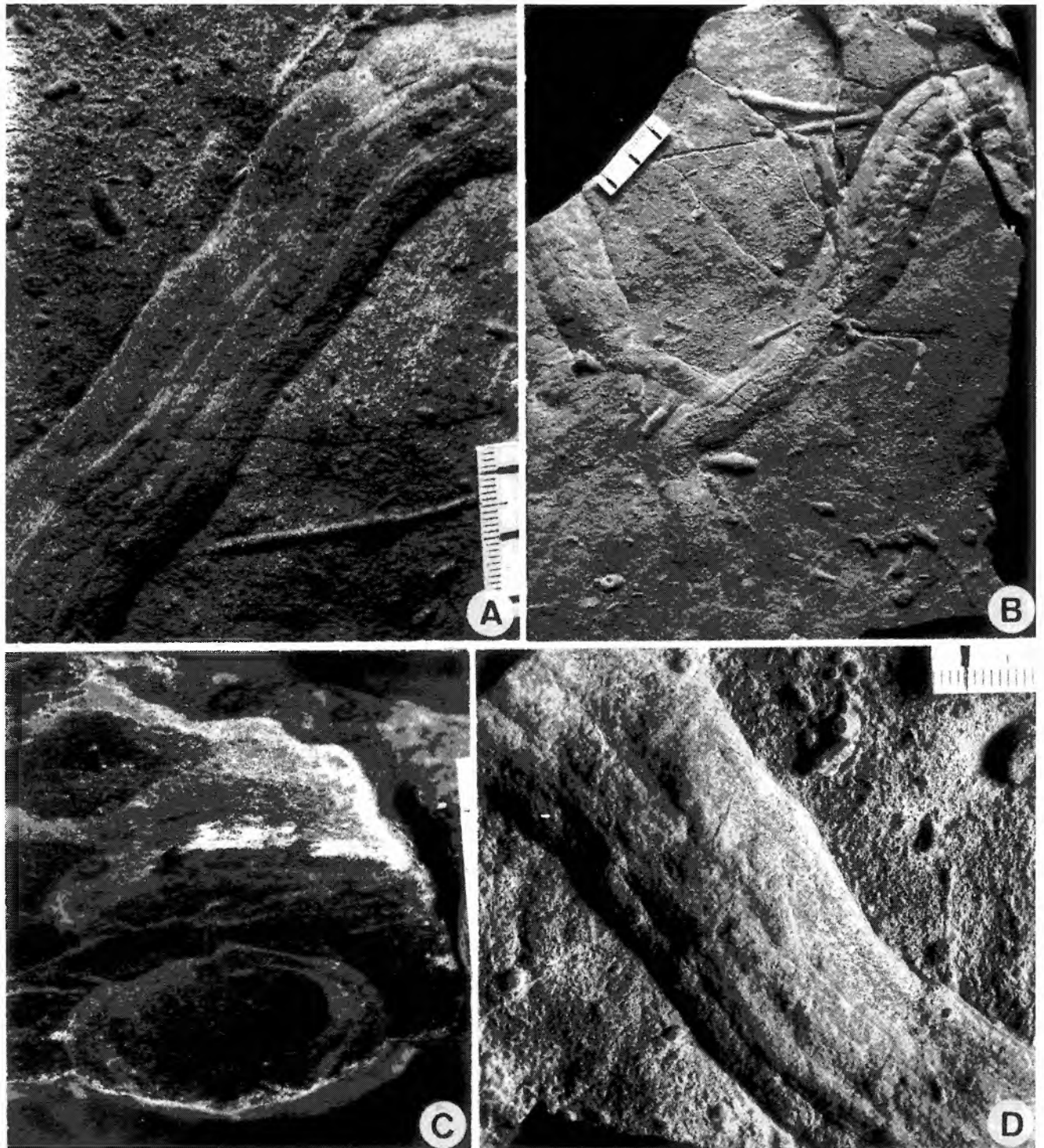
Fig. 60. Scolicia plana Książkiewicz in turbidite sandstone beds. A-C. Hypichnial views of ventral exterior. A. UJ TF 2545, Variegated Shale (Paleocene–Eocene), Kałowa. B. UJ TF 1542, Beloveža Formation (Eocene), Lipnica Wielka (labelled as Subphyllochorda granulata ). C-D. UJ TF 2543, Variegated Shale (Paleocene–Eocene), Kałowa. C. Cross-section view. D. Hypichnial view. Scales in mm
