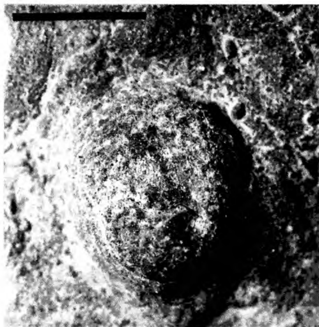
Fig. 3. ? Bergaueria prantli Książkiewicz, sole of turbiditic sandstone bed. UJ TF 907, Ropianka beds (Senonian–Paleocene), Kałowa. Scale bar = 1 cm
