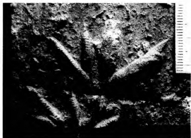
Fig. 6. Arthropycus strictus Książkiewicz. Sole of a turbiditic sandstone bed. UJ TF 124, Ropianka beds (Senonian–Paleocene), Mszana Dolna. Scale in mm
