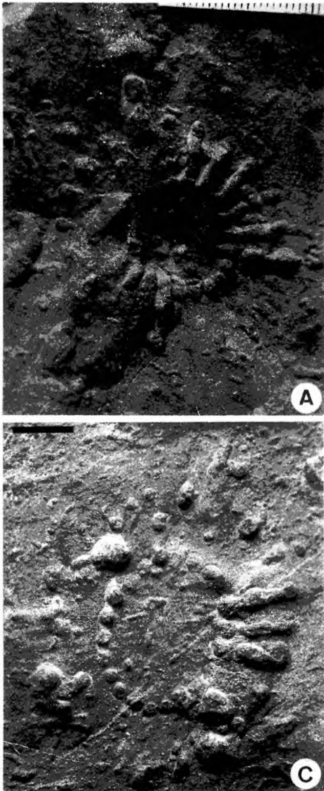
Fig. 35. Lorenzina carpathica (Zuber), different types of preservation. A. UJ TF 85, Variegated Shale (Paleocene-Eocene), Lipnica Mała (labelled as L. aff. moreae ). B. UJ TF 1109, Variegated Shale (Paleocene-Eocene), Lipnica Mała-Gubernas (labelled as L. aff. moreae ). C. UJ TF 84, Variegated Shale (Paleocene-Eocene), Lipnica Mała-Gubernas (labelled as L. peralta ). Scale in A in mm, scale bars in B-C = 1 cm
