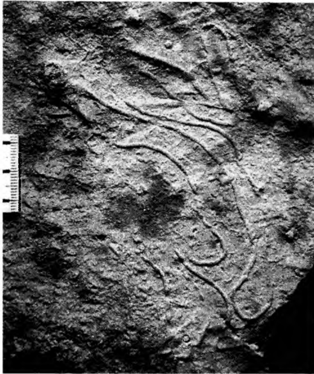
Fig. 81. Helminthorhapha japonica (Tanaka) on sole of turbiditic sandstone bed. UJ TF 104, Ciężkowice Sandstone (Eocene). Znamirowice (labelled as Helminthoidea crassa tenuis ). Scale in mm
