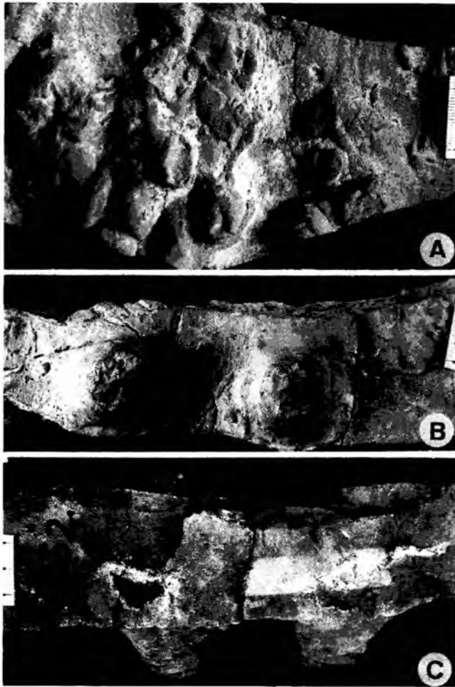
Fig. 31. Parahaentzschelinia isp. Hypichnial forms on turbiditic sandstone beds. UJ TF 855, Beloveža beds (Eocene), Berest (labelled as Tuberculichnus bulbosus ). B. UJ TF 1262, Tokarnia (part of label lost). C. Side view of B. Scale in mm
