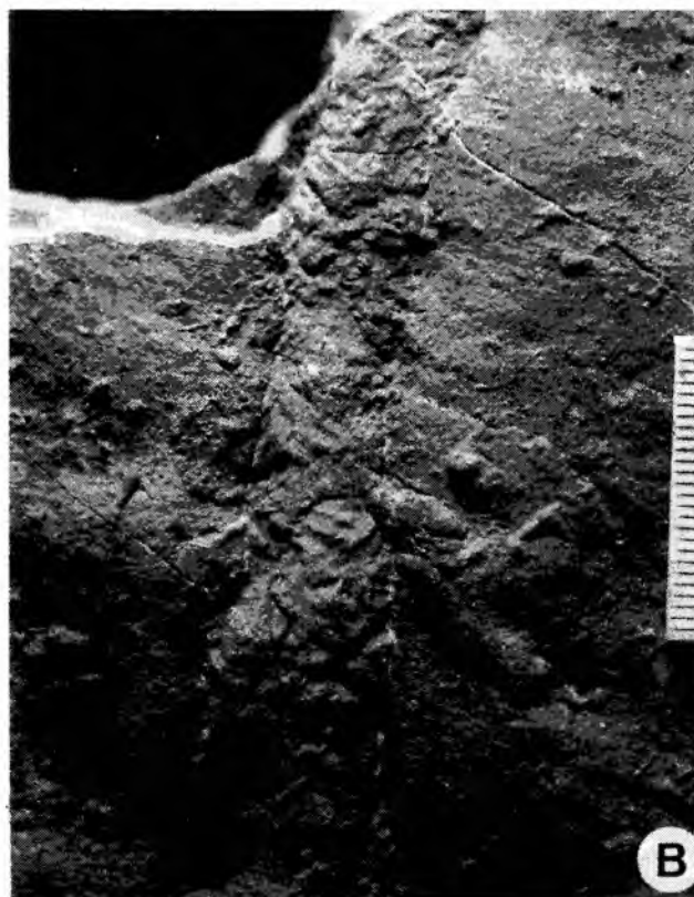
Fig. 29. Spongiomorpha sublumbrioides (Azpeitia-Moros). Sole of turbiditic sandstone bed. UJ TF 80, Beloveža Formation (Eocene), Lipnica Mala. A. General view. B. Detail of A. Scales in mm
