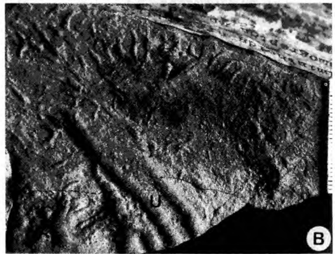
Fig. 97. Desmograpton alternum (Książkiewicz) on sole of turbiditic sandstone bed. UJ TF 816, Beloveža beds (Eocene), Berest. Scale in mm
