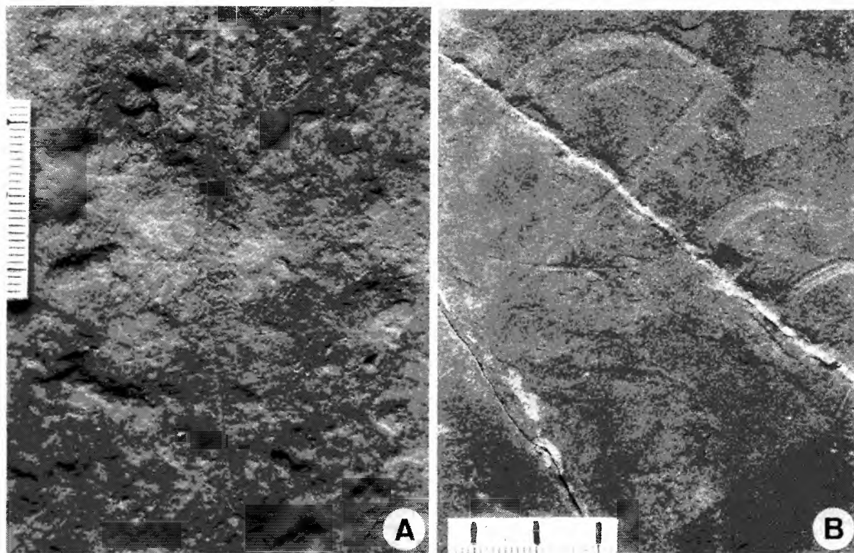
Fig. 72. Oniscoidichmus carpathicus Książkiewicz. Epichnial forms in marly siltstone beds, Krosno beds (Oligocene), Lubomierz. A. UJ TF 1741, holotype. B. UJ TF 1472a. Scales in mm
