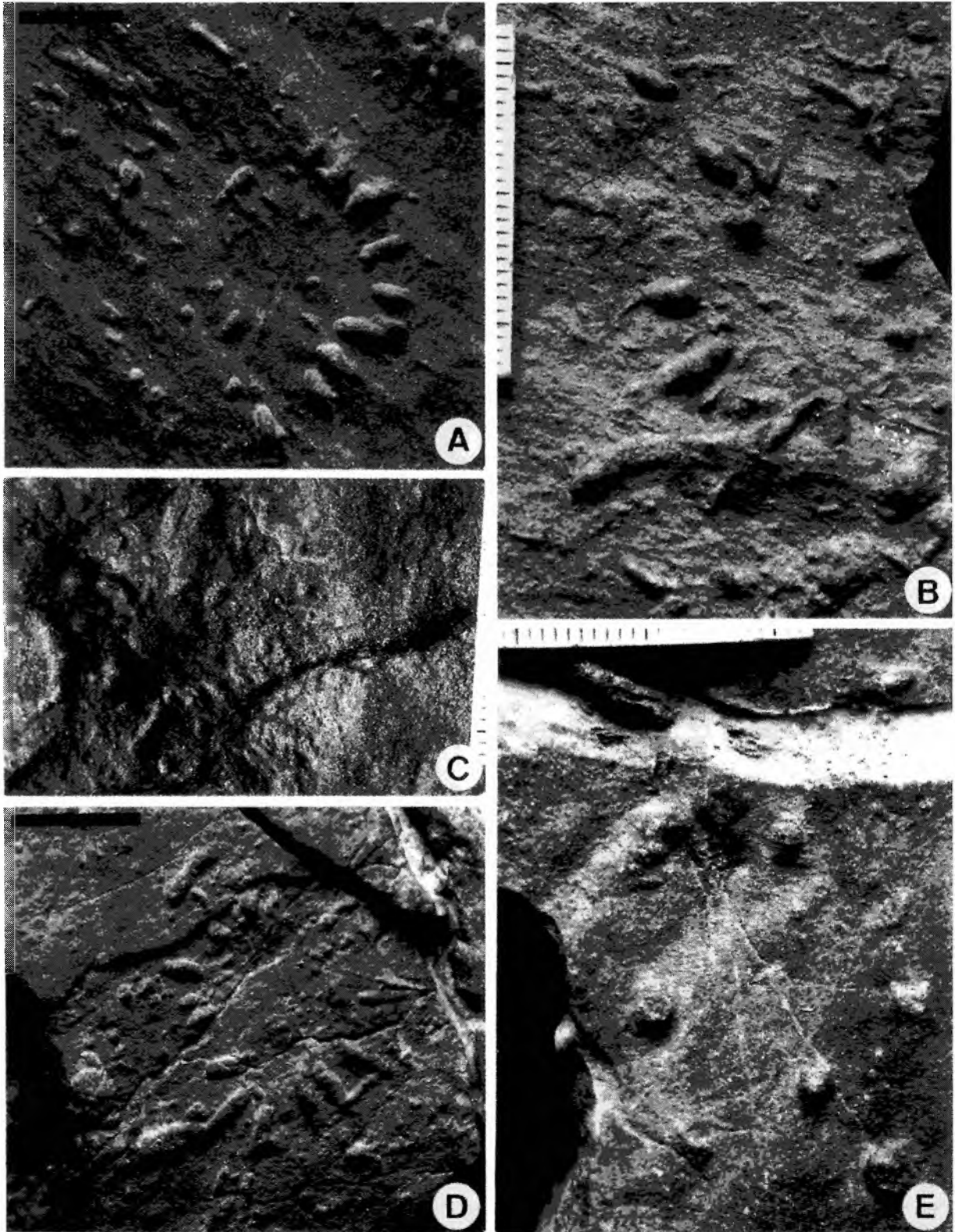
Fig. 38. Lorenzinia plana (Książkiewicz), soles of turbiditic sandstone beds. A. UJ TF 2588, Jordanów (part of label lost). B. UJ TF 971, Ropianka beds (Senonian–Paleocene), Grzechynia near Grybów (labelled as Sublorenzinia pusilla ). C. UJ TF 931, (labelled as Sublorenzinia pusilla , part of label lost). D. UJ TF 136, Hieroglyphic beds (Eocene), Grzechynia near Grybów (labelled as Sublorenzinia pusilla ). E. UJ TF 1300 (part of label lost, labelled as Sublorenzinia pusilla ). Scale bars in A, D = 1 cm, scales in B–C, E in mm
