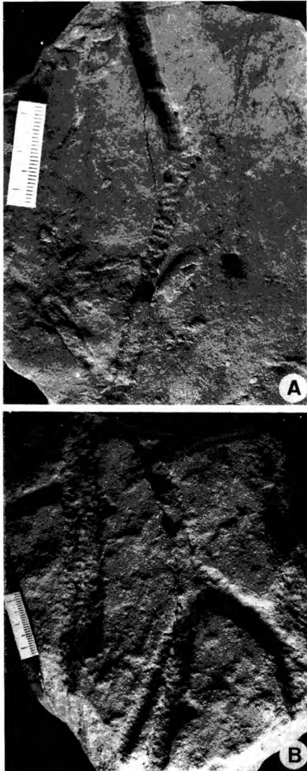
Fig. 24. Ophiomorpha annulata (Książkiewicz). Endichnial forms in turbiditic sandstone. A. UJ TF 123, Ciężkowice Sandstone (Eocene), Znamirowice. B. UJ TF 1444. Beloveža Formation (Eocene), Lipnica Mała. Scale in mm
