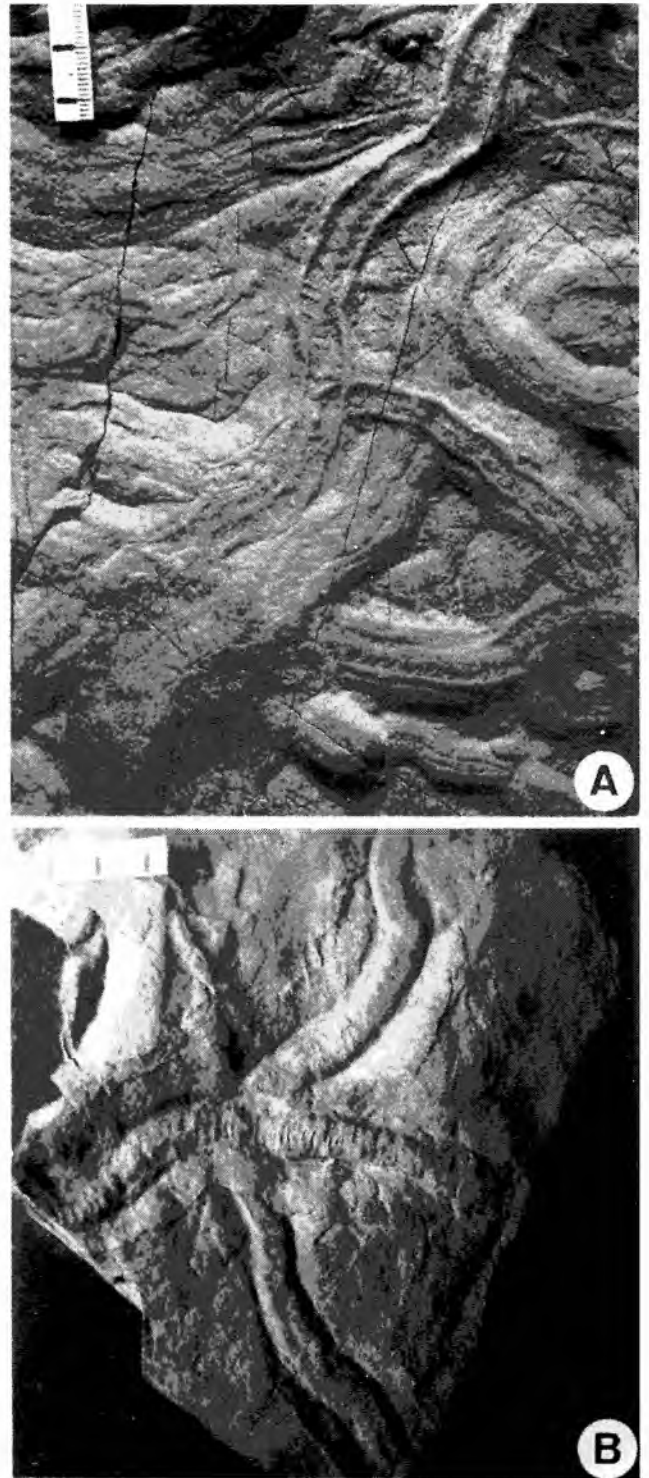
Fig. 59. Scolicia plana Książkiewicz in turbiditic sandstone beds. A. UJ TF 481, Cenomanian–Lower Senonian), Rzyki. Epichnial view of ventral interior. B. UJ TF 635, Variegated Shale (Paleocene–Eocene), Lubomierz (labelled as Subphyllochorda striata ). Hypichnial view of ventral exterior. Scales in mm
