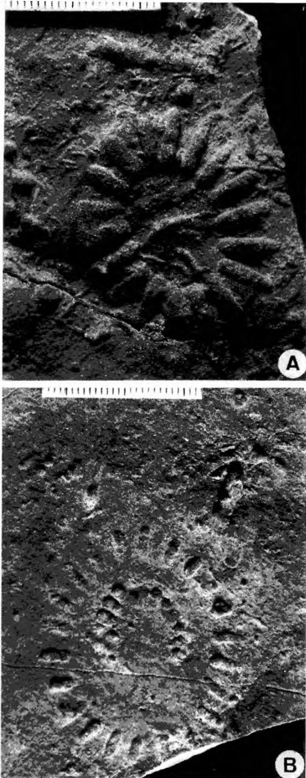
Fig. 36. Lorenzium carpathica (Zuber) on sole of turbiditic sandstone beds. A. UJ TF 871, Variegated Shale (Paleocene–Eocene), Lipnica Mała (labelled as L. carpathica ). B. UJ TF 2022, Ropianka beds (Senonian–Paleocene), Siedkierzyna (labelled as L. moreae ). Scale in mm
