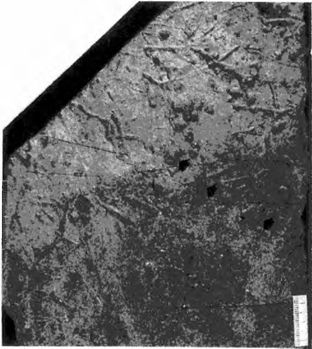
Fig. 4. Arthrophyucus strictus Książkiewicz (arrowed) and Arthrophyucus tenuis (Książkiewicz). Sole of a turbiditic sandstone bed. UJ TF 131, Lgota beds (Albian), Rzyki near Andrychów. More details are shown in Fig. 5. Scale in mm
