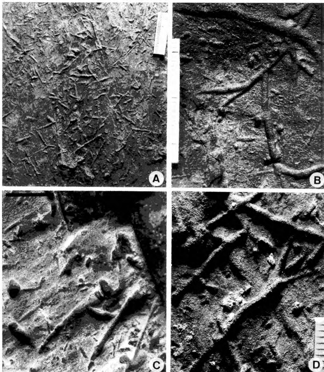
Fig. 7. Arthrophyucus tenuis (Książkiewicz). Soles of a turbiditic sandstone beds. A. UJ TF 1687, holotype, Krosno beds (Oligocene), Wujskie. B. UJ TF 2680, label lost. C. UJ TF 374, Kałowa, Ropianka beds (Senonian–Paleocene). Coll. W. Szajnocha. D. UJ TF 373, Krosno beds (Oligocene), Słonne near Załuż. Scale bars = 1 cm, scale in C in mm
