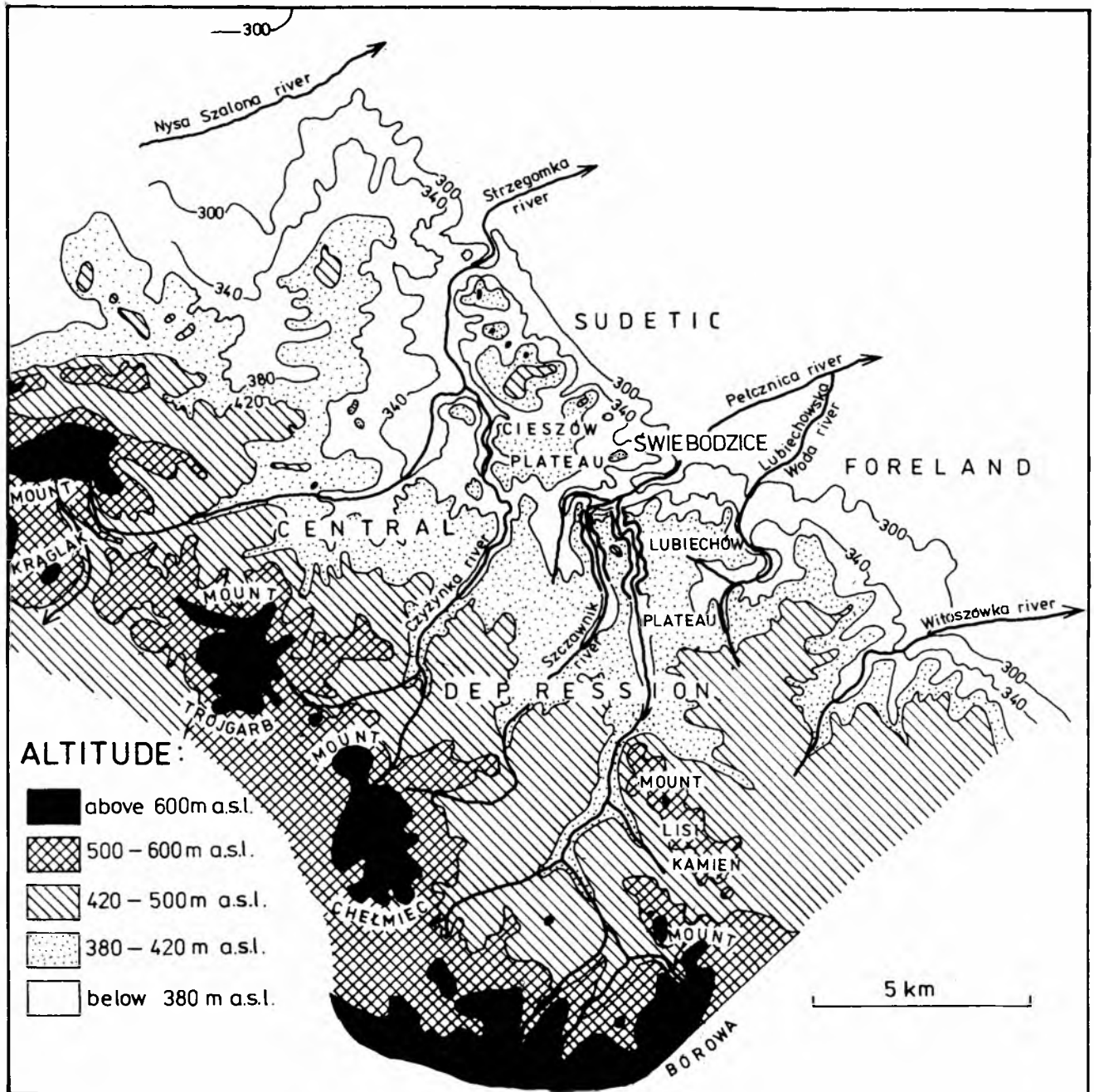
Fig. 3. Hypsometry of the Wałbrzych Upland
