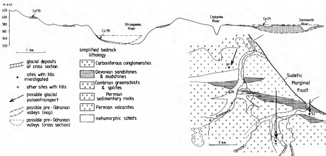
Fig. 30. Position of tills at the Walbrzych Upland (upper section) and possible glacial palaeotransport directions in relation to the bedrock (map). Bedrock geology after Teisseyre & Gawroński (1965), Teisseyre (1969) and Haydukiewicz et al. , (1982)
