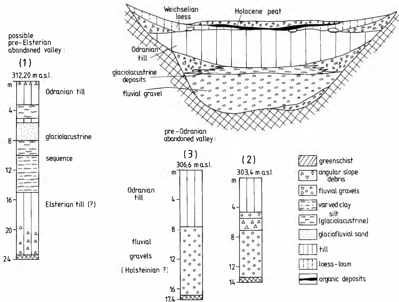
Fig. 16. Geological profiles (boring-logs) of the abandoned valleys near Dobromierz. The section in upper right is based on the data from the outcrop described by A. Jahn ( vide Stachura, 1993a) (location of borings and the outcrop is in Fig. 13)
