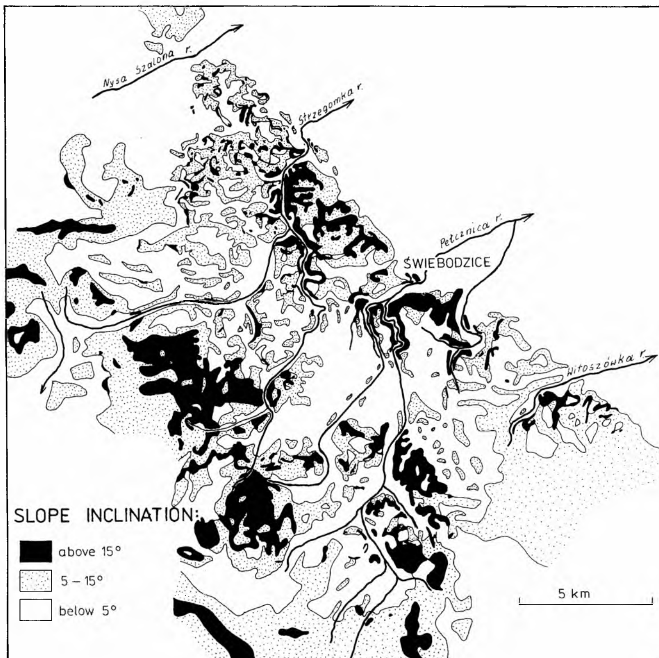
Fig. 4. Map of slope inclination. The map has been compiled on the basis of a topographic map (1:25 000) using the equation \operatorname{tg}\alpha = h d^{-1} , where \alpha – slope inclination, h – height between contour lines, d – distance between contour lines
