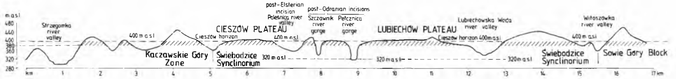
Fig. 7. Morphological cross section along the Cieszów horizon near the Sudetic Marginal Fault zone. Location of the section in Fig. 1
