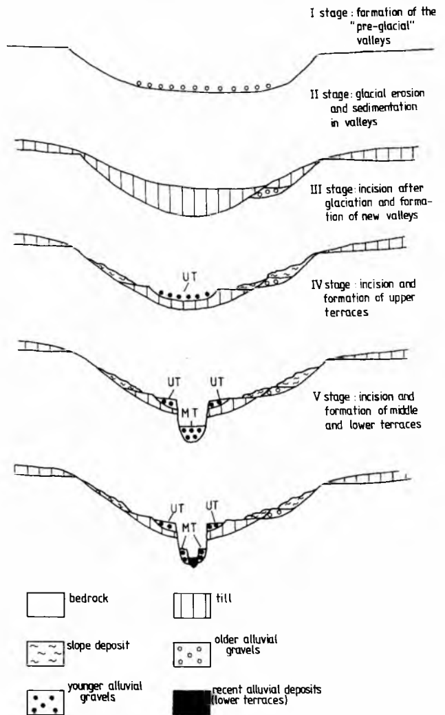
Fig. 26. Stages of the Pelcznica river valley development through Late Quaternary
