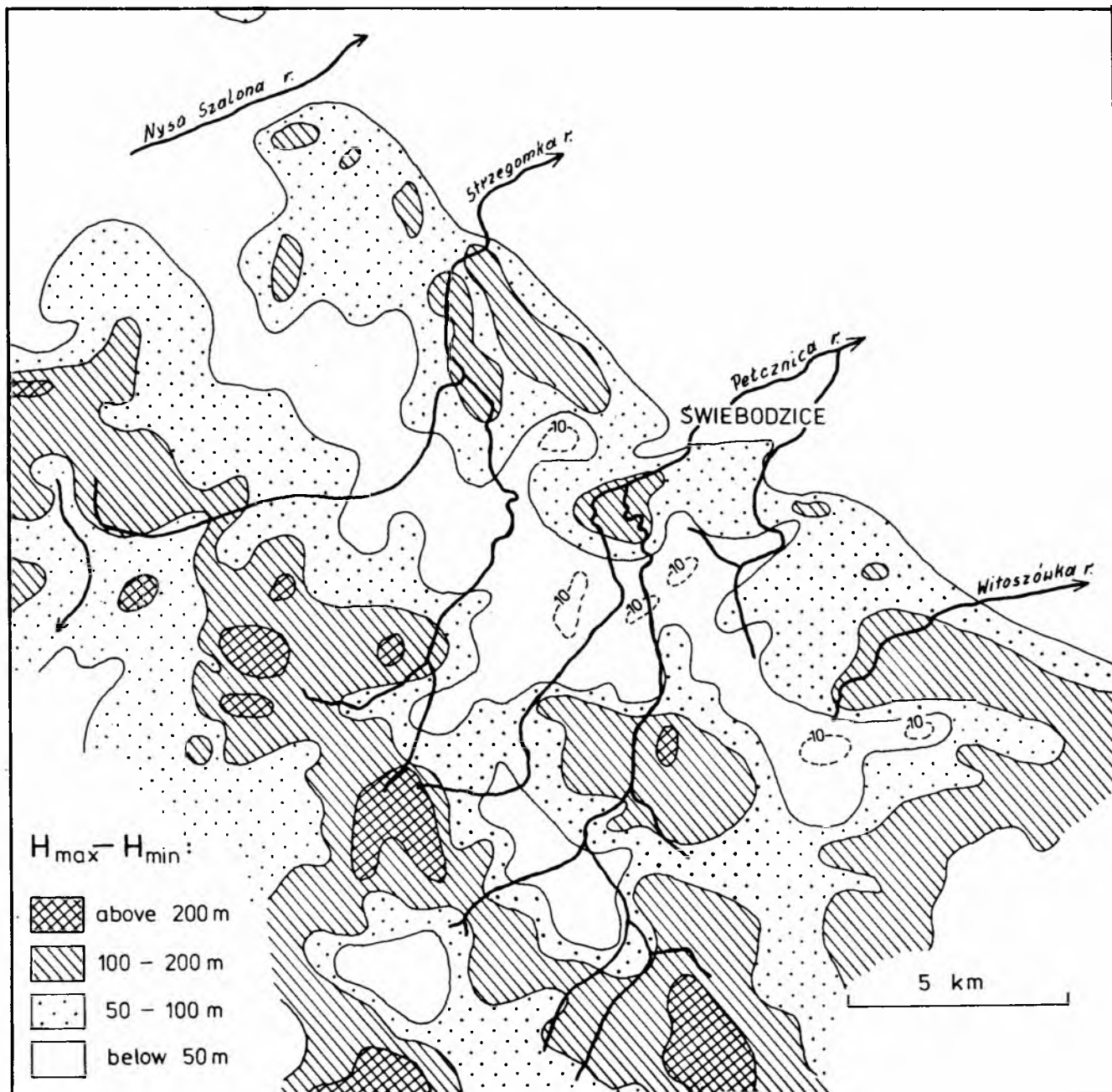
Fig. 5. Map of relief energy ( H_{max} - highest elevation in m a.s.l. H_{min} - lowest elevation in m a.s.l.). The map has been interpolated on the basis of a topographic map (1:25 000) with a net of squares (area 1 \text{ km}^2 , distance between centres 0.5 km)
