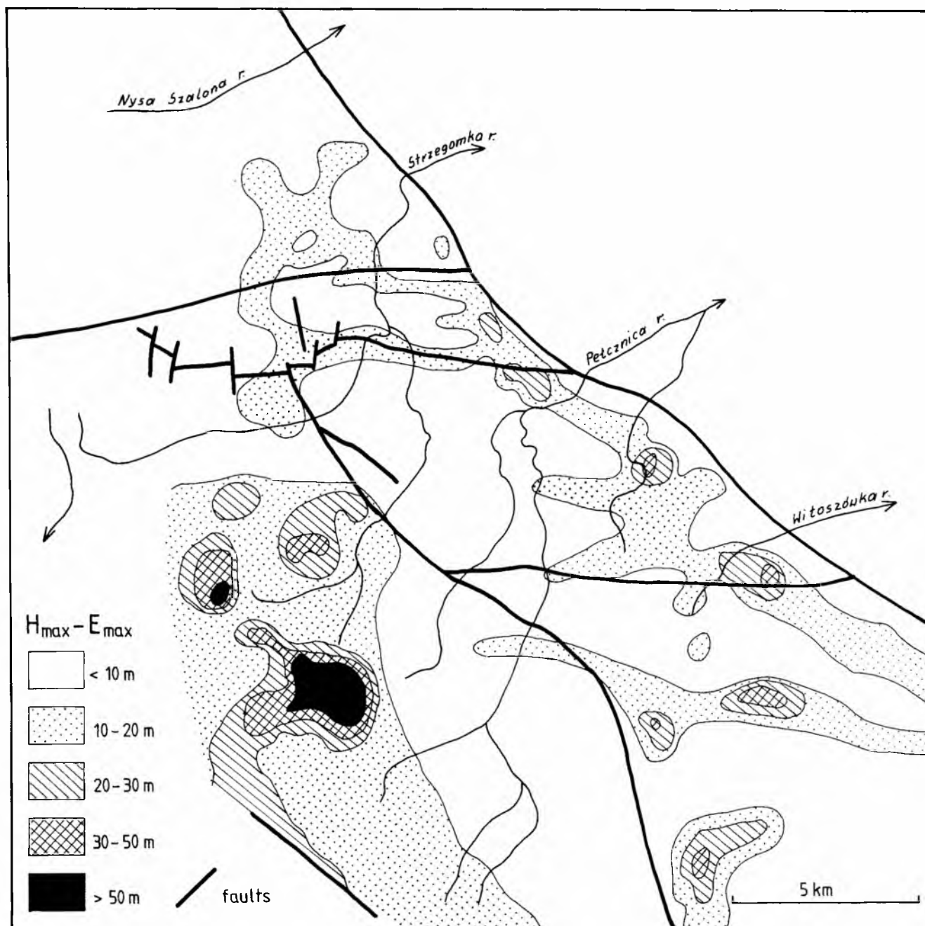
Fig. 6. Map of the relief belt above headstream erosion ( H_{\max} – highest elevation in m a.s.l., E_{\max} – highest position of erosion). The map has been interpolated on the basis of a topographic map (1:25 000) with a net of squares (area 1 \text{ km}^2 , distance between centres 0.5 km)
