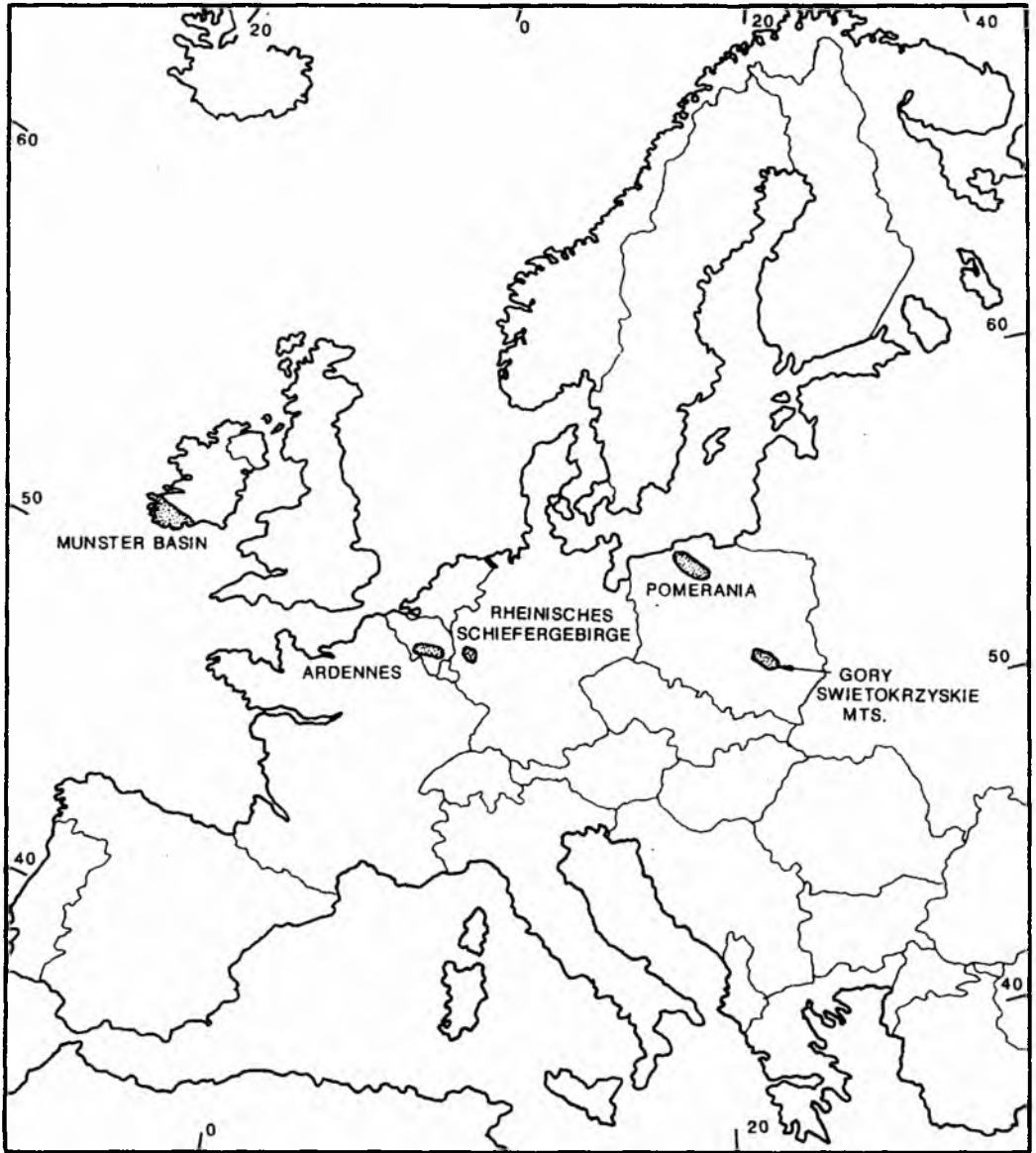
Fig. 1. Map showing position of areas discussed in text
