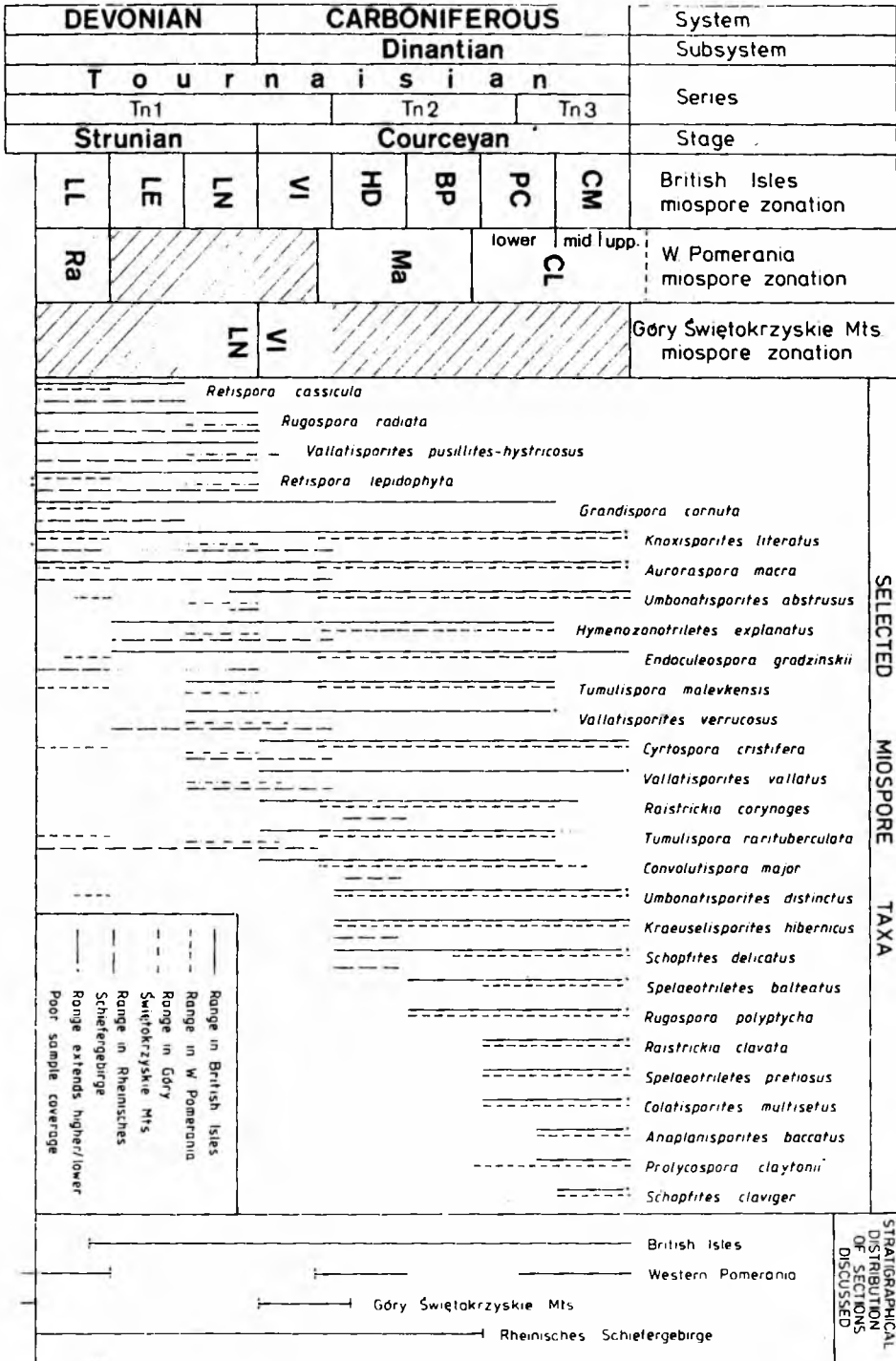
Fig. 2. Correlation of Tournaisian miospore zonation of Poland and the British Isles and stratigraphical ranges of selected spore species.
