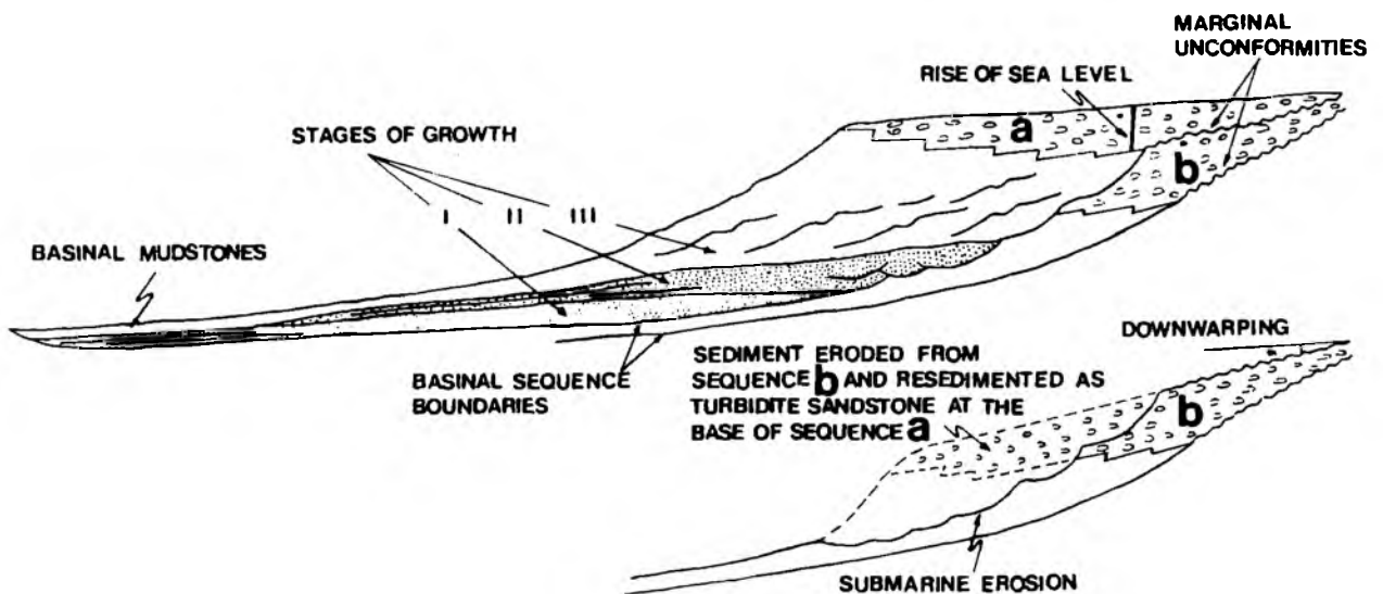
Fig. 3. Relative changes of sea level and different stages of growth of depositional sequences in elongate flysch basin (after Mutti, 1985). Earlier situation shown lower
