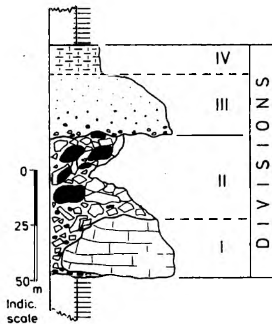
Fig. 4. Internal organization of megaturbidite. I – great blocks of platform carbonates and small fragments of limestones (white) and shales (black); II – breccia with limestone (white) and shale (black) clasts; III – graded division, changing upwards from calcirudite to calcarenite, greater fragments of limestone (white) and shale (black) at bottom; IV – marls. Beneath and above the megaturbidite is normal sequence of siliciclastic sediments
