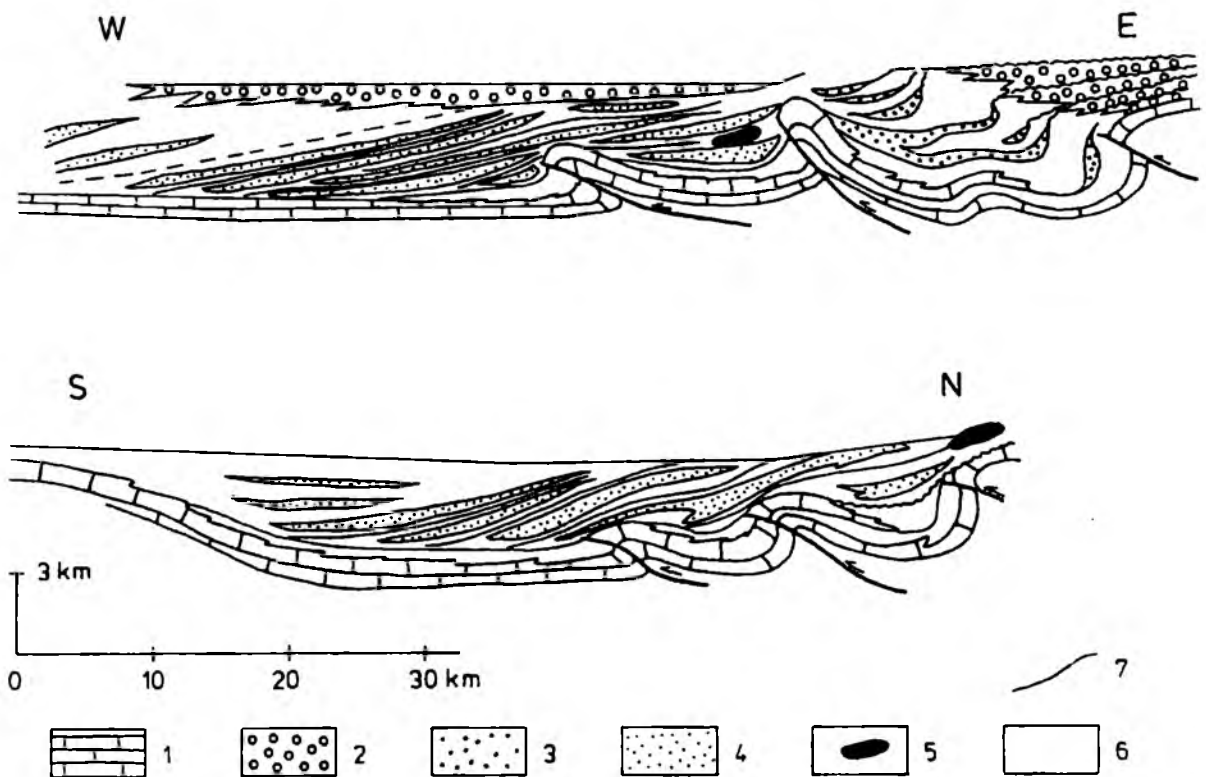
Fig. 2. Cross-sections through Ager-Jaca-Pamplona Basin. Lower section is through central part. 1 - carbonate platforms; 2 - siliciclastics platforms; 3 - channel and canyon fills; 4 - sandstone lobes; 5 - olistholites; 6 - hemipelagic and interchannel deposits; 7 - megaturbidites
