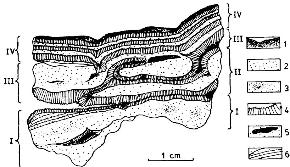
Fig. 9. Assemblage of crusts, polished section. I, II, III, IV — crust symbols; 1 — overlying deposit; 2 — cemented clastic material; 3 — loose clastic material; 4 — druzey calcite; 5 — voids within rock; 6 — laminated deposit
