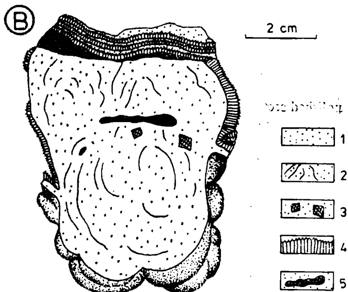
Fig. 7. Concretion B , polished section. 1 — cemented clastic material; 2 — weakly marked streaks within nonlaminated material; 3 — rock fragments; 4 — druzy calcite; 5 — pore spaces
