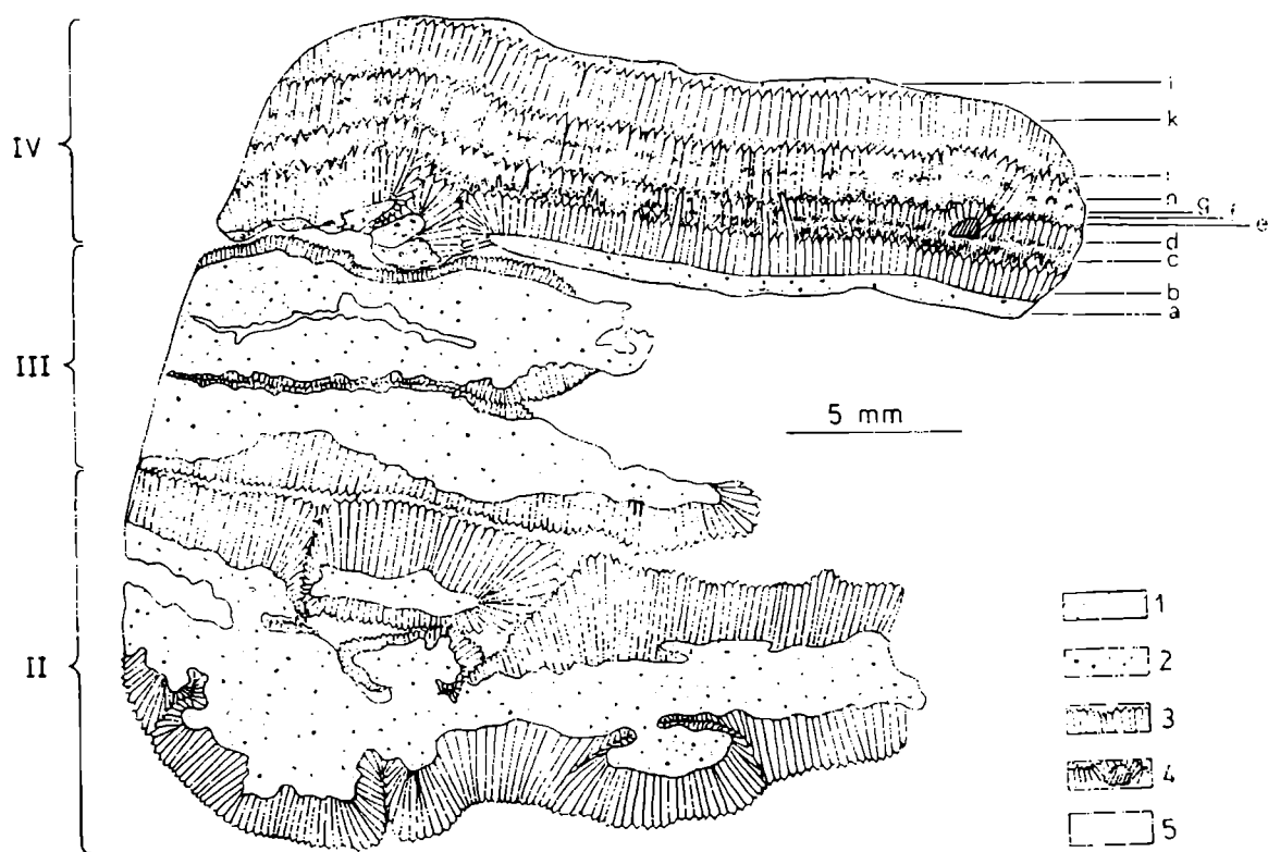
Fig. 10. Assemblage of crusts, thin section. II, III, IV — symbols of crusts; a-l — symbols of laminae; 1 — sedimentary laminae within druzi calcite of crust IV ; 2 — cemented clastic material; 3 — druzi calcite; 4 — fragment of shale overgrown with druzi calcite within sedimentary lamina; 5 — pore spaces
