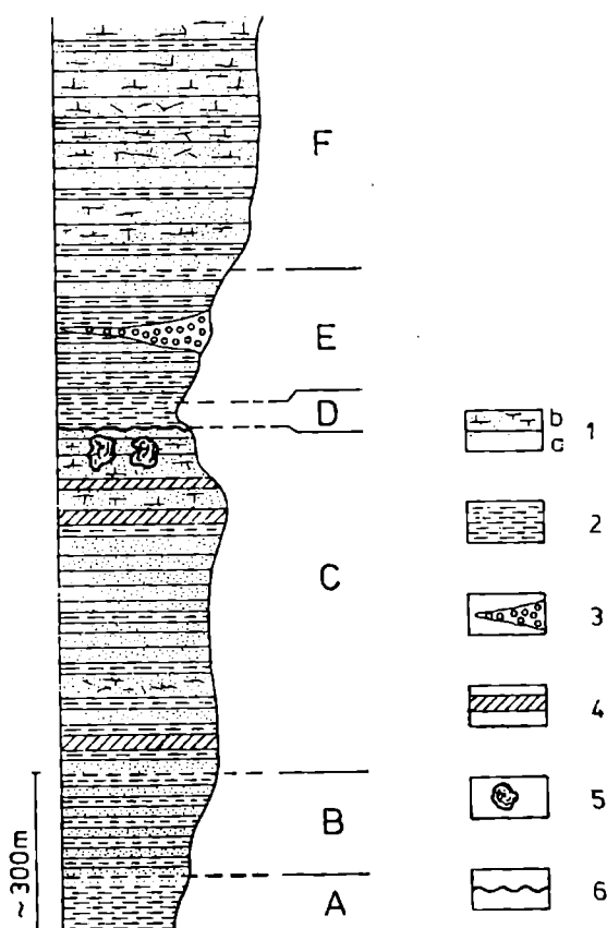
Fig. 3. Schematic lithostratigraphic section of Tylicz area. A -- variegated shales containing Glomospira (Paleocene--lower Eocene); B -- Beloveza Beds (lower Eocene); C -- Łącko Beds (undifferentiated, lower Eocene); D -- red shales containing Cyclammina amplexens (middle Eocene); E -- Hicroglyphic Beds (middle-upper Eocene); F -- Magura Beds (upper Eocene); 1 -- sandstones ( a -- solid, b -- fissured); 2 -- shales; 3 -- conglomerates; 4 -- marls; 5 -- mineral water deposits; 6 -- unconformity
