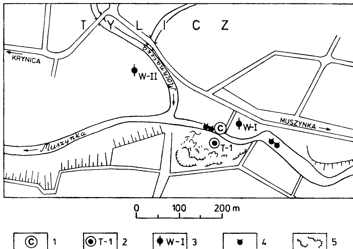
Fig. 2. Map of Tylicz showing position of trench with mineral water deposits. 1 – trench; 2 – main mineral water spring of Tylicz; 3 – wells; 4 – exhalation of free \text{CO}_2 ; 5 – slumps
