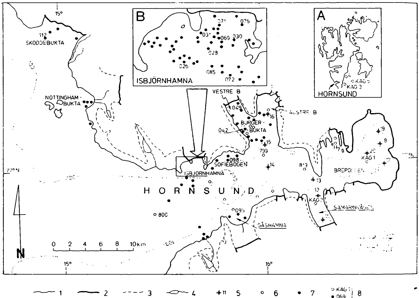
Fig. 1. Sampling sites in Hornsund and on south Spitsbergen shelf. A — Spitsbergen with sampling sites in Storffjorden (KAG 3 to KAG 5); B — Isbjörnhamna bay; 1 — shoreline; 2 — glacier margins in sea and on land; 3 — 100 m contour line; 4 — rivers and lakes; 5 — coring sites; 6 — samples recovered by J. M. Węśławski, C. Filipowicz, M. Zajączkowski and W. Moskal; 7 — samples recovered by the present author; 8 — sample numbers
