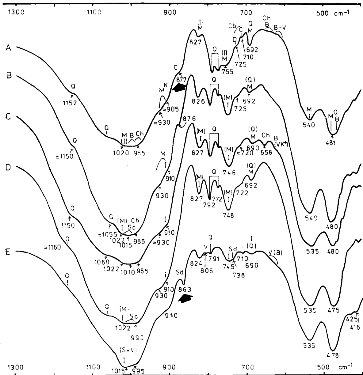
Fig. 5. Infrared spectra of variously treated and untreated fractions of sediment sample 069. A — bulk sample; B — untreated fraction < 2 \mu\text{m} ; C — \text{K}^+ saturated fraction < 2 \mu\text{m} ; D — 1n HCl treated fraction < 2 \mu\text{m} ; E — untreated fraction < 0.2 \mu\text{m} . Arrows indicate: calcite band in spectrum A and siderite band in spectrum E. Symbols for minerals as in Fig. 3
