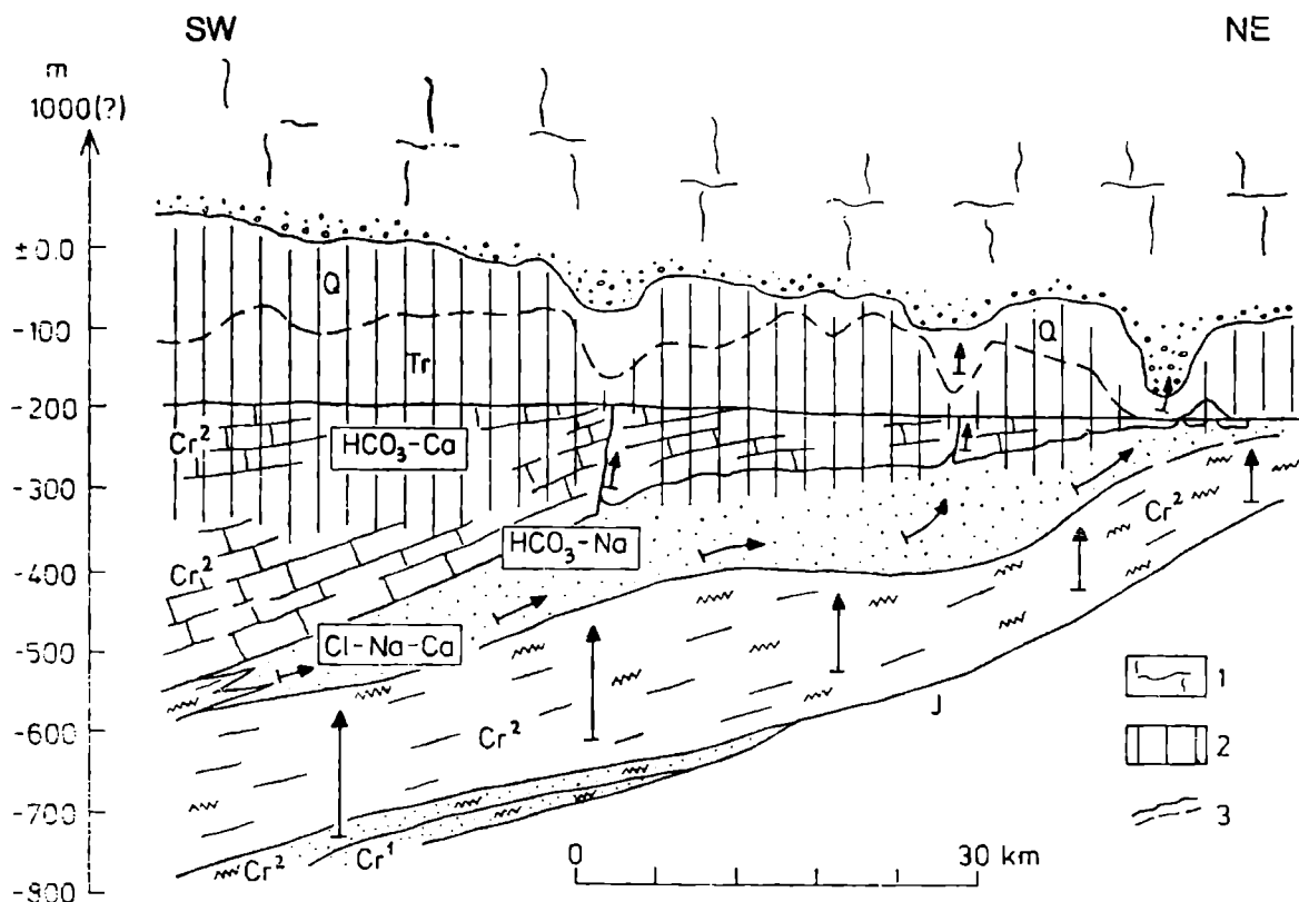
Fig. 8. Schematic cross-section of the basin during the Pleistocene glaciation (glaci-sedimentary sub-stage). 1 -- ice body, 2 -- permafrost, 3 -- lithologic and stratigraphic boundaries. Other explanations as in Fig. 4
