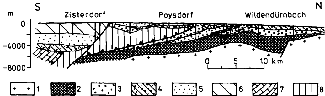
Fig. 3. Cross section through Vienna Basin (modified after Kapounek, Kröll et al. , 1965). 1 – crystalline core of Bohemian Massif, 2 – Mesozoicum, 3 – Eggenburgian–Ottngian, 4 – Karpatian, 5 – Badenian, 6 – Sarmatian, Pannonian, 7 – Northern Calcareous Alps, 8 – flysch. For other explanations – see Fig. 2
