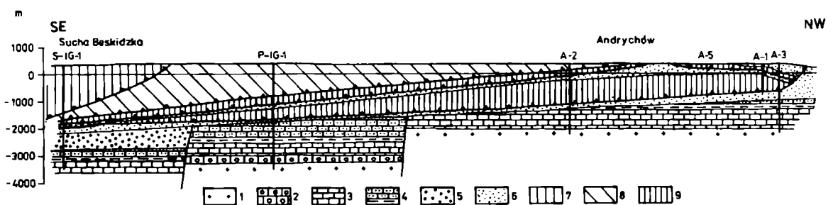
Fig. 5. Cross section through western part of Polish Flysch Carpathians. 1 – crystalline zone, 2 – old Palaeozoic, 3 – Devonian, 4 – Carboniferous, 5 – Lower Miocene (Karpatian–Ottngian), 6 – Lower Badenian, 7 – Magura Unit, 8 – Silesian Unit, 9 – Subsilesian Unit. For other explanations – see Fig. 2
