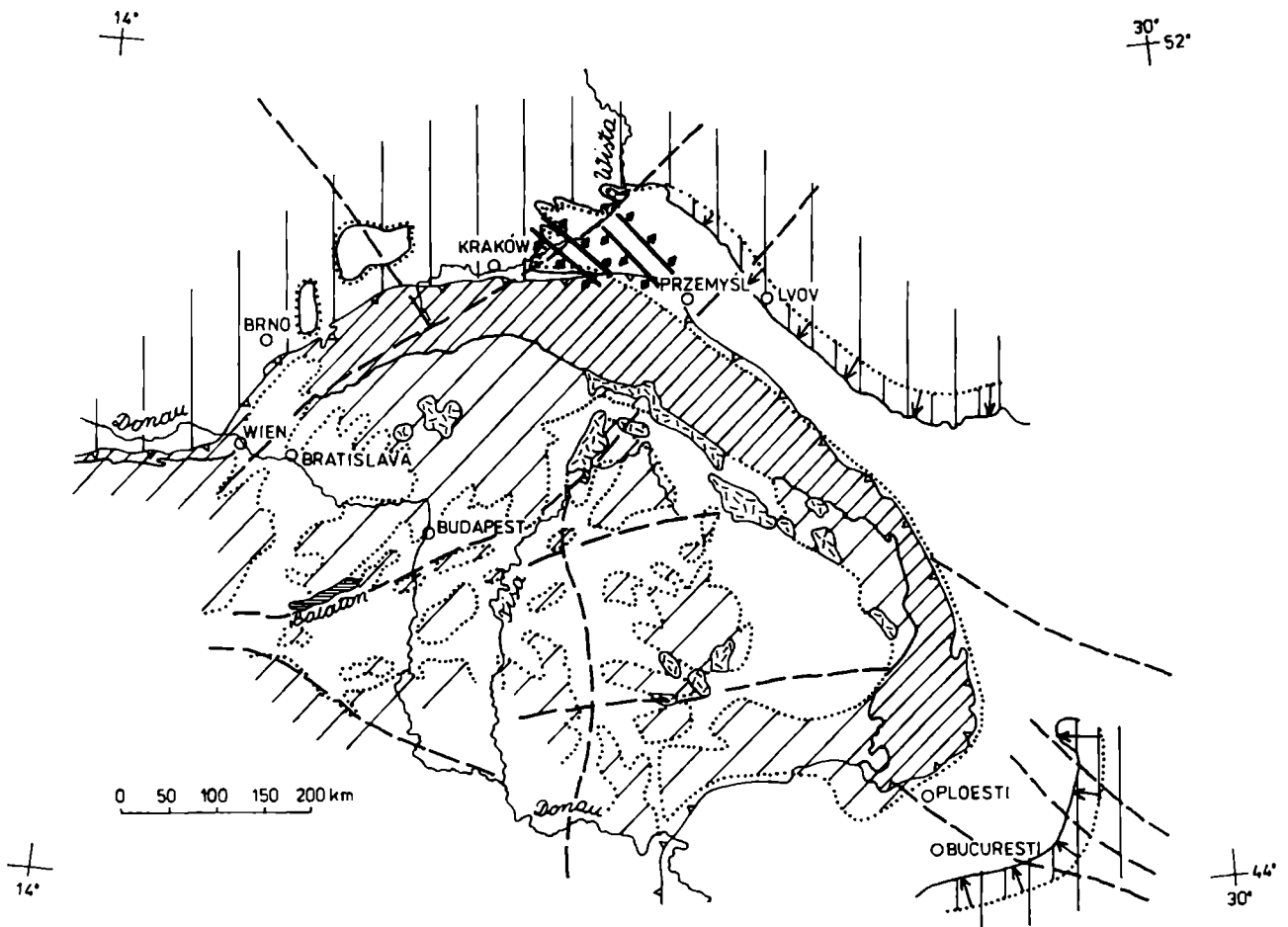
Fig. 11. Early Sarmatian palaeogeography and palaeotectonics of Carpathians. For explanation see Fig. 9
