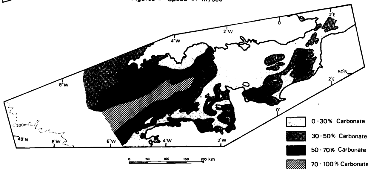
Fig. 5. Sediment type distribution of sea floor sediments in the English Channel (based on Larssonneur et al. , 1979)
