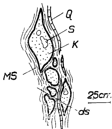
Fig. 2. Kaolinite with relics of feldspars. Cross-section sub-parallel to the bc plane. Q — quartz, S — feldspars; MS — muscovite and sericite; ds — small fractures
