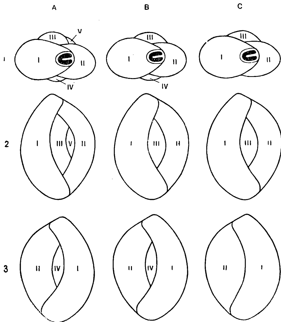
Fig. 1. External structure of tests with quinqueloculine and cryptoquinqueloculine arrangement of chambers. A, B — quinqueloculine tests with five and four external chambers; C — cryptoquinqueloculine test with three external chambers. 1 — apertural side; 2 — many-chambered side; 3 — few-chambered side; I, II, III, IV, V — external chambers counted from the final on
