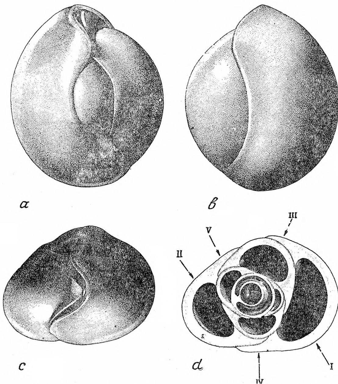
Fig. 5. Miliolinella aff. valvularis (Reuss) ×120. Original sample No. 528/56 in the collection of NIGRI (Leningrad). Peschanokopsk region (North Caucasus). Lower Oligocene ( Spiroplectammina carinata oligocenica beds) (a — many-chambered side; b — few-chambered side; c — apertural side; d — median cross section (polished section); I—V — chambers counted from the final on
