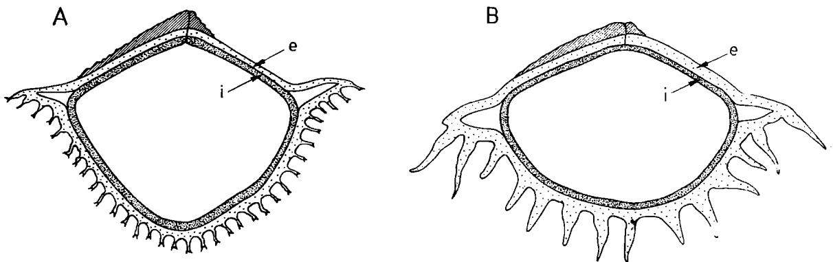
Fig. 2. Diagrammatic reconstructions in polar sections. A. Ancyrospora kedoeae , B. Spinozonotriletes cf. naumovii ; e — exoexine; i — intexine
