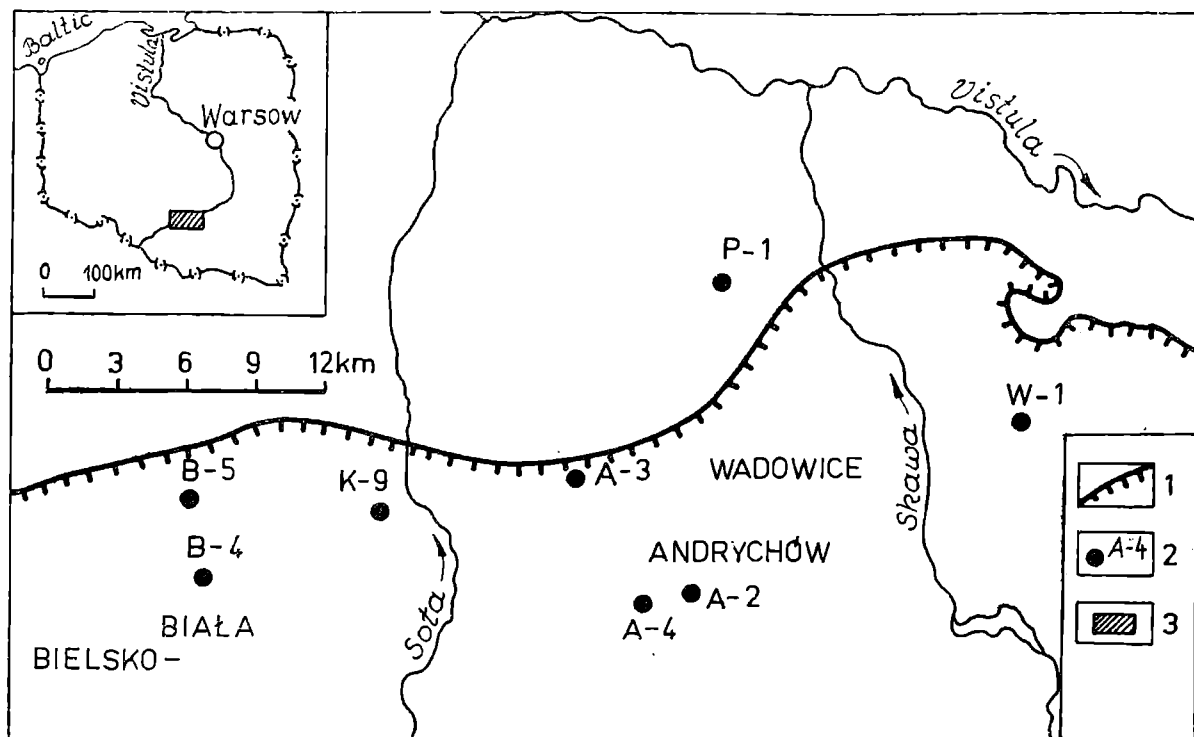
Fig. 1. Sketch map of the area studied with location of boreholes referred to in the text. 1 — northern limit of the Carpathians; 2 — boreholes; B — Bielsko; K — Kęty; A — Andrychów; P — Piotrowice; W — Wysoka; 3 — studied area.
