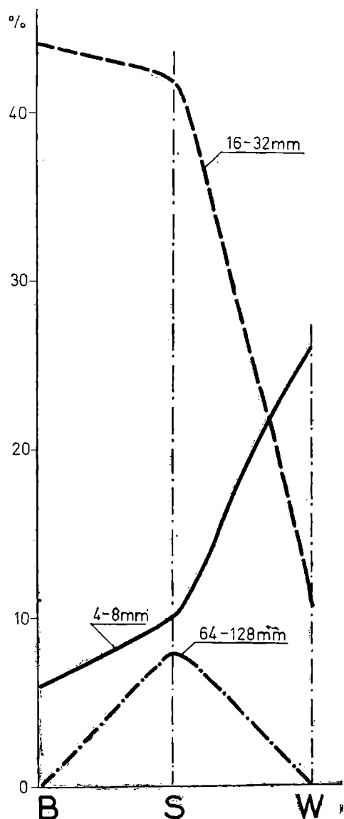
Fig. 5. Content changes of different fractions in conglomerates of the Lower Świerzawa Member: W — Wolbromek; S — Świerzawa; B — Bystrzyca
