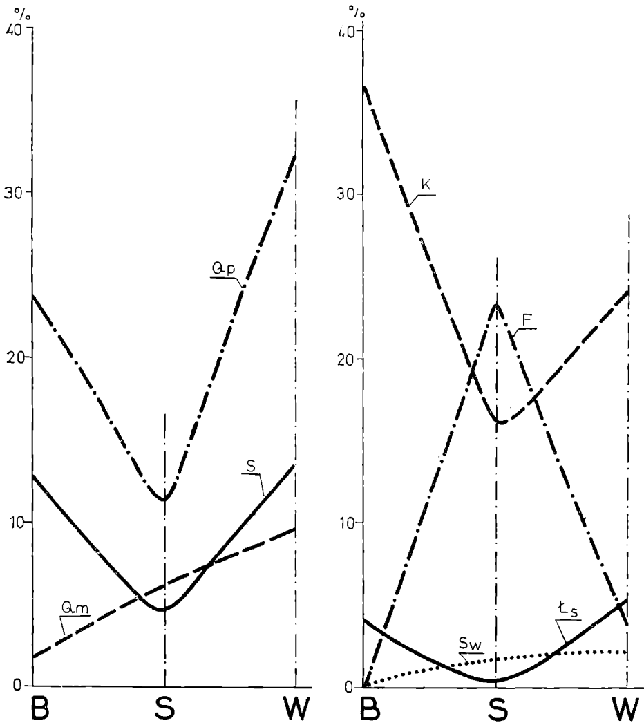
Fig. 9. Content changes of various components in sandstones of the Upper Świerzawa Member: Q p — polycrystalline quartz; Q m — monocrystalline quartz; S — Feldspars; K — quartzites; F — phyllites; S w — eruptive rocks; Ł s — sericite slates; W — Wolbromek; S — Świerzawa; B — Bystrzyca
