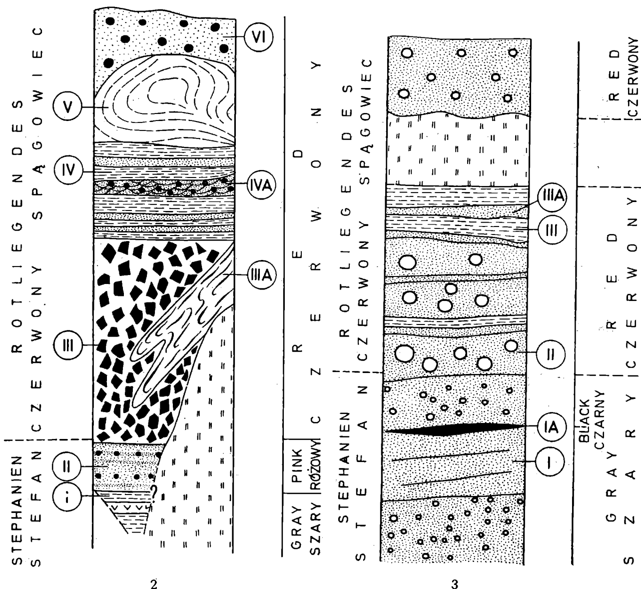
Fig. 2. Synthetic profile of the Stephanian and Rotliegendes in the Wolbromek trough — for further explanations see the text
