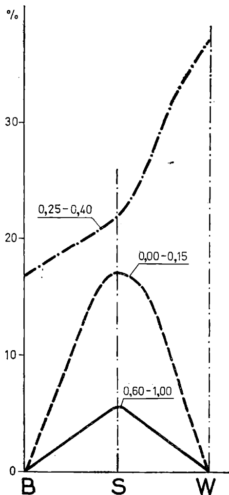
Fig. 4. Content changes of various roundness classes in conglomerates of the Lower Świerzawa Member: W — Wolbromek; S — Świerzawa; B — Bystrzyca
