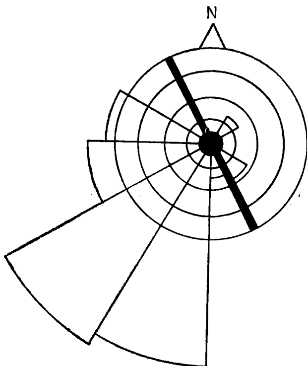
Fig. 12. Imbrication and current marks orientation (thick line) in the exposure near the Świerzawa dam
