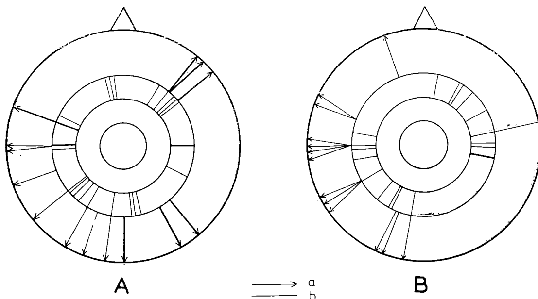
Fig. 10. Comprehensive diagrams of current marks from the Lower (A) and Upper (B) Świerzawa Members; a — flute, b — groove marks
