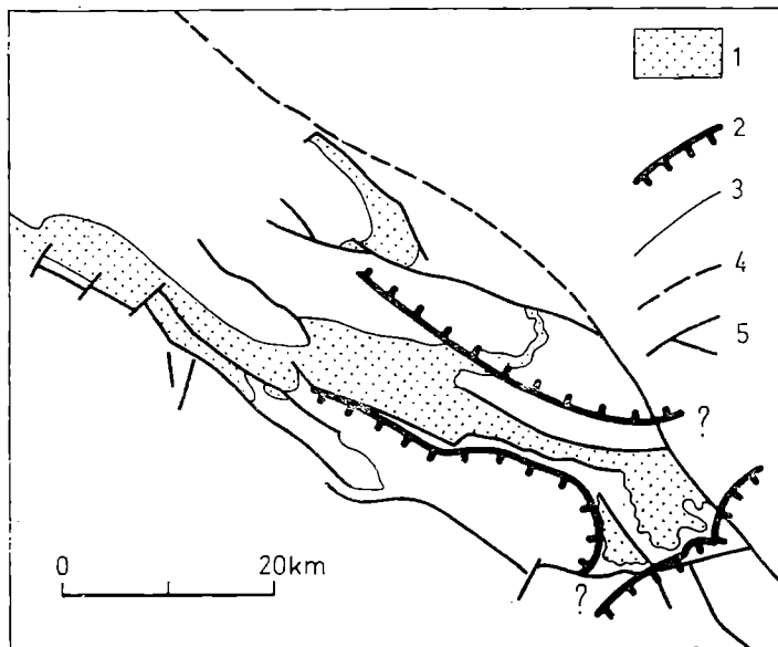
Fig. 13. General paleogeographic situation in the Stephanian and Lower Rotliegendes of the Kaczawa Mountains: 1 — Carboniferous and Lower Permian deposits; 2 — basin margins; 3 — geological boundaries; 4 — supposed faults; 5 — proved faults
