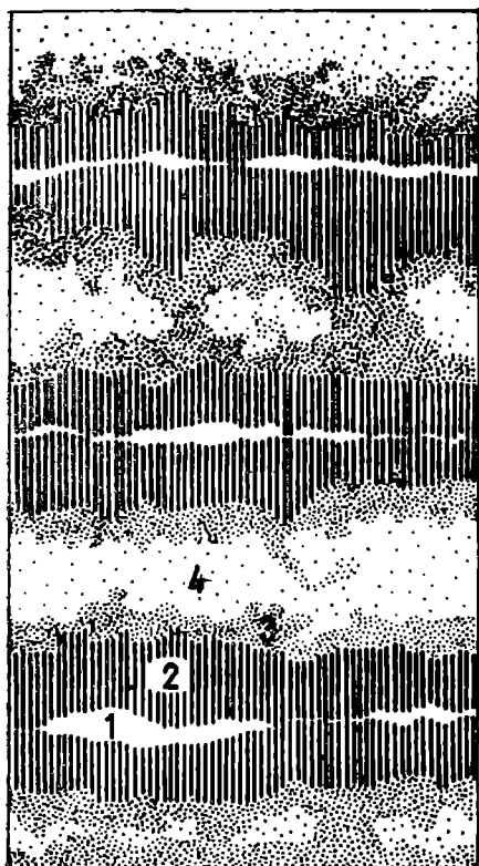
Fig. 3. Diagram showing essentials of ore rhythmus. 1 — solution cavities, 2 — sphalerite incrustations, 3 — sphalerite replacement rims and 4 — relics of unmineralized dolomite
