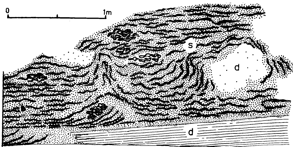
Fig. 5. Cross section of portion of ore body showing contortions resembling or preserving pattern of primary soft-rock deformations. Black lines are sphalerite incrustations lining vugs and sheet cavities. Dotted areas are all dolomite partly or totally replaced by sphalerite
