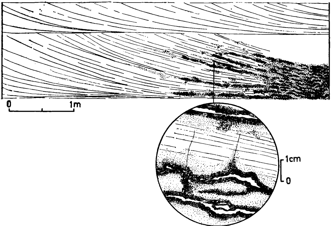
Fig. 2. Contact between mineralized (dotted) and unmineralized parts of a set of cross-strata. Note incongruity between bedding controlled, ore-lined voids (thick lines) and lamination (circle)
