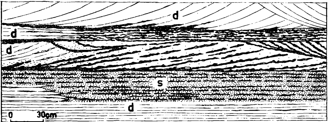
Fig. 1. Section showing contact of sphalerite ores (s) with barren dolomite (d). Ores reflect inherited pattern of cross-stratification and horizontal lamination. Thick lines are sphalerite incrustations lining voids. Dotted areas are dolomite with scattered sphalerite grains. Part of this section is shown in Pl. XXVIII, fig. 1
