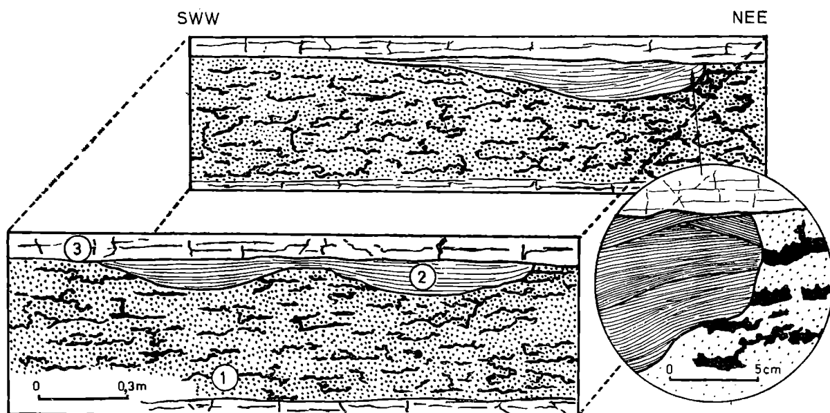
Fig. 3. Dolomite-filled cavity developed in sanded dolomite. Note plano-convex shape of the cave and distinct lamination of cave deposit (2). 1 — disaggregated dolomite with “wermicular” galena veinlets; 2 — laminated cave deposit; 3 — ore-bearing dolomite not affected by solutional disaggregation. Note crosscutting relations between galena veinlets (black patches) and cavity walls (circle-lower right)
