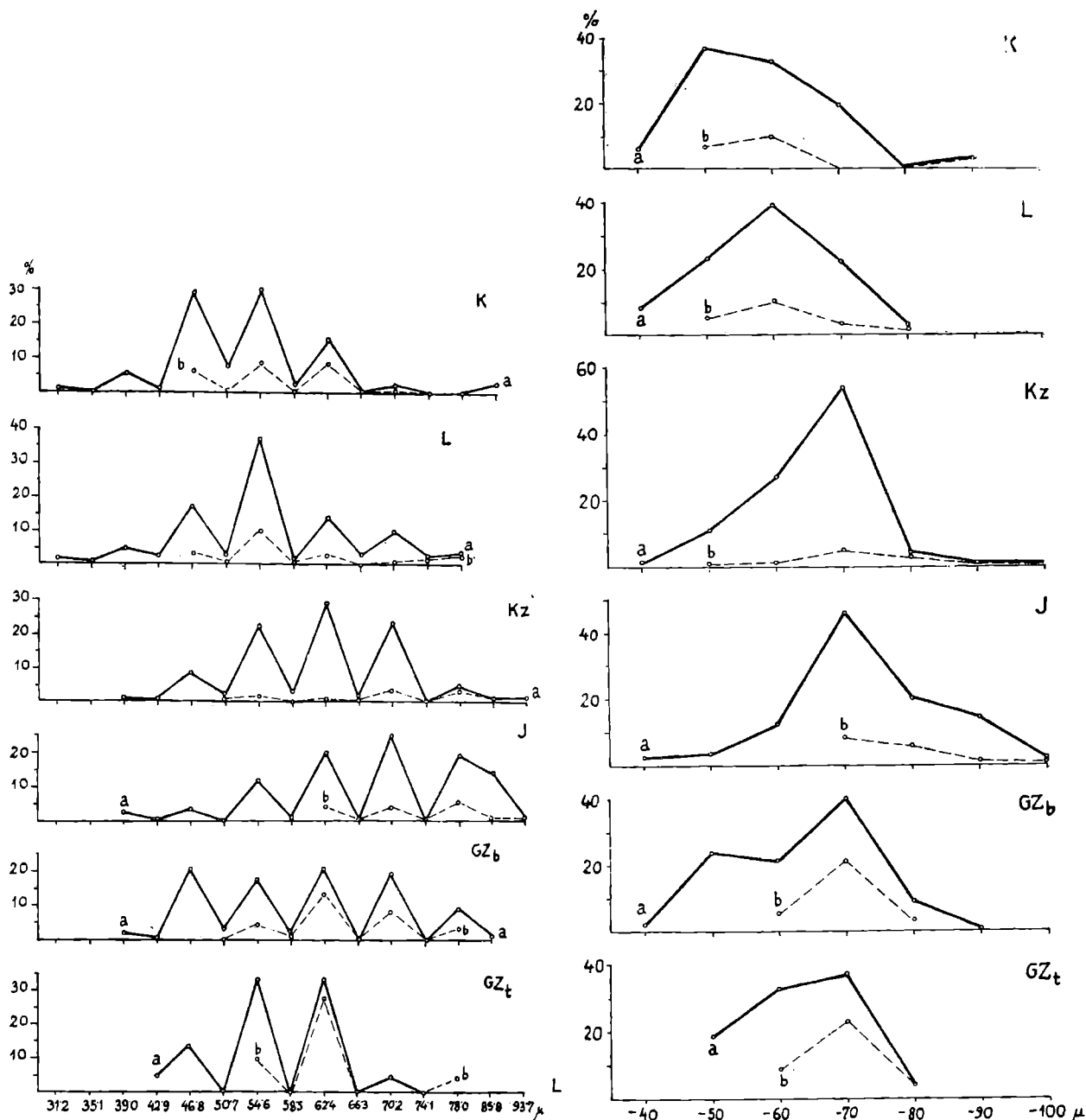
Fig. 7-8. Frequency distribution of length of lorica ( L ) of specimens of Calpionella alpina L.or. (a) and C. elliptica C.ad. (b) in the Upper Tithonian — Berriasian — ?Valanginian Fig. 8 — generalized frequency distribution
