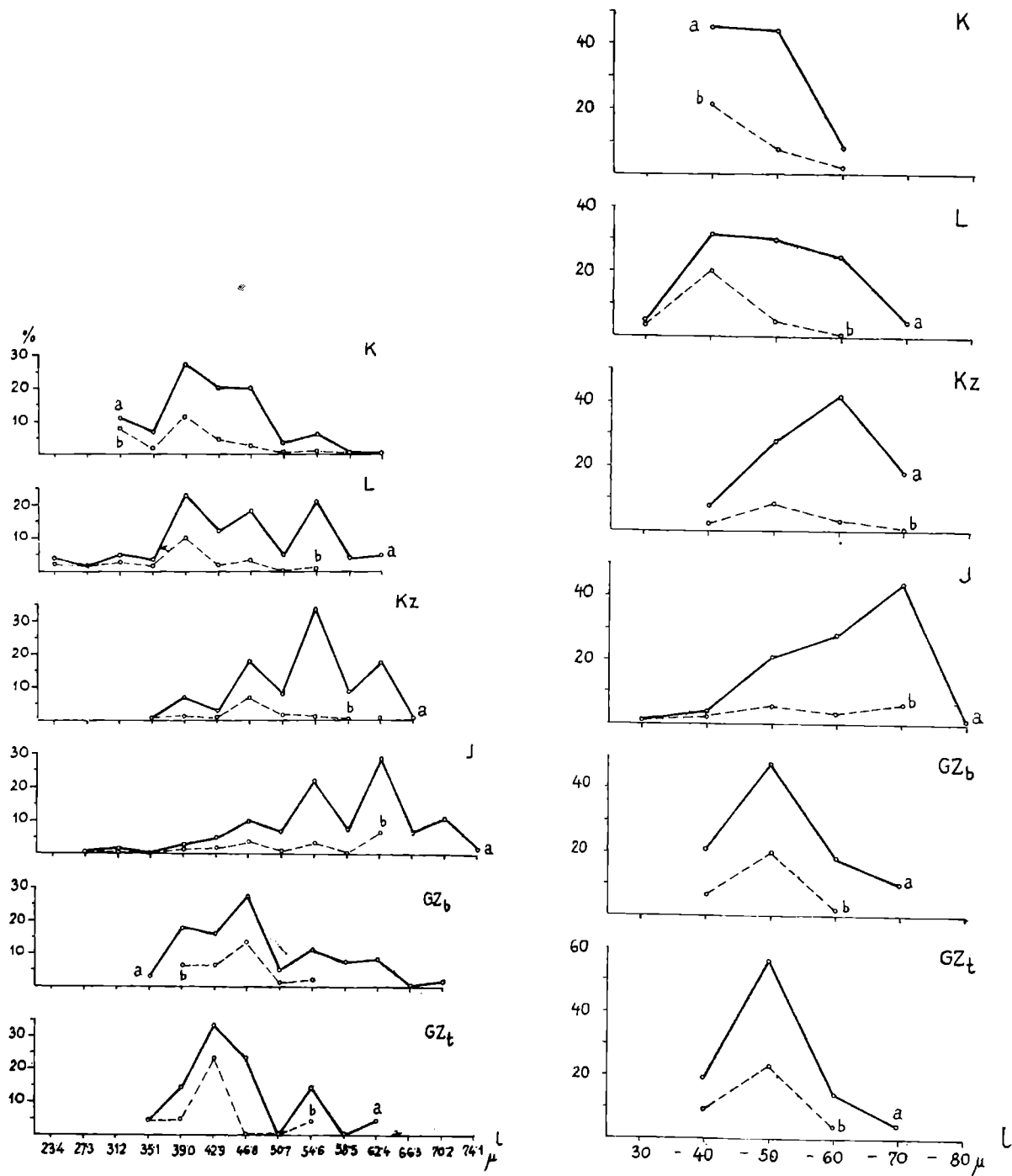
Fig. 9-10. Frequency distribution of width of lorica ( l ) of specimens of Calpionella alpina Lor. (a) and C. elliptica Cad. (b) in the Upper Tithonian — Berriasian — ?Valanginian
