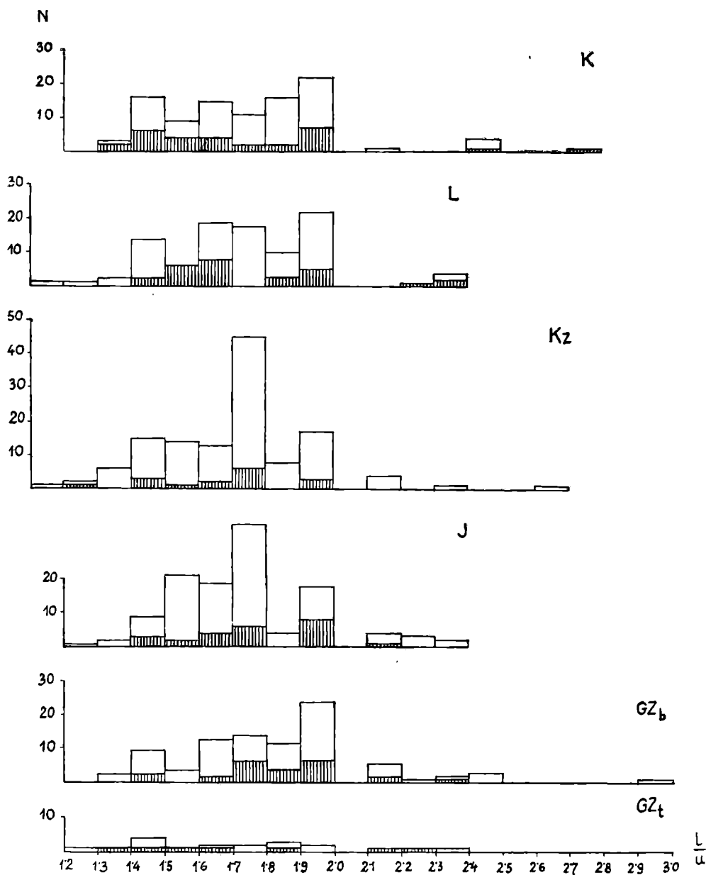
Fig. 13. Variability of the relation l/u of the specimens of Calpionella alpina L or. and C. elliptica C ad. in the Upper Tithonian — Berriasian — ?Valanginian. Explanation of symbols see Fig. 6
