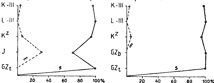
Fig. 14. Frequency distribution of small, medium and large specimens of Calpionella alpina Lor. and C. elliptica Cad. in the Upper Tithonian — Berriasian — ?Valanginian of the Polish Cieszyn Silesia
