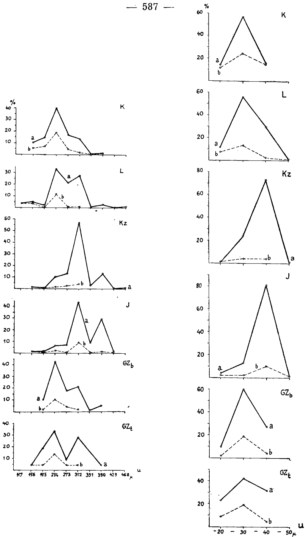
Fig. 11-12. Frequency distribution of width of oral opening ( u ) of specimens of Calpionella alpina Lor. and C. elliptica Cad. in the Upper Tithonian — Berriasian — ?Valanginian
