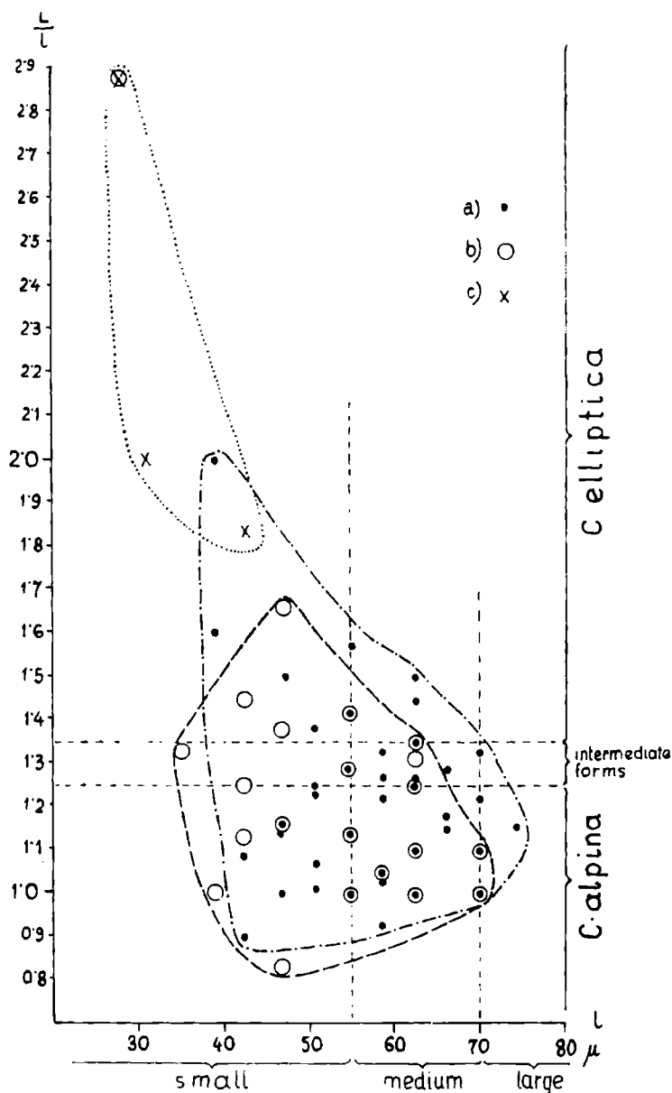
Fig. 4. Calpionella alpina Lor. and C. elliptica Cad. from the lower part of Berriasian in Jasienica. Specimens from a — intrasparites; b — biopelmicrites; c — marls. Other symbols see Fig. 2
