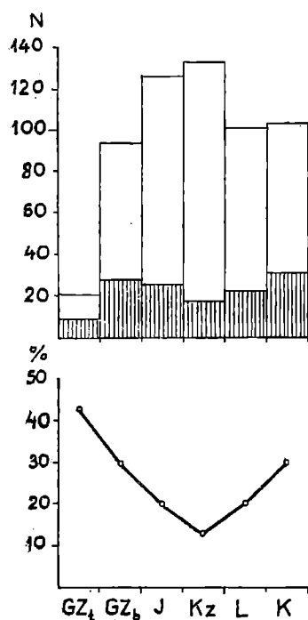
Fig. 6. Frequency distribution of Calpionella alpina L or. and C. elliptica C a d. N—total number of specimens; hatched areas — C. elliptica ; free areas — C. alpina . GZ t — Cieszyn I, Upper Tithonian; GZ b — Cieszyn II, lower part of Berriasian; J — Jasienica, lower part of Berriasian; Kz — Kozy, middle part of Berriasian; L — Lipnik III, upper part of Berriasian; K — Kamienica III, uppermost part of Berriasian — ? Valanginian
