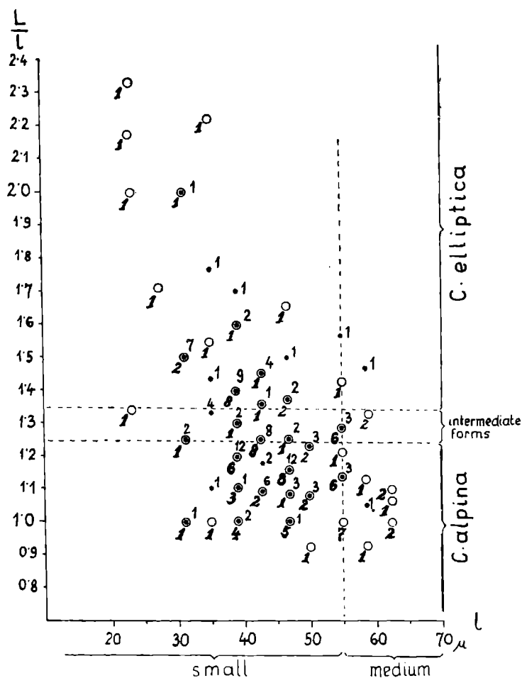
Fig. 5. Calpionella alpina Lor. and C. elliptica Cad. from the upper part of Berriasian in Lipnik III (101 specimens — circles and italics) and 103 specimens from the uppermost Berriasian — ?Valanginian of Kamienica III. Scatter diagram for L/l and l . Other symbols see Fig. 2
