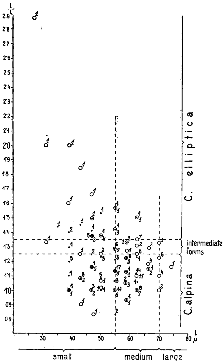
Fig. 3. Calpionella alpina Lor. and C. elliptica Cad. from the lower part of Berriasian in Jasienica (126 specimens — circles and italics) and from the middle part of the Berriasian in Kozy. (133 specimens). Scatter diagram for L/l and l
