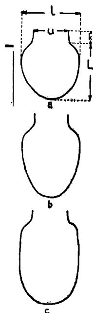
Fig. 1. Schematized outlines of Calpionellae . a — C. alpina Lor.; b — form intermediate between C. alpina and C. elliptica ; c — C. elliptica Cad.; L — length of lorica; l — width of lorica; u — width of oral opening; L/l — elongation of lorica
