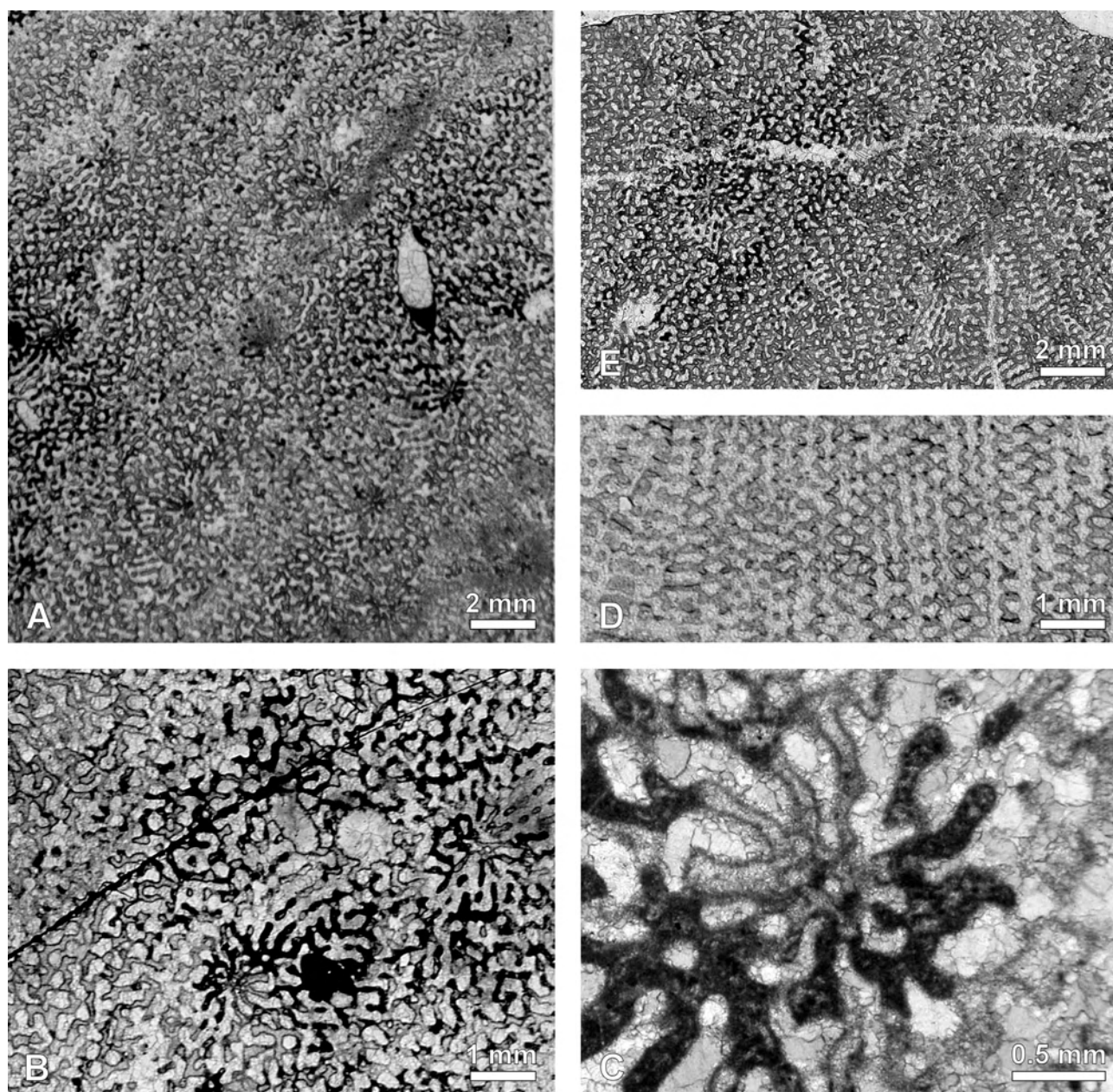
Fig. 7. Microsolena parva sp.n., No. 279, holotype: A – transverse thin section (279a) showing small corallites arranged in series; B, C – detail from Fig. 7A: B – Skeleton not well preserved but outlines of thick trabeculae are marked; C – Corallite with slightly wavy septa S1; D – longitudinal, partly tangential septal section (No. 279b) displaying pennules coalescing into menianes (at left); E – transverse thin section (No. 279c) showing corallites arranged in series
