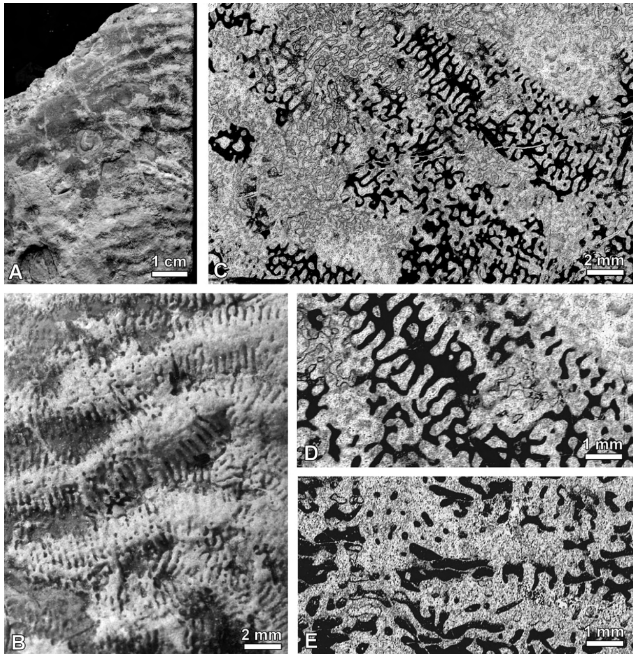
Fig. 15. Meandreaea robusta sp.n., No. 4455/2, holotype: A – upper surface of part of colony showing corallite series arranged subconcentrically; B – enlarged part of Fig. 15A. to show calicular series with small, sub- and nondistinct calicinal fossettes; C – transverse thin section (No. 233a) of corallite series; D – detail from Fig. 15C: septa converging and showing centres of subdistinct calices; E – longitudinal thin section (No. 12b) of septa, partly tangential to the septal surfaces (at left) showing regularly porous radial element with thick menianes. Note also the presence of thin extended dissepiments
