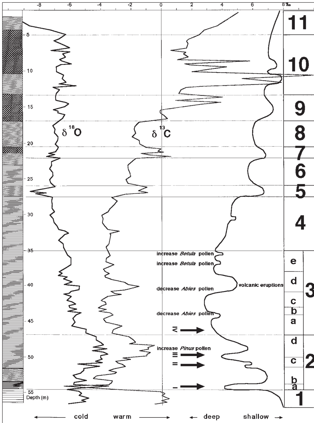
Fig. 20. Isotope horizons (1,2,...) and sub-horizons (a,b,...) of the Mazovian Interglacial and the initial part of the Middle Polish Glaciation, versus probable changes of water level in the palaeolake and isotopes for calcareous sediments in the Ossówka OS 1/96 borehole; arrows indicate increased marine influence; for lithological explanations see Text-fig. 8
