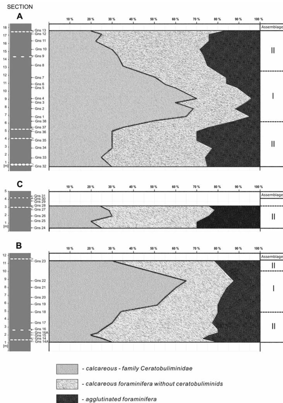
Text-fig. 4. Relative abundance (%) of calcareous and agglutinated foraminifers and distinguished type of foraminiferal assemblages (I and II) in the Gnaszyn sections A, B and C
