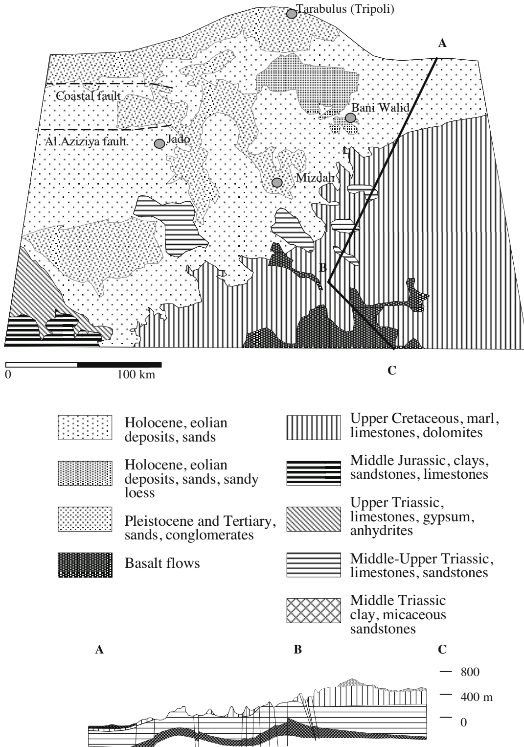
Text-fig. 2. Schematic geological map and N-S cross-section
