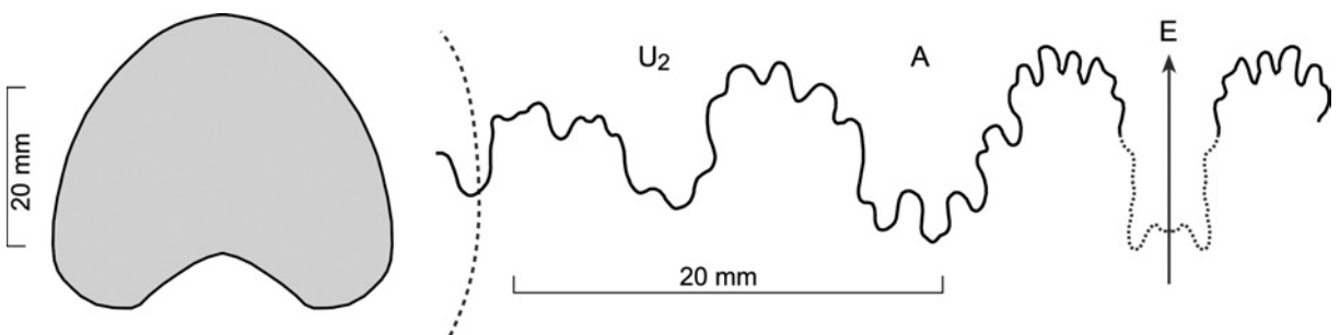
Text-fig. 7. Whorl section and suture line of Vascoceras cauvini Chudeau, 1905, Upper Cenomanian of the Galala Formation, specimen AfK 302
