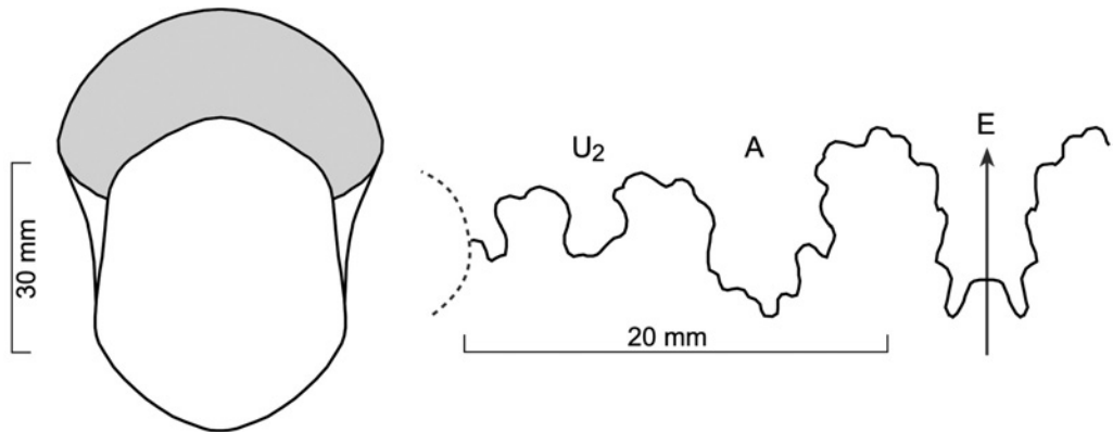
Text-fig. 10. Whorl section and suture line of Vasoceras kossmati Choffat, 1898, Lower Turonian of the Galala Formation, specimen AfK 309
