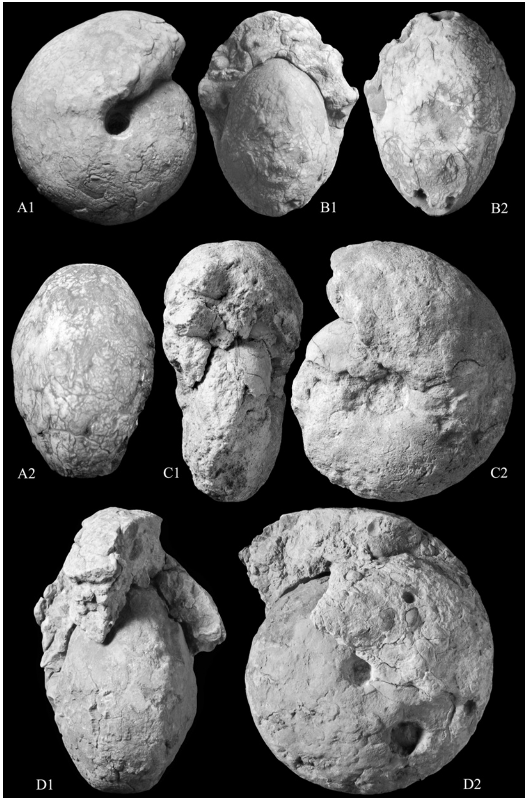
Text-fig. 13. A – Vascoceras kossmati Choffat, 1898 (A1, A2 – lateral and ventral views of AfK 311, \times 1 ). B – Neoptychites cephalotus (Courtillet, 1860) (B1, B2 – apertural and ventral views of AfK 313, \times 1 ). C – Thomasites gongilensis (Woods, 1911) (C1, C2 – apertural and lateral views of AfK 314, \times 1 ). D – Thomasites rollandi (Thomas and Peron, 1889) (D1, D2 – apertural and lateral views of AfK 316, \times 1 ). All specimens from the Lower Turonian of the Galala Formation
