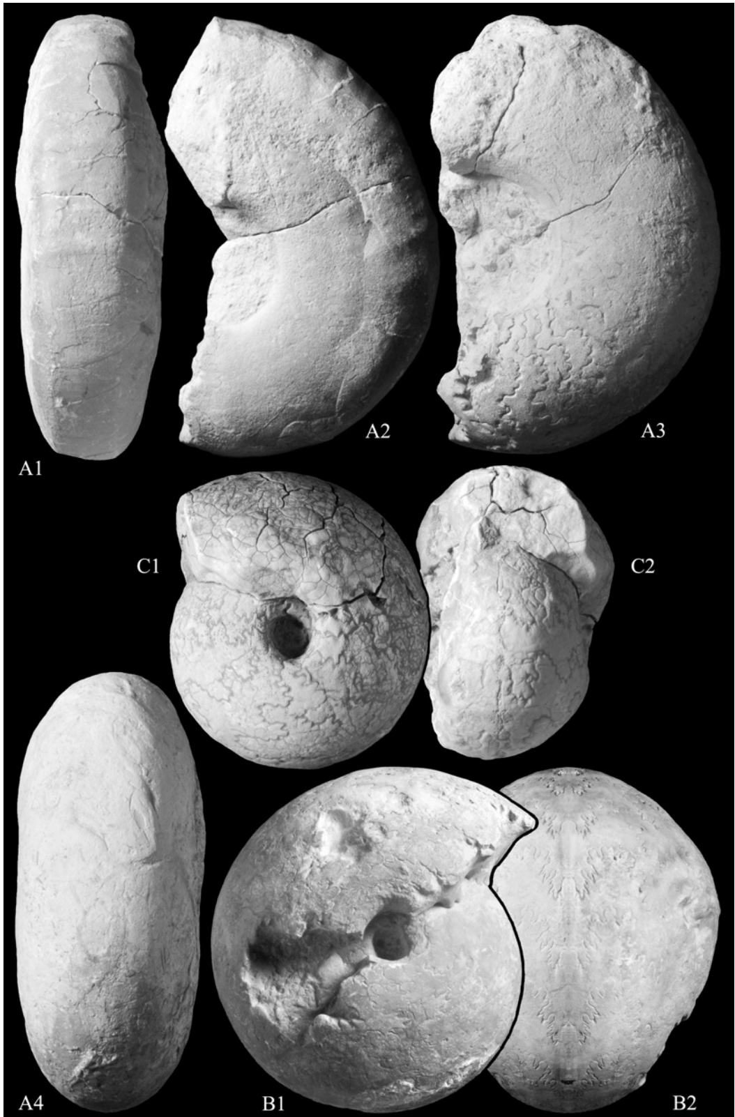
Text-fig. 9. A – Vascoceras cauvini Chudeau, 1909 (A1, A2 – ventral and lateral views of AfK 303, \times 1 ; A3, A4 – lateral and ventral views of AfK 302, \times 1 ; Upper Cenomanian of the Galala Formation). B – Vascoceras globosum globosum (Reyment, 1954) (B1, B2 – lateral and ventral views of AfK 308, \times 1 ; Lower Turonian of the Galala Formation). C – Vascoceras kossmati Hoffât, 1898 (C1, C2 – lateral and apertural views of AfK 309, \times 1 ; Lower Turonian of the Galala Formation)
