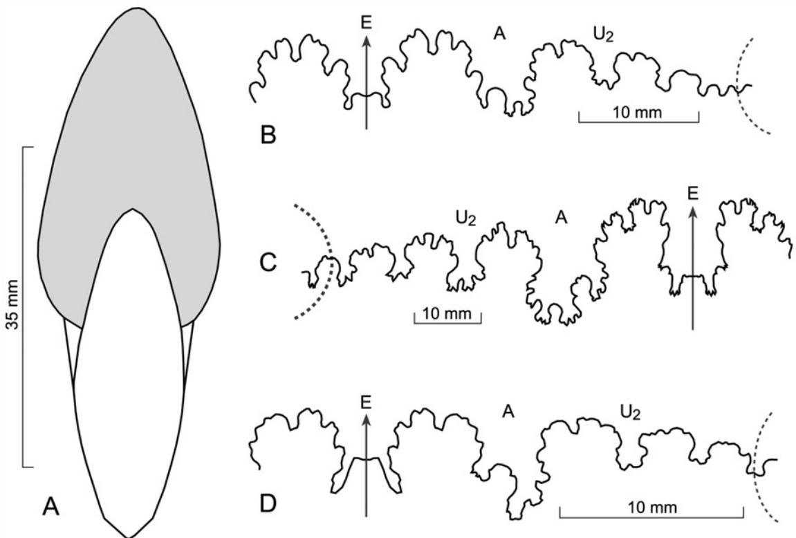
Text-fig. 18. Whorl section and suture line of Choffaticeras ( Choffaticeras ) segne (Solger, 1903), Lower Turonian of the Galala Formation, A, B – specimen AfK 321;
