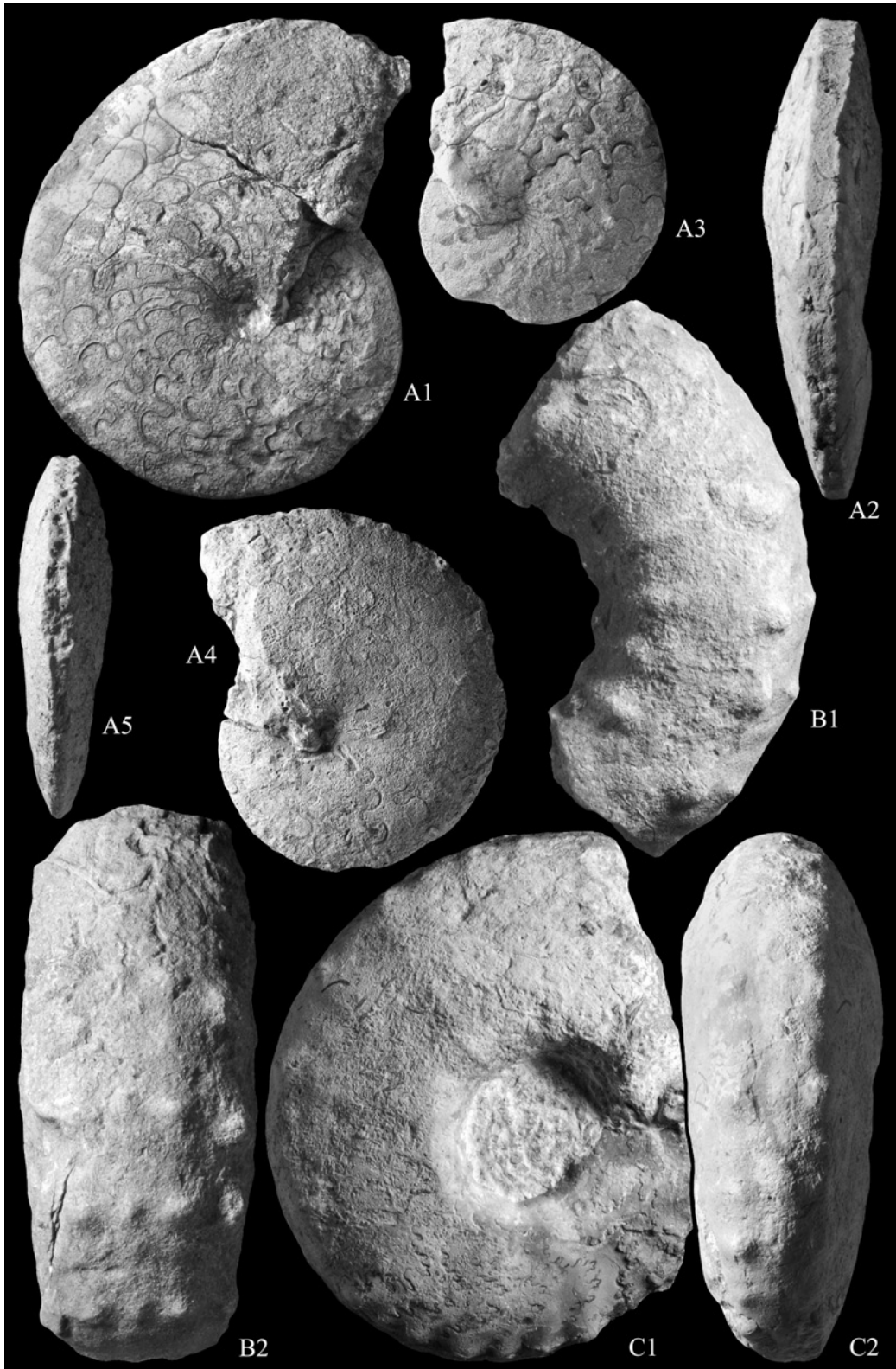
Text-fig. 6. A – Neolobites vibrayeanus (d’Orbigny, 1841) (A1, A2 – lateral and ventral views of AfK 298, \times 1 ; A3 – lateral view of AfK 300, \times 1 ; A4, A5 – lateral and ventral views of AfK 301, \times 1 ). B – Euomphaloceras costatum Cobban, Hook and Kennedy, 1989 (B1, B2 – lateral and ventral views of AfK 305, \times 1 ). C – Pseudaspidoceras sp. (C1, C2 – lateral and ventral views of AfK 304, \times 1 ). All specimens from the Upper Cenomanian of the Galala Formation
