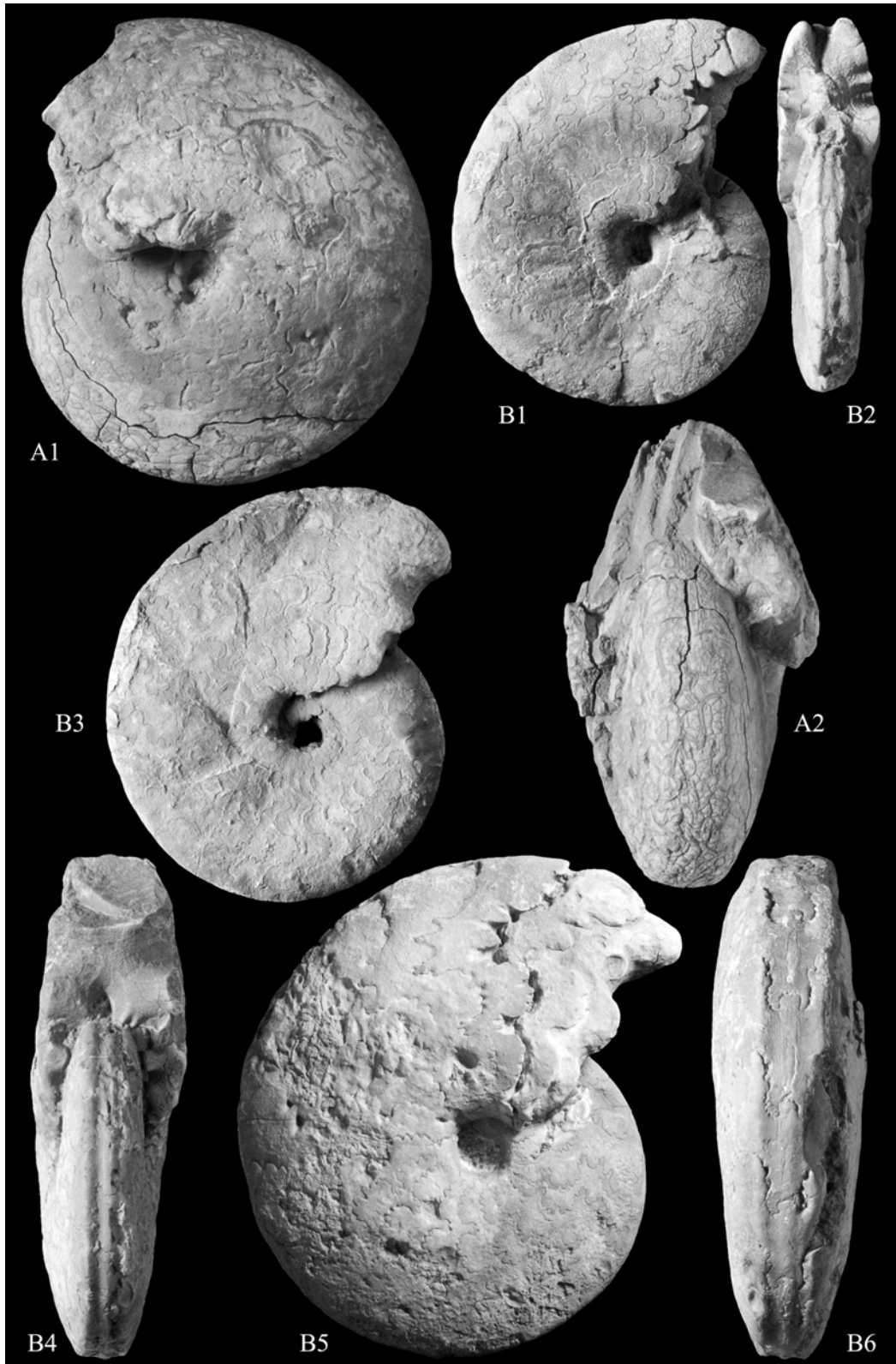
Text-fig. 16. A – Thomasites rollandi (Thomas and Peron, 1889) (A1, A2 – lateral and apertural views of AfK 315, \times 1 ). B – Pseudotissotia nigeriensis (Woods, 1911) (B1, B2 – lateral and apertural views of AfK 328, \times 1 ; B3 – lateral view of AfK 334, \times 1 ; B4, B5, B6 – apertural, lateral and ventral views of AfK 329, \times 1 ). All specimens from the Lower Turonian of the Galala Formation
