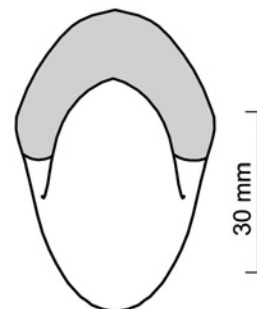
Text-fig. 11. Whorl section of Neoptychites cephalotus (Courtyiller, 1860), Lower Turonian of the Galala Formation, specimen AfK 313
