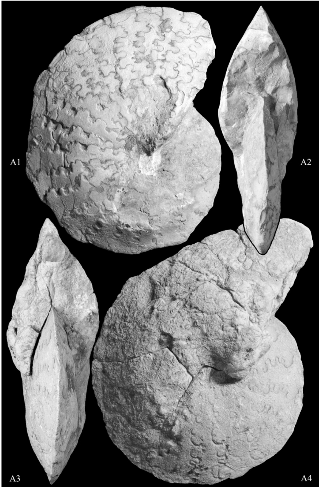
Text-fig. 21. Coilopoceras requienianum (d'Orbigny, 1841) from the Upper Turonian of the Umm Omeiyid Formation. A1, A2 – lateral and apertural views of AfK 339, \times 1 ;
