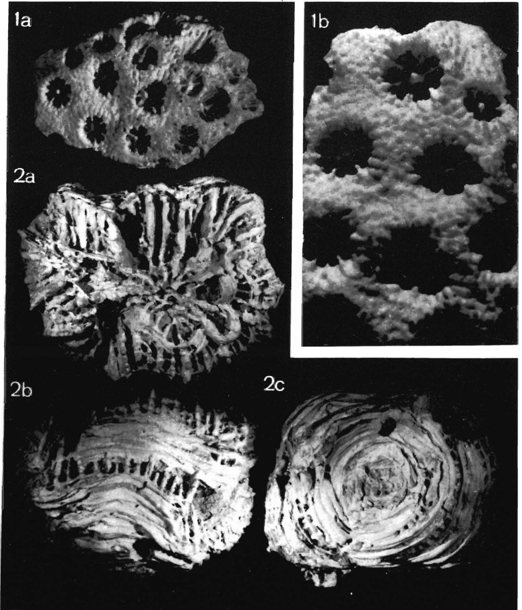
1 — Stylophora reussiana MONTANARO-GALLITELLI & TACOLI; ZPAL H. I/559; 1a —incipient colony, \times 10 , 1b —detail of Fig. 1a, \times 20 ; note intercorallite granulation and differentiation of septa SI into thick, exsert peripheral and thin, deeply hidden parts 2 — Syzygophyllia brevis REUSS; ZPAL H. I/572; 2a — distal view [note evidence of initial budding ( arrows )], 2b — lateral view, 2c — proximal view; all \times 2
