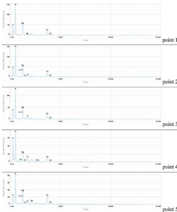
Text-fig. 6. Microphotography of the PSK sample with points of analysis, BSE and EDS spectra.
