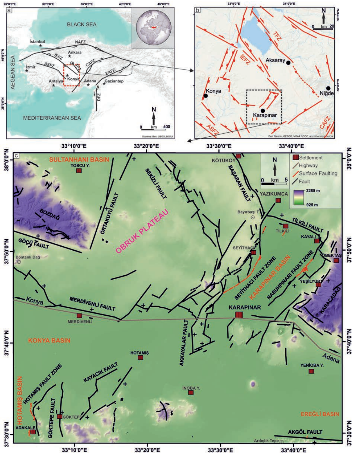
Text-fig. 1. Location map of the study area, (a) Major tectonic structures of Central and Western Anatolia (NAFZ: North Anatolian fault zone, EAFZ: East Anatolian fault zone, DSFZ: Dead Sea fault zone, CAFZ: Central Anatolian fault zone, TFZ: Tuz Gölü fault zone, IEFZ: İnönü - Eskişehir fault zone, ASFZ: Akşehir fault zone), (b) Important faults around the study area, (c) Morphometric map of Karapınar region with main faults.
