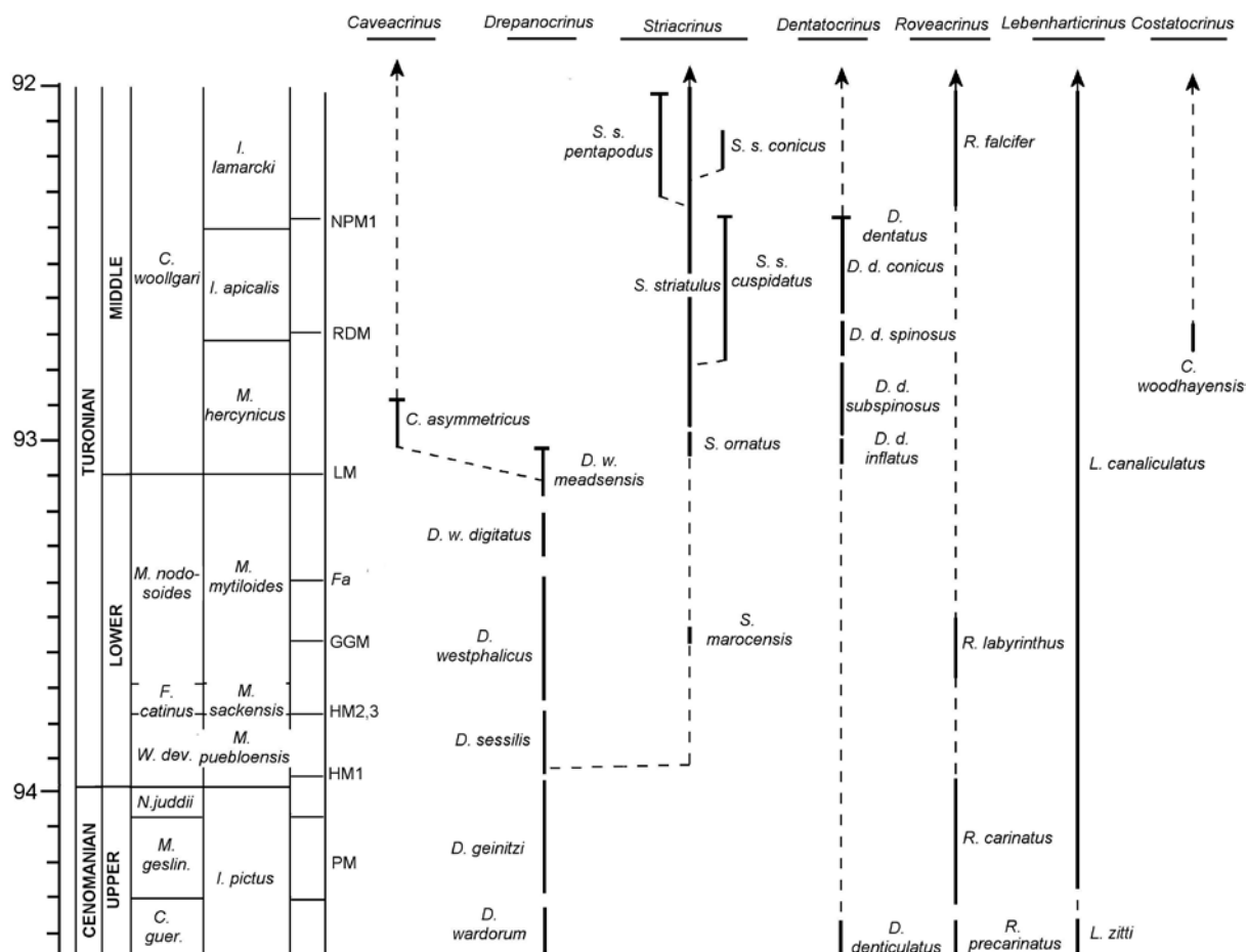
Text-fig. 4. Proposed phylogeny of saccocomid and roveacrinid microcrinoids in the Cenomanian–middle Turonian of the Anglo-Paris Basin. The ancestry of Caveacrinus is uncertain. Abbreviations: Lithological markers: PM – Plenus Marl, HM1–3 – Holywell Marls, GGM – Gun Gardens Marls, Fa – Filograna avita Bed, LM – Lulworth Marl, RDM – Round Down Marl, NPM1 – New Pit Marl 1. Ammonite zones: C. guer. – Calyoceras guerangeri Zone, M. geslin. – Metoicoceras geslinianum Zone, N. juddii – Neocardioceras juddii Zone, W. dev. – Watinoceras devonense Zone, F. catinus – Fagesia catinus Zone, M. nodosoides – Mammites nodosoides Zone, C. woollgari – Collignoniceras woollgari Zone. Inoceramid zones: I – Inoceramus , M – Mytiloides .
