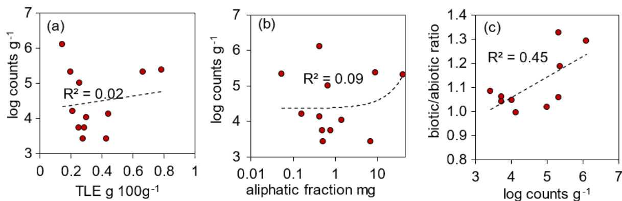
Text-fig. 7. Rectilinear correlation between number of microorganisms (log counts g -1 ) and TLE content (a), aliphatic fraction content (b, logarithmic scale) and biotic/abiotic ratio (c). R^2 – coefficient of determination.
