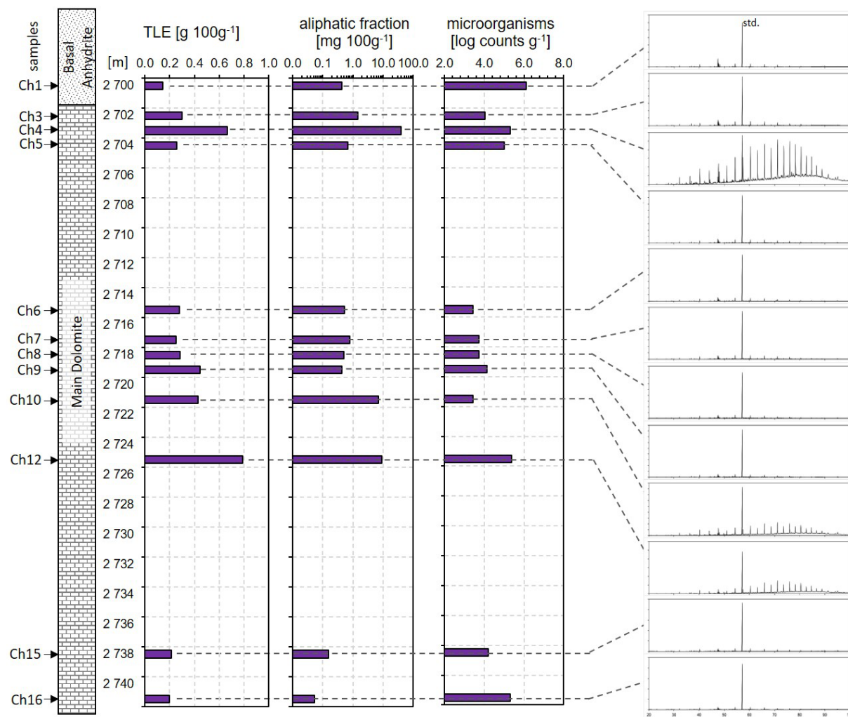
Text-fig. 4. Total lipid extract ( \text{g } 100 \text{ g}^{-1} of rock sample), content of aliphatic fraction ( \text{mg } 100 \text{ g}^{-1} of rock sample) and number of microorganisms in samples (Ch1–Ch16) obtained from C-1 core. On the right, the TLE chromatograms were presented in the same scale for comparison (std. – internal standard).
