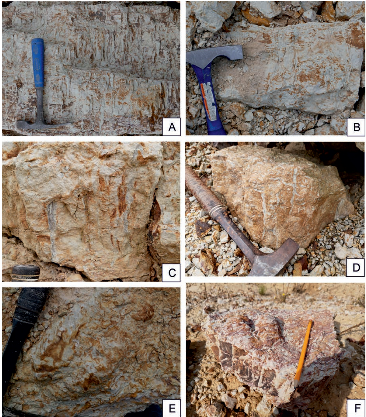
Text-fig. 8. Examples of ichnofossils from the middle shoreface deposits of Dziwiątle Quarry. A – Skolithos isp. from complex K (sub-association 3c); B – Diplocraterion isp. from complex K (sub-association 3c); C – Rosselia isp. from complex I.2 (sub-association 3b); D – ?Lennea isp. from complex J (sub-association 3c); E – Rusophycus isp. from complex H.1 (sub-association 3a); F – Rusophycus dispar (Linnarsson, 1871) from complex I.1 (sub-association 3b).
