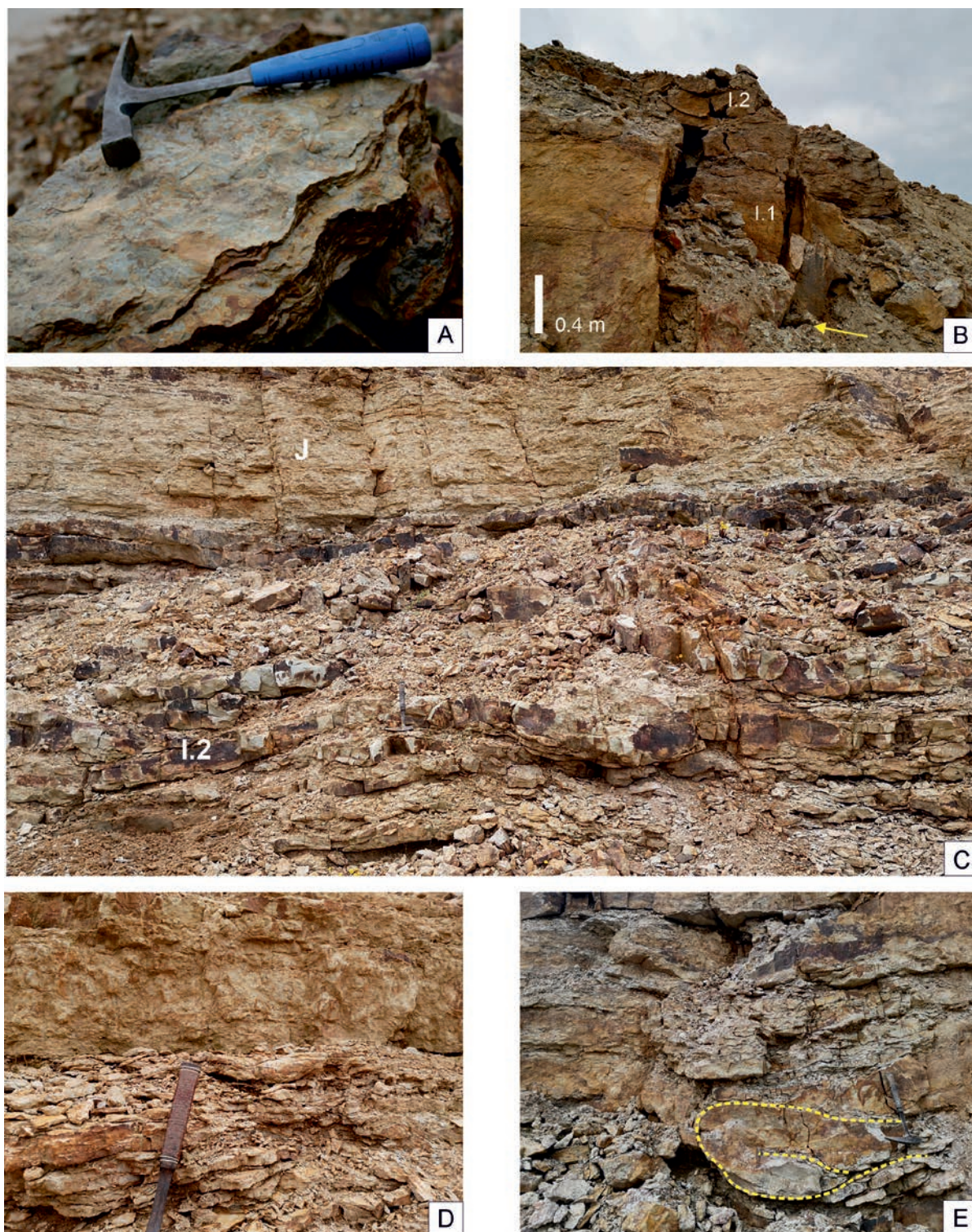
Text-fig. 7. Sedimentological features of lower shoreface (A) and middle shoreface (B–E) deposits of Dziwiątł Quarry. A – Sandstones with symmetrical ripple marks of complex E (sub-association 2a); B – Massive sandstones of complex I.1 (sub-association 3b) and sandstones with HCS of complex I.2 (sub-association 3b); yellow arrow marks the basal erosional surface of complex I.1; C – Sandstones with HCS of complex I.2 (sub-association 3b), gradually passing into sandstones with wave ripple marks, overlain by silty sandstones with wave ripple marks of complex J (sub-association 3c); D – Sandy beds with small scale wave ripple marks of complex J (sub-association 3c); E – Syn-sedimentary fold in sandstones with HCS of complex I.2 (sub-association 3b).
