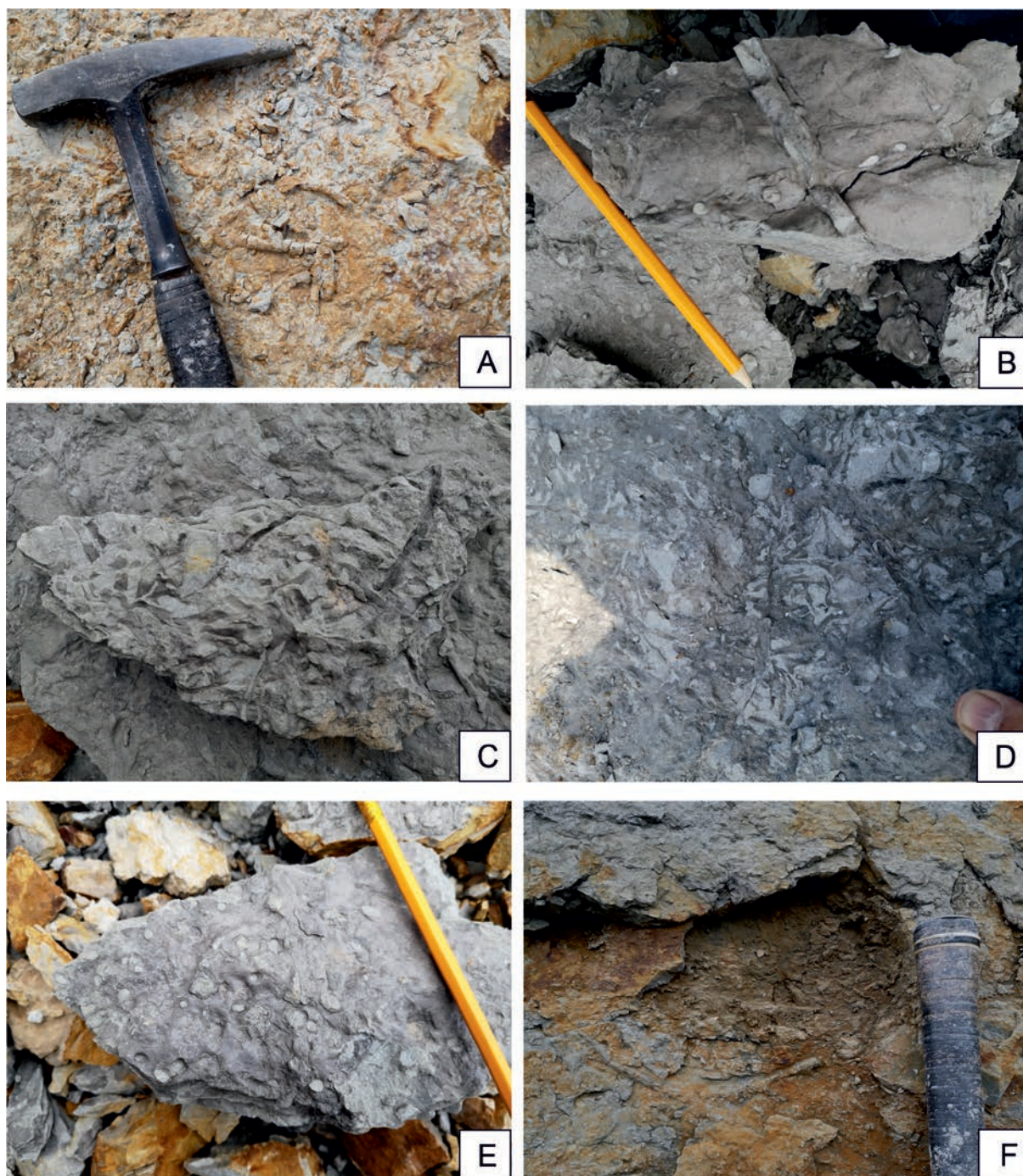
Text-fig. 6. Examples of ichnofossils from the middle shoreface (A), lower shoreface (B–E) and offshore (F) deposits of Dziewiątle Quarry. A – Planolites isp. (sub-association 3a, complex H.2); B – Palaeophycus isp. (sub-association 2a, complex E); C, D – Phycodes isp. (sub-association 2a, complex D); E – Monocraterion isp. (sub-association 2a, complex E); F – Syringomorpha isp. (sub-association 1b, complex B).
