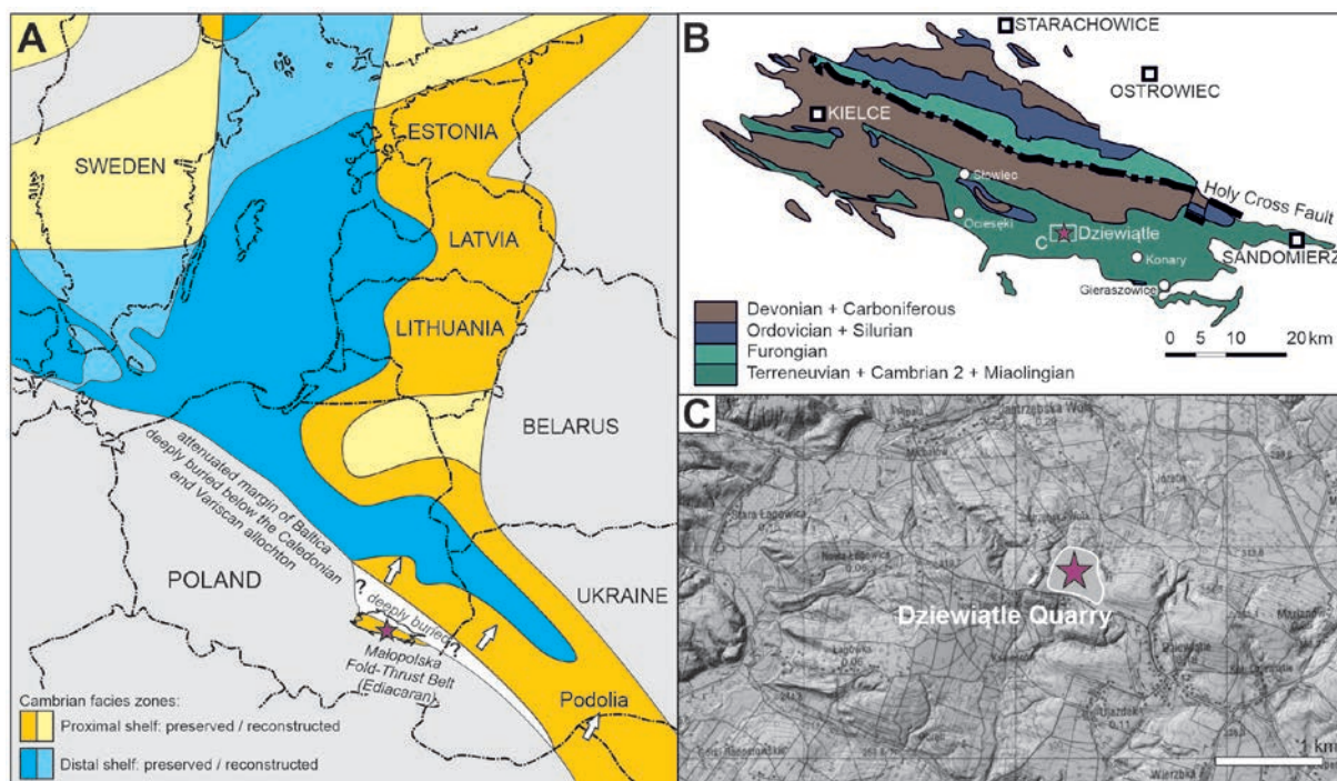
Text-fig. 1. Location of Dzięwiątł Quarry (violet star) with regard to: A – Palaeogeography and general facies distribution during the late part of Cambrian Stage 2 in the SW part of Baltica; based on Rozanov and Lydka (1987), Nielsen and Schovsbo (2011), Stadnik et al. (2019, fig. 8), and Wendorff (2019); white arrows point to transport directions, those for Podolia (Ukraine) are according to Paszkowski et al. (2021); B – Generalized geological map of the Palaeozoic inlier of the Holy Cross Mountains (after Czarnocki 1957), and C – LiDAR map, background map downloaded from https://mapy.geoportal.gov.pl accessed on 19.04.2024.
