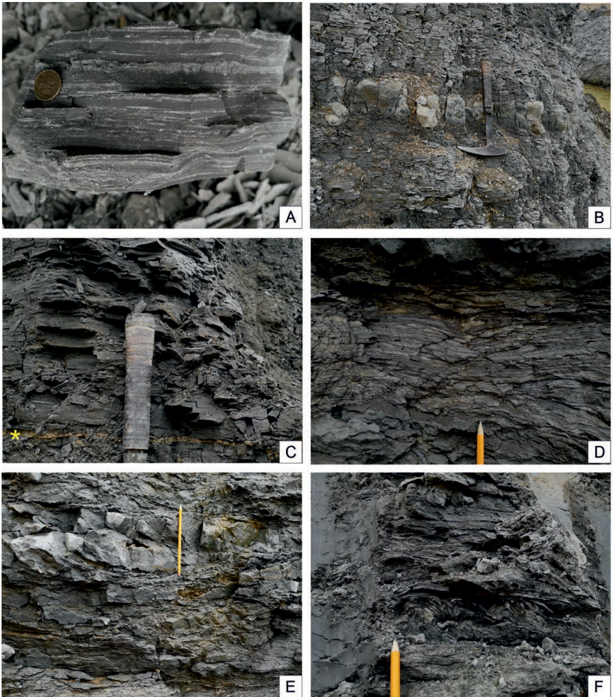
Text-fig. 5. Sedimentological features of offshore deposits exposed in Dziwiątle Quarry. A – Dark grey horizontally laminated silty mudstones of complex A (sub-association 1a) with intercalations of bioturbated sandy beds; B – Discrete irregular thin laminae of silt in the horizontally laminated mudstones of complex A (sub-association 1a); C – Dark grey horizontally laminated mudstones of complex B (sub-association 1b); yellow star indicates yellow tuffite lamina; D – Grey heteroliths of complex F (sub-association 1b) with flaser and wavy lamination; pencil points to post-depositional convolutions; E – Grey heteroliths of complex F (sub-association 1b) with cross-bedded sandy lenses (length of pencil 18 cm); F – Convolute beds of grey heteroliths of complex F (sub-association 1b).
