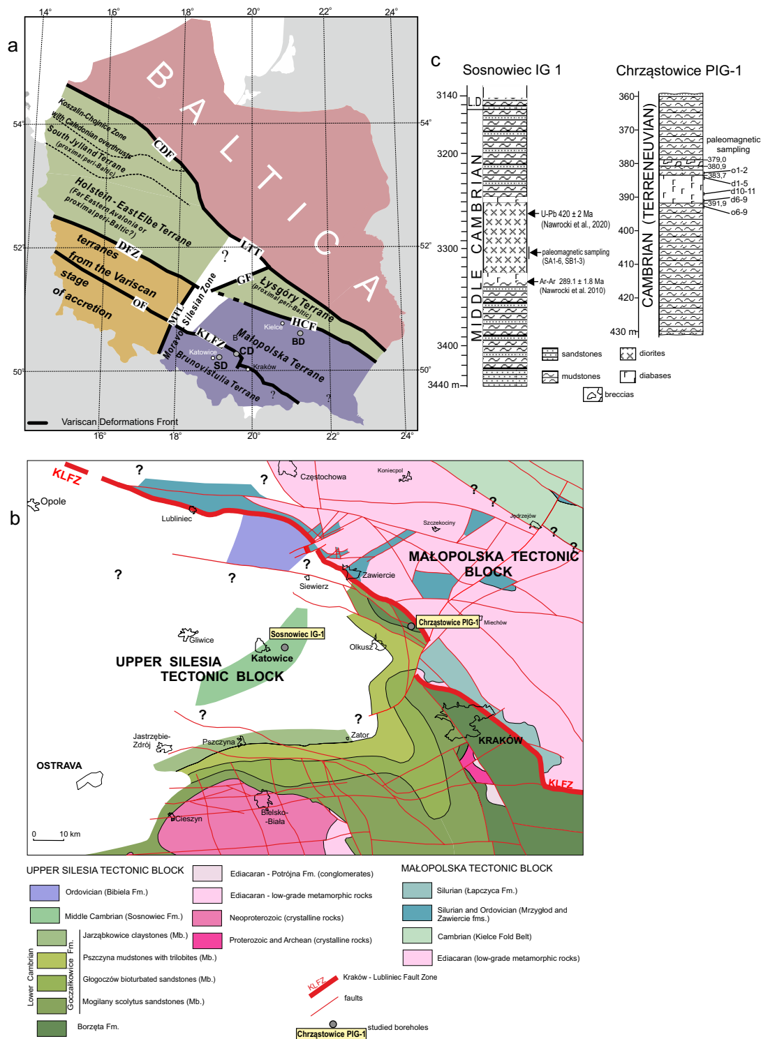
Text-fig. 1. (a) The location of Chrząstowice PIG-1 and Sosnowiec IG-1 sampling sites for palaeomagnetic study on the map of terranes in Poland (see Nawrocki 2015) (CDF – Caledonian Deformation Front, LTT – Teisseyre-Tornquist tectonic line, GF – Grójec Fault, DFZ – Dolsk Fault Zone, OF – Odra Fault, KLFZ – Kraków-Lubliniec Fault Zone, MTL – Moravian Tectonic Line, HCF – Holy Cross Fault, SD – Sosnowiec IG1 borehole with diorite intrusion, BD – Bardo diabase, CD – Chrząstowice diabase). (b) Simplified geological map of the contact zone between the Małopolska and Upper Silesia tectonic blocks (after Buła and Habryn 2015), with studied boreholes marked. (c) Simplified lithological columns of Middle Cambrian rocks cut by magmatic intrusions drilled in the Sosnowiec IG-1 and Chrząstowice PIG-1 boreholes. Location of samples for palaeomagnetism and isotope age estimations are marked.
