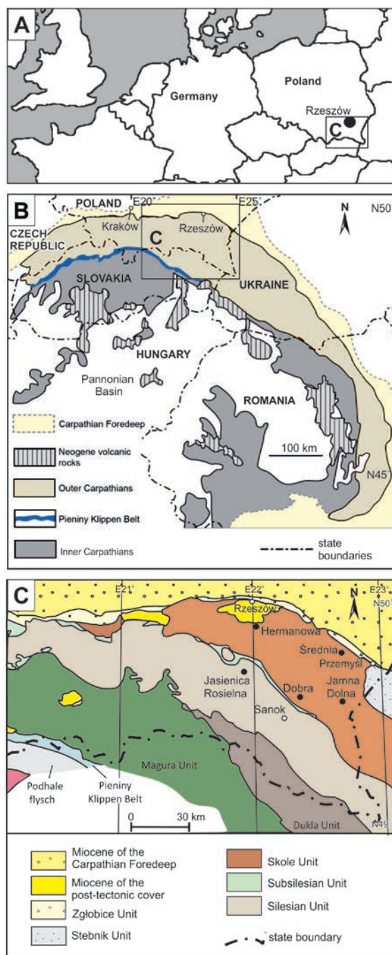
Text-fig. 1. Location maps. A – Study area within Central Europe; B – Study area within simplified geological map of the Outer Carpathians (modified from Kováč et al. 1998); C – Localities where the specimens were collected (black dots) within simplified geological map of the Polish part of the Outer Carpathians (modified from Żytko et al. 1989).
