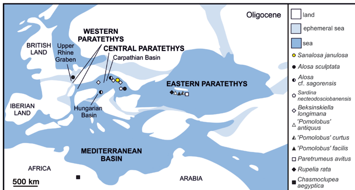
Text-fig. 10. Paleobiogeography of representatives of the Order Clupeiformes in the Oligocene based on skeleton findings; palaeogeography adopted from Popov et al. (2002).
