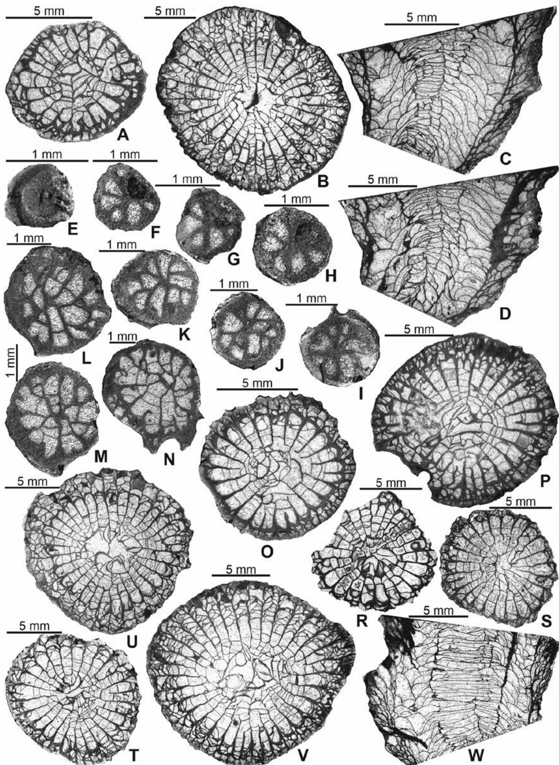
Text-fig. 8. Yuanophylloides (Patulaxis) molestus sp. nov. Transverse sections, except when stated otherwise. A–D – USNM PAL 795352, holotype; A – late neanic/early mature growth stage, B – mature growth stage, C, D – longitudinal sections; C – centric, D – slightly eccentric. E–P – USNM PAL 795353; E – brephic growth stage, F–N – neanic growth stage, O – early mature growth stage, P – mature growth stage. R–W – USNM PAL 795354. R, S – late neanic/early mature growth stage, T – early mature growth stage, U, V – mature growth stage, W – centric longitudinal section. For stratigraphic positions see text.
