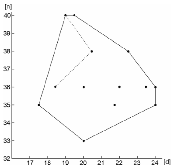
Text-fig. 14. Yuanophylloides (Patulaxis) parvus sp. nov.; n:d values of selected specimens. Different n:d values of mature growth stage in one specimen shown by dotted lines. Abbreviations: d – diameter, n – number of septa.
