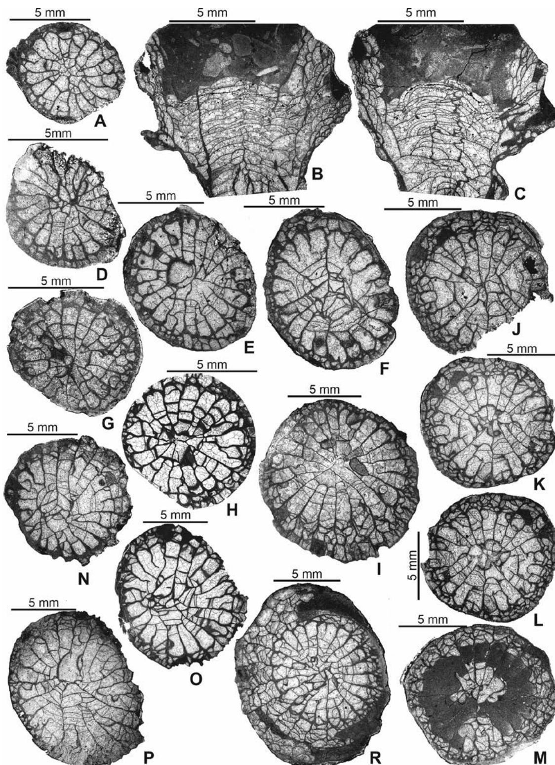
Text-fig. 5. Yuanophylloides ( Yuanophylloides ) petilus (Cocke, 1970). Transverse sections, except when stated otherwise. A–C – USNM PAL 795332; A – late neanic/early mature growth stage, B, C – longitudinal sections through mature growth stage and calice. D–F – USNM PAL 795333; D – late neanic/early mature growth stage, E, F – mature growth stage. G–I – USNM PAL 795334; G, H – late neanic/early mature growth stage, I – mature growth stage. J–M – USNM PAL 795335, mature growth stage. N–P – USNM PAL 795336; N, O – late neanic/early mature growth stage, P – early mature growth stage. R – USNM PAL 795337, mature growth stage; rejuvenated in part. For stratigraphic positions see text.
