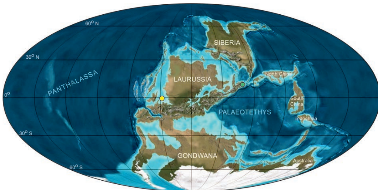
Text-fig. 3. Late Pennsylvanian paleogeography (map by Ron Blakey via Wikipedia under CC-BY-SA & GFDL); yellow dot marks the position of the study area in Texas, USA; green dot marks the approximate position of the Donets Basin in Ukraine.
