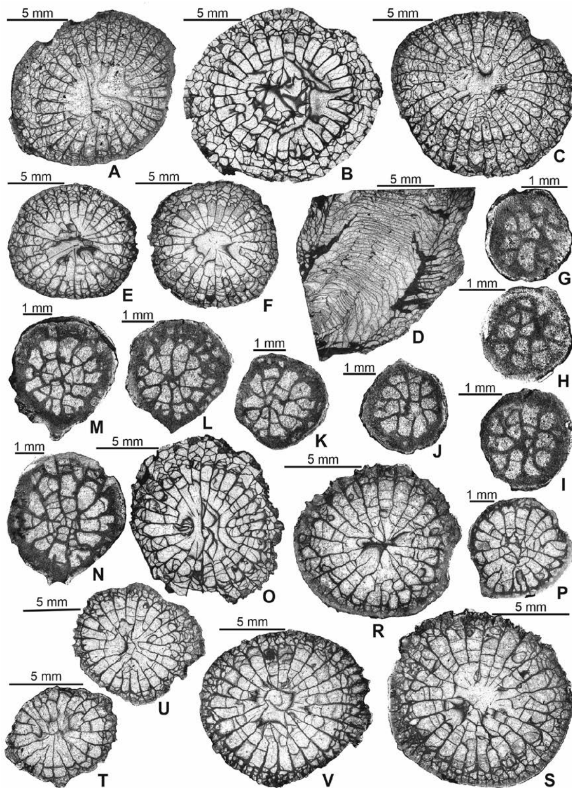
Text-fig. 9. Yuanophylloides (Patulaxis) molestus sp. nov. Transverse sections, except when stated otherwise. A–D – USNM PAL 795355; A–D – mature growth stage, D – centric longitudinal section. E, F – USNM PAL 795356, mature growth stage. G–O – USNM PAL 795357; G–N – neanic growth stage, O – mature growth stage. P–S – USNM PAL 795358; P – late neanic/early mature growth stage, R, S – mature growth stage. T–V – USNM PAL 795359; T – late neanic/early mature growth stage, U – early mature growth stage, V – mature growth stage. For stratigraphic positions see text.
