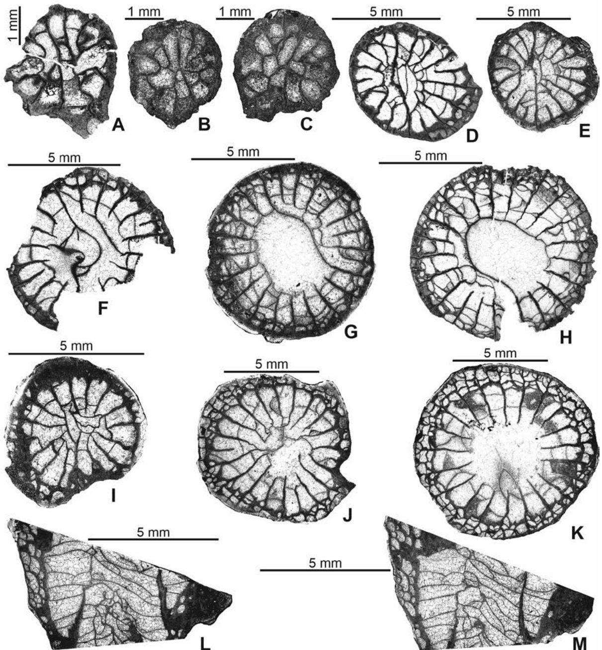
Text-fig. 15. Yuanophylloides ( Patulaxis ) sp. Transverse sections, except when stated otherwise. A–H – USNM PAL 795401; A–C – neanic growth stage, D, E – late neanic/early mature growth stage, F–H – mature growth stage; I–M – USNM PAL 795402; I – late neanic/early mature growth stage, J, K – mature growth stage, L, M – longitudinal sections; L – eccentric, M – almost centric. For stratigraphic positions see text.
