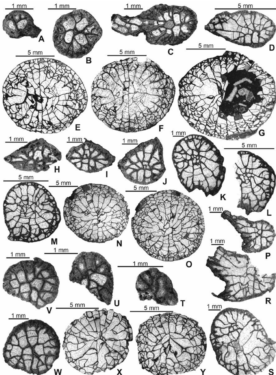
Text-fig. 4. Yuanophylloides ( Yuanophylloides ) petilus (Cocke, 1970). Transverse sections. A–G – USNM PAL 795328; A – brephic or early neanic growth stage, B–D – neanic growth stage, E–G – mature growth stage. H–O – USNM PAL 795329; H–L – neanic growth stage, M – late neanic early mature growth stage, N, O – mature growth stage. P–S – USNM PAL 795330; P, R – neanic growth stage, S – late neanic/early mature growth stage. T–Y – USNM PAL 795331; T–W – neanic growth stage, X – late neanic/early mature growth stage, Y – mature growth stage. For stratigraphic positions see text.
