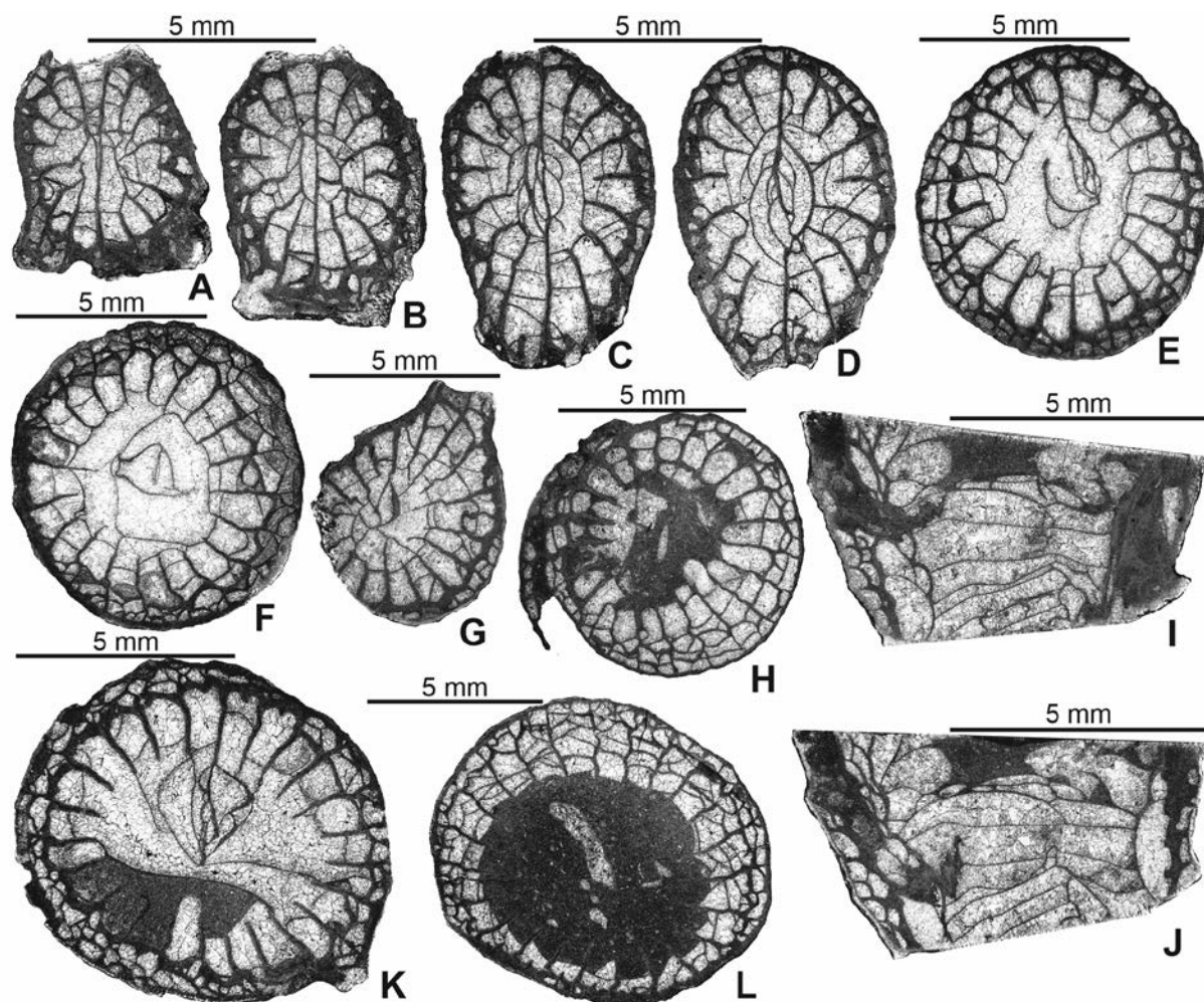
Text-fig. 7. Yuanophylloides ( Yuanophylloides ) perplexus (Cocke, 1970). Transverse sections, except when stated otherwise. A–F – USNM PAL 795349; A–C – neanic growth stage, D – late neanic/early mature growth stage, E, F – mature growth stage. G–J – USNM PAL 795350; G – neanic growth stage, H – mature growth stage, I, J – longitudinal sections; I – centric, J – slightly eccentric. K, L – USNM PAL 795351; K – mature growth stage, L – calice reduced in size. For stratigraphic positions see text.
