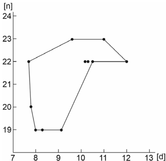
Text-fig. 6. Yuanophylloides ( Yuanophylloides ) petilus (Cocke, 1970); n:d values of selected specimens. Abbreviations: d – diameter, n – number of septa.
