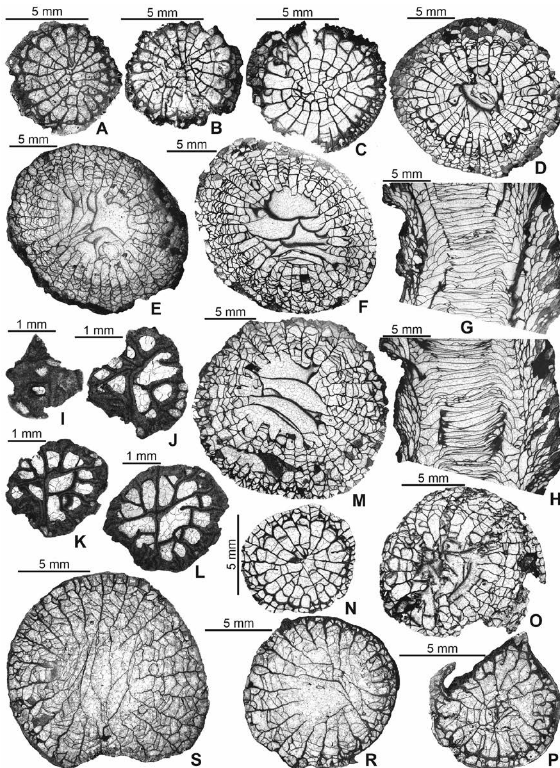
Text-fig. 12. Yuanophylloides (Patulaxis) parvus sp. nov. Transverse sections, except when stated otherwise. A–H – USNM PAL 795385, holotype; A, B – late neanic growth stage, C – late neanic/early mature growth stage, D–F – successive sections of mature growth stage, G, H – longitudinal sections; G – slightly eccentric, H – centric. I–M – USNM PAL 795386; I–L – neanic growth stage, M – mature growth stage. N, O – USNM PAL 795387; N – late neanic/early mature growth stage, O – mature growth stage. P–S – USNM PAL 795388; P – late neanic/early mature growth stage, R – early mature growth stage, S – mature growth stage. For stratigraphic positions see text.
