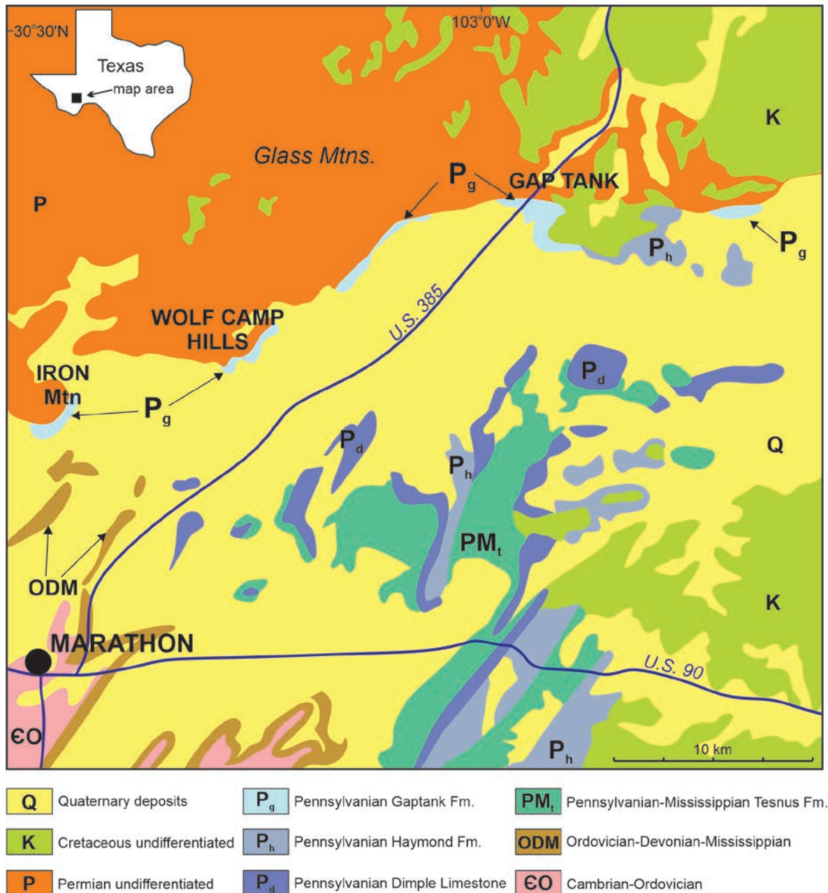
Text-fig. 1. Map of geological strata in the northern part of Marathon Basin (after Chapman and McCarty 2013, simplified). For details of the study area see Cooper and Grant (1972).
