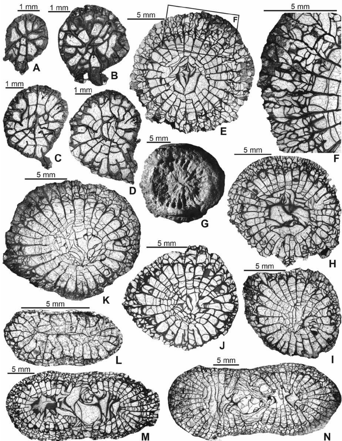
Text-fig. 10. Yuanophylloides (Patulaxis) molestus sp. nov. Transverse sections. A–G – USNM PAL 795360; A–C – neanic growth stage, D – late neanic/early mature growth stage, E – mature growth stage, F – complex dissepimentarium and differentiated length of minor septa; enlarged from E. G – calice. H – USNM PAL 795361, mature growth stage. I–K – USNM PAL 795362, successive sections of mature growth stage. L–N – USNM PAL 795363, composed of two calices surrounded by common external wall. L – late neanic/early mature growth stage, M, N – mature growth stage. For stratigraphic positions see text.
