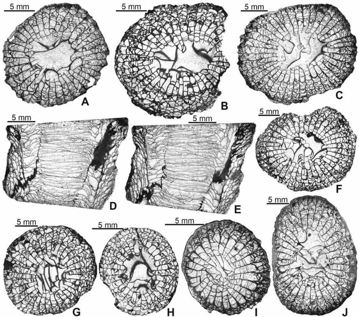
Text-fig. 13. Yuanophylloides (Patulaxis) parcus sp. nov. Transverse sections, except when stated otherwise. A–E – USNM PAL 795389; A–C – successive mature growth stage, D, E – longitudinal sections. F – USNM PAL 795390, mature growth stage. G – USNM PAL 795391, mature growth stage. H – USNM PAL 795392, mature growth stage. I, J – USNM PAL 795393, mature growth stage. For stratigraphic positions see text.
