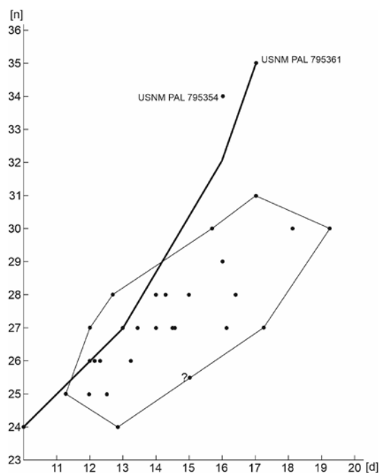
Text-fig. 11. Yuanophylloides (Patulaxis) molestus sp. nov. N:d values of selected specimens. Typical values contoured. Values of two specimens that show typical morphology of species differ. Values of one of them, starting from neanic and ending with mature growth stage connected by bold line. Abbreviations: d – diameter, n – number of septa.
