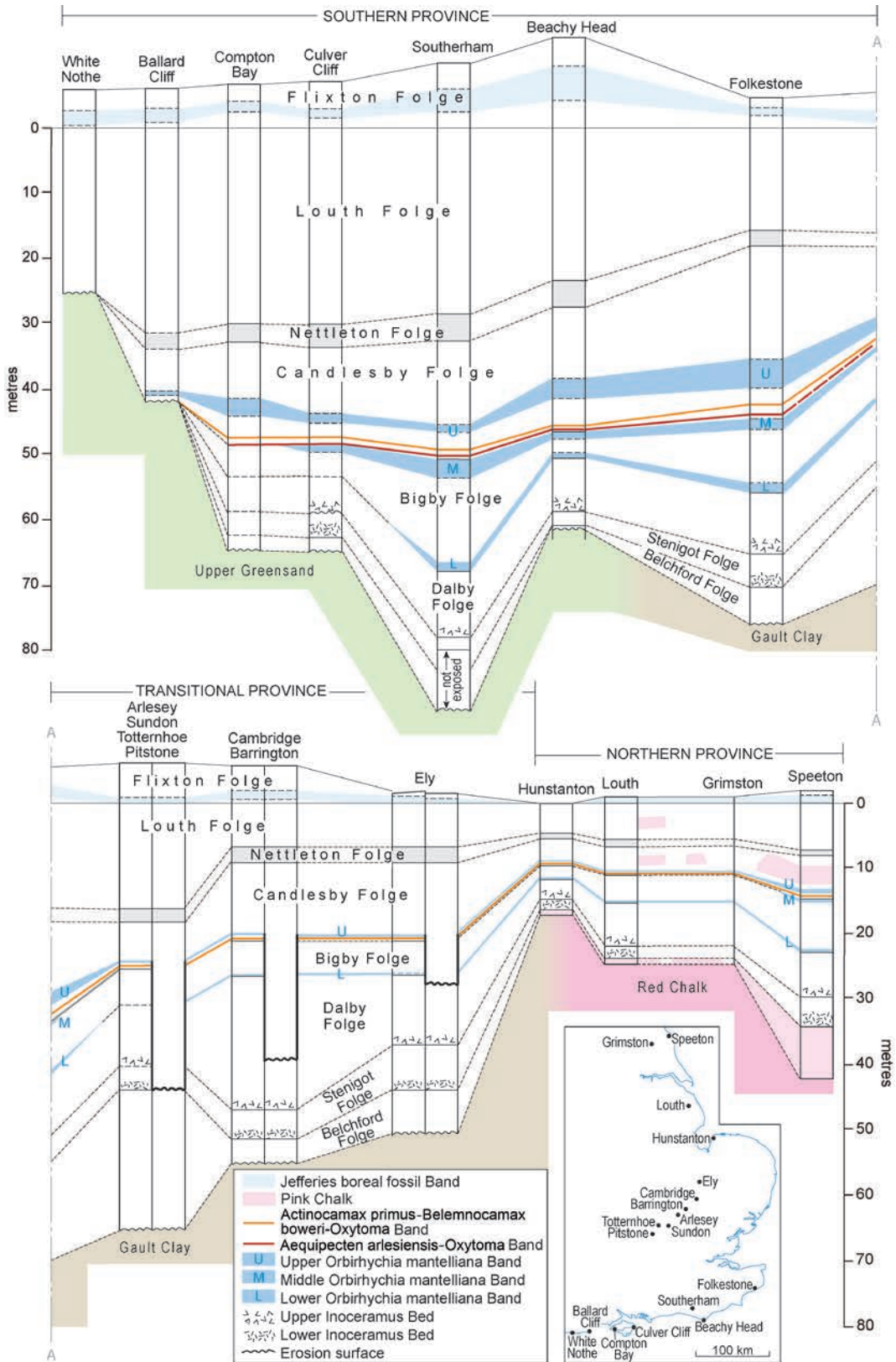
Text-fig. 6. Correlation in the Cenomanian Chalk of the Northern, Transitional and Southern provinces of England based upon Folgen and inter-regional marker bands.
