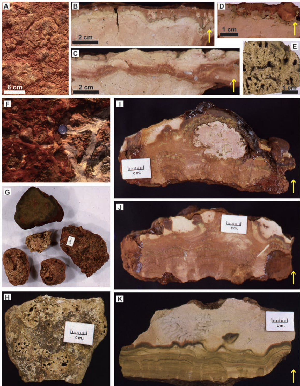
Text-fig. 12. Sedimentary features at the top of the Red Chalk and the base of the overlying Belchford Folge. A – Red Chalk, Hunstanton, top surface showing areas of bored lithified limestone and stromatolite “crust”; B, C – Red Chalk, Hunstanton: vertical sections through the stromatolite “crust”, the underlying pale pink limestone, and its bored upper surface; D, E – Red Chalk, Rosin Hill: bored top surface of the Red Chalk. F. Base of the Paradoxica Bed, Hunstanton: plan view showing the basal stromatolite columns, the overlying band of bored pebbles and callianaspid burrows; G, H – Bored limestone pebbles and a sandstone pebble from the pebble bed near the base of the Paradoxica Bed; I, J, K – Vertical section through the base of the Paradoxica Bed showing the stromatolite columns cross-cut by late diagenetic banded iron oxide staining that encompasses a bored pebble (I) and cross-cuts a fossil sponge (K).
