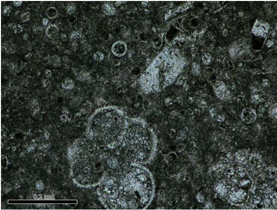
Text-fig. 18. Thin-section of the arenaceous silt-grade well-cemented chalk of the Nettleton Stone Band, Taylor Cove, Speeton (Text-fig. 22). This band has a high bulk specific gravity (2.52; porosity 6.70%, acid insoluble residue by weight 5.10%).
