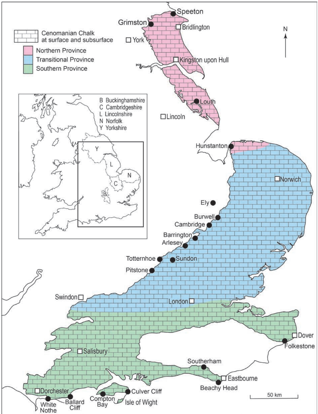
Text-fig. 3. Distribution of outcrop, subcrop and the provinces of the Cenomanian Chalk of England. The insert shows county names mentioned in the text. All locations and key localities in the Transitional and Southern provinces are shown.
