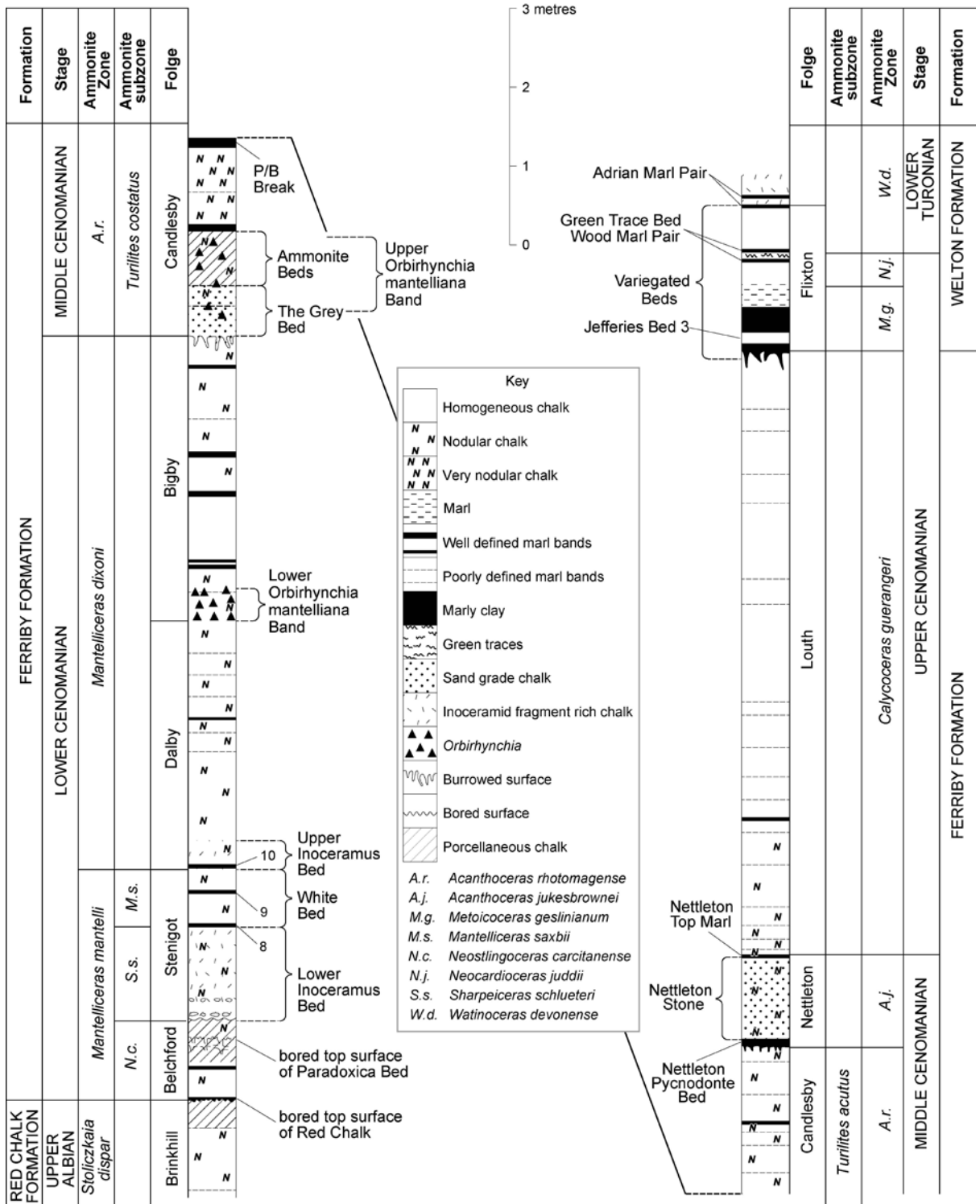
Text-fig. 8. Relationship between the eight Cenomanian folgen and the Ferriby Formation and the basal part of the Welton Formation at South Ferriby, Lincolnshire.
