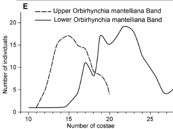
Text-fig. 21. Histograms showing the pattern of costae numbers in Orbirhynchia from the Lower and Upper Orbirhynchia mantelliana bands in the Northern Province of England.
