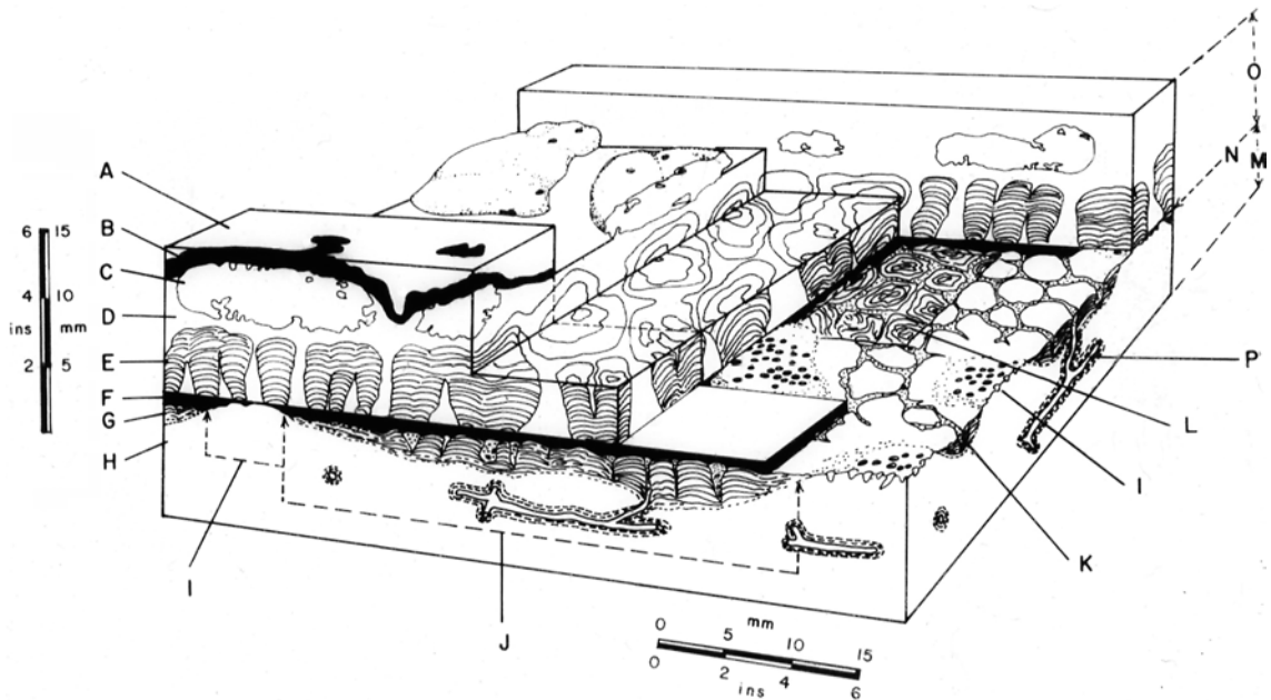
Text-fig. 13. Block diagram of the structure and inter-relations between the top of the Red Chalk Formation and the base of the Paradoxica Bed at Hunstanton, Norfolk. A – Pink chalk at the base of the Paradoxica Bed; B – Hard brown ochre to brown iron oxide layer formed by the replacement of chalk during late non-intrinsic diagenesis – running parallel to this are numerous very fine ochreous bands that cross-cut earlier diagenetic structures; C – Pebbles of pink limestone extensively bored and glauconite stained. Up to 18 cm in maximum dimension; D – Basal chalk of the Paradoxica Bed infilling between stromatolite columns; E – Stromatolite columns of alternating thin dark green glauconitic clay layers and thicker reddish calcareous layers; F – Friable red clay with brown stained sand grains and small pebbles; G – Stromatolite layer at the top of the Hunstanton Red Chalk Formation consisting of irregular sheets or vertical columns (polygonal in plan) of alternating thin (approximately 0.1 mm) ochreous to red carbonate layers; H – Pale pink chalky laminae with irregular, vertically elongated patches of coarse sand grains: gradational junction with G; I – Higher surfaces penetrated by undistorted borings or burrows (1–1.5 mm diameter) – surfaces, borings and burrows coated by blackish green glauconite skins [ <1 mm thick]; J – Topographic lows (up to 19 mm below the higher bored regions) on the top surface of the Red Chalk; K – Reticulated network of soft pink chalk with numerous sand grains and small pebbles infilling between stromatolitic columns; L – Horizontal section through stromatolites showing internal structure; M – Top part of the Red Chalk; N – Junction of Red Chalk and Ferriby Formation; O – Basal part of Paradoxica Bed; P – Undistorted sediment filled reticulated burrow system with Liesegang glauconite staining of its walls, paling into the matrix, connected to slightly distorted sediment-filled tubes (1–2 mm diameter) with walls stained by thin skin of blackish-green glauconite.
