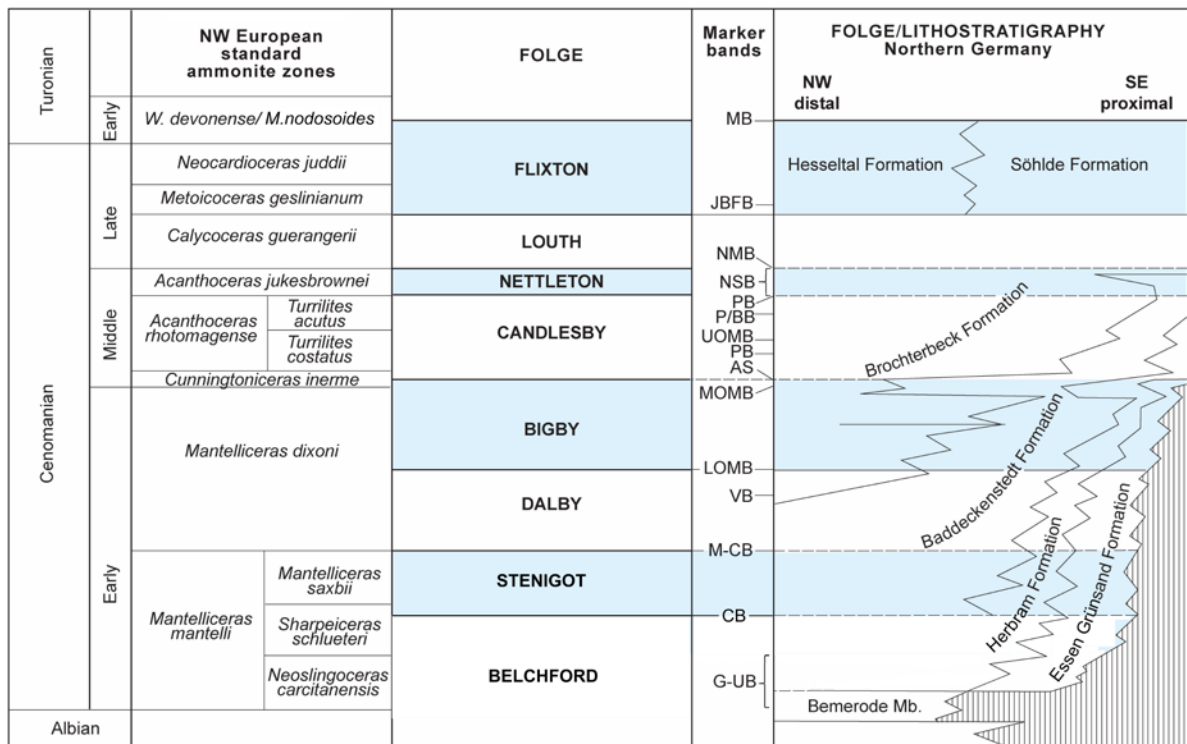
Text-fig. 20. Interpretative and predictive lithofacies model showing the distribution of the eight Cenomanian folgen in relation to the lithological formations of northern Germany. Based in part on Wilmsen (2007, text-fig. 2). G-UB – Gryphaeoides/Ultimus Band; CB – Crippsi Band; M-CB – Mariella/Crippsi Band; VB – Virgatus Band; LOMB – Lower Orbirhynchia mantelliana Band; MOMB – Middle Orbirhynchia mantelliana Band; AS – Arlesiensis Band; PB – Primus Band; UOMB – Upper Orbirhynchia mantelliana Band; P/BB – Planktonic/benthonic Break; PB – Pycnodonte Band; NSB – Nettleton Stone Band; NMB – Nettleton Marl Band; JBFB – Jefferies Boreal Fossil Band; MB – Mytiloides Band.
