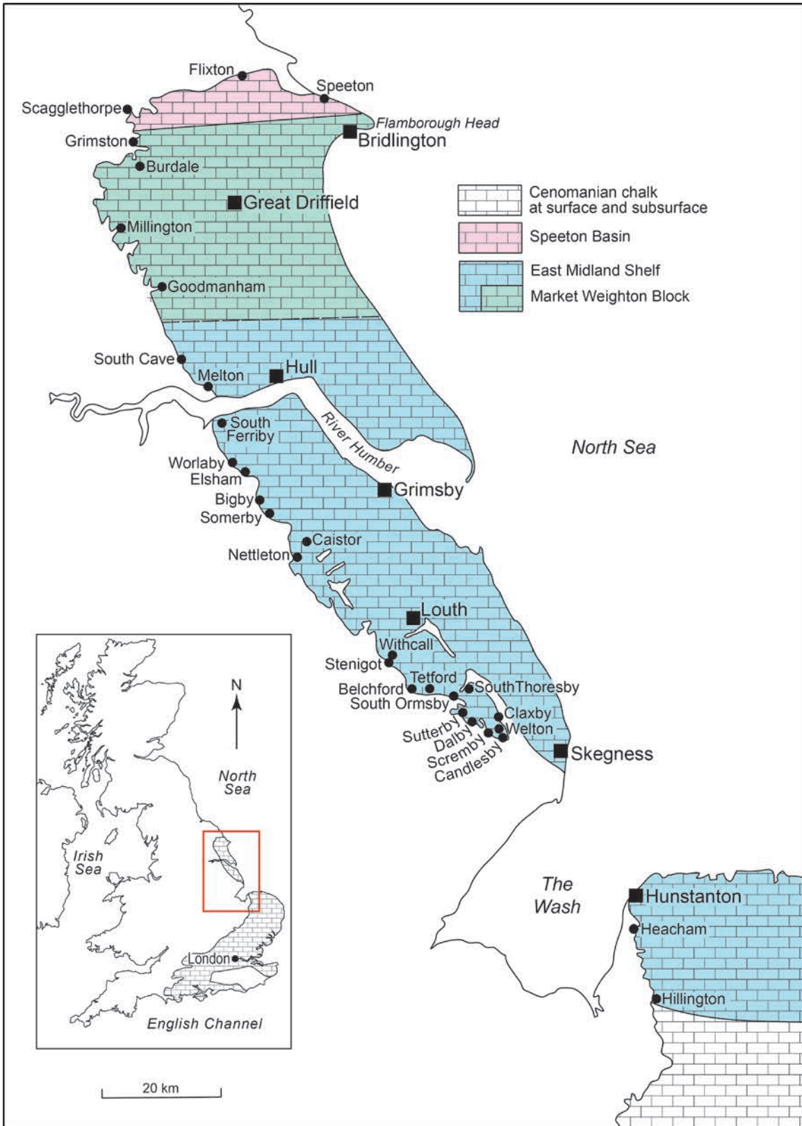
Text-fig. 5. Distribution of the Cenomanian Chalk at the surface and sub-surface in the Northern Province of England and in the adjacent part of the Transitional Province showing the locations and the extent of the Midland Shelf, Market Weighton Block, and the Speeton Basin.
