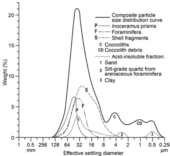
Text-fig. 17. Particle size distribution curves for the total sample and the various components of the Burwell Rock (Candlesby Folge), Burwell, Cambridgeshire (after Black 1980, p. 65).
