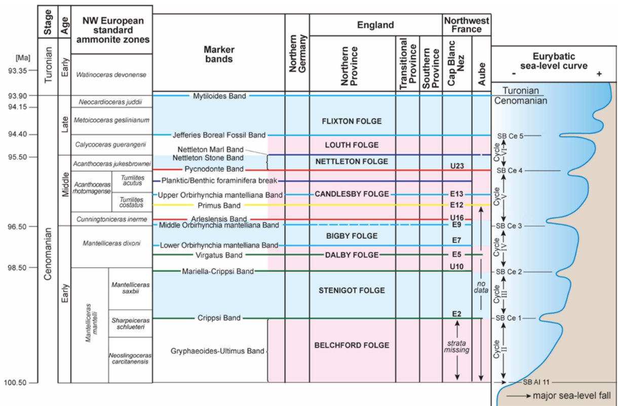
Text-fig. 2. The extent of the eight folgen of the Cenomanian Chalk strata and their inter-regional marker bands in England, northern Germany and northwest France. Their relationship is shown to (a) lithofacies Cycles II-VI of the Northern Chalk Province, (b) the sequence stratigraphy of northern Germany and northwest France, and (c) the standard ammonite zones for northwest Europe. Based in part on Janetschke et al. (2015), Amédéo and Robaszynski (1999). Radiometric dates are based on Ogg et al. (2012).
