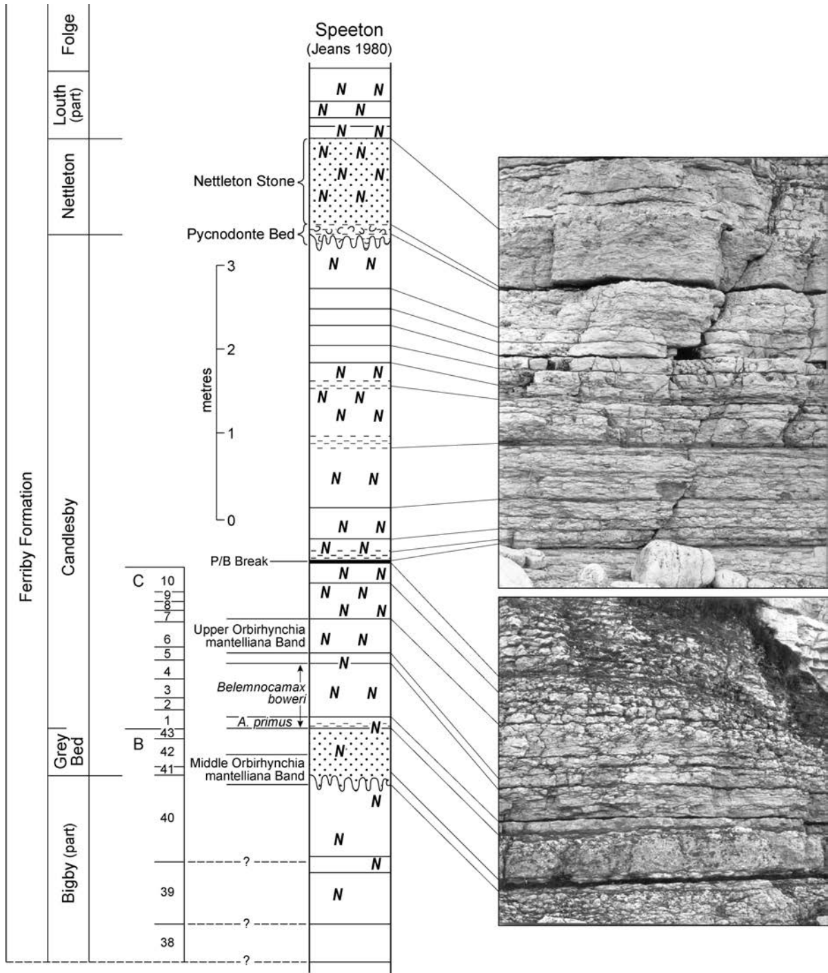
Text-fig. 22. Middle Cenomanian sequence at Jake and Taylor Coves, Speeton showing the regional marker bands and contrasting the interpretations of the section by Jeans (1980, fig. 16) and Paul et al. (1994, fig. 11).
