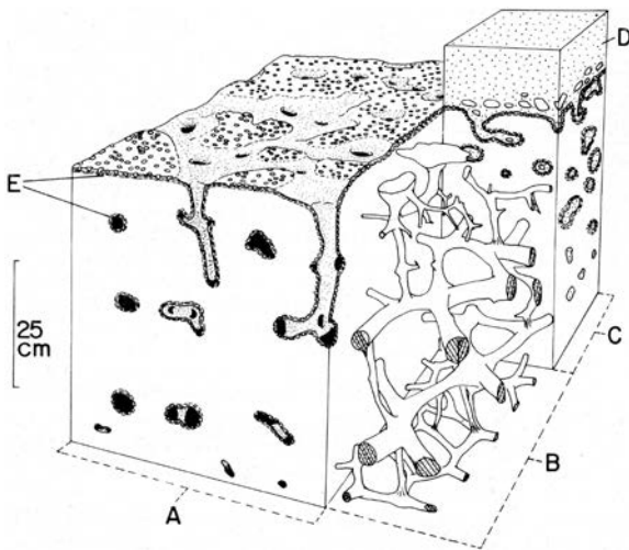
Text-fig. 14. Structure of the Paradoxica Bed at Hunstanton prior to pressure dissolution. A – Original form when exposed on the Chalk seafloor with a bored flat surface and the unbored depressions leading into the glauconite stained callianaspid burrow system (Jeans et al. 2014b); B – Excavated system of burrows now infilled with grey gritty chalk; C – The relationship between the Paradoxica Bed and the overlying Lower Inoceramus Bed; D – Basal part of the Paradoxica Bed; E – Liesegang zones of glauconite staining.
