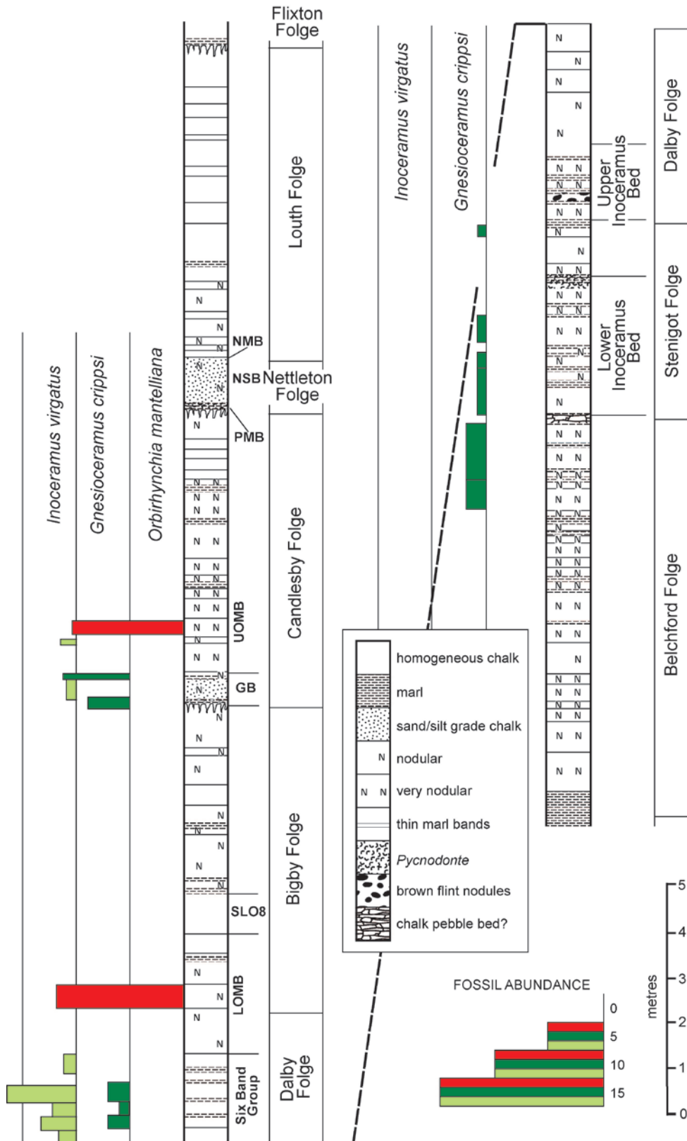
Text-fig. 9. Lithological sequence of the Cenomanian folges in the cliffs at Speeton, Yorkshire. The distribution of Inoceramus virgatus and Gnesioceramus crippei is shown in relation to various marker bands. Key for marker bands, see Text-fig. 10.
