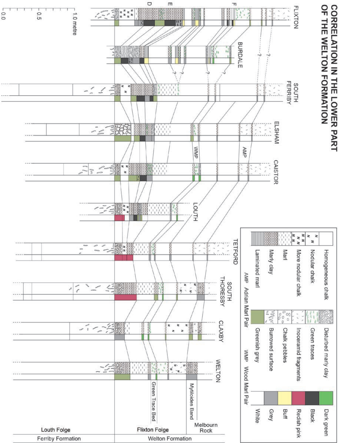
Text-fig. 19. Correlation chart in the Flixton Folge within the Welton Formation, Northern Province.
