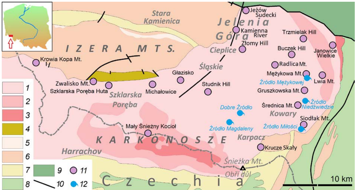
Text-fig. 1. Eastern part of the Karkonosze Variscan pluton and its metamorphic envelope: 1 – porphyritic monzogranite and granodiorite; 2 – medium-grained biotite monzogranite; 3 – fine-grained monzogranite; 4 – hornfels; 5 – leucogranite; 6 – gneiss; 7 – chlorite-mica schists; 8 – mafic metamagmatites and schists; 9 – mainly mafic metamagmatic rocks; 10 – faults; 11 – fluorite sampling locations; 12 – springs. Geological background after Krenz et al. (2001), modified. Insert – location in Poland.
