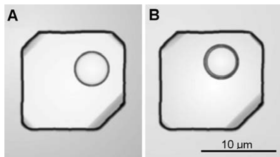
Text-fig. 15. Inclusion with CO 2 in fluorite at room temperature (A) and cooled to +2°C (B), thin rim of liquid carbon dioxide around gas bubble is visible. Zwalisko Mt.
