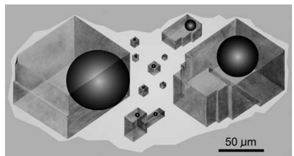
Text-fig. 7. Fluid inclusion in fluorite, originally of abnormal shape and due to recrystallization divided into several daughter inclusions with vacuole faces of cube. The initial shape is outlined by the light (pale violet) part in distinctly not recrystallized darker fluorite. Note the different volume proportions of gas bubble and liquid phase in various daughter inclusions. Michałowice quarry.
