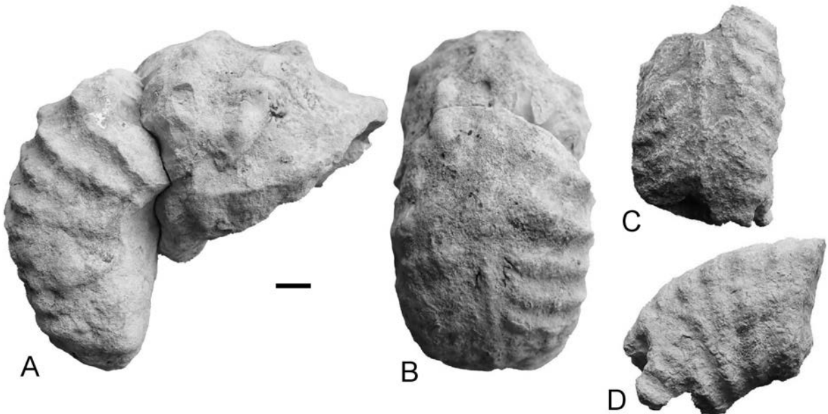
Text-fig. 12. Pervinqueria (Subschloenbachia) perinflata (Spath, 1922). A, B – OUMNH KX.17290, from the 20 m level; C, D – OUMNH KX.17293, collected loose at the same level, Aït Lamine Formation, Oued Abouda, Upper Albian, Pervinqueria (Subschloenbachia) perinflata Zone. Scale bar 10 mm.
