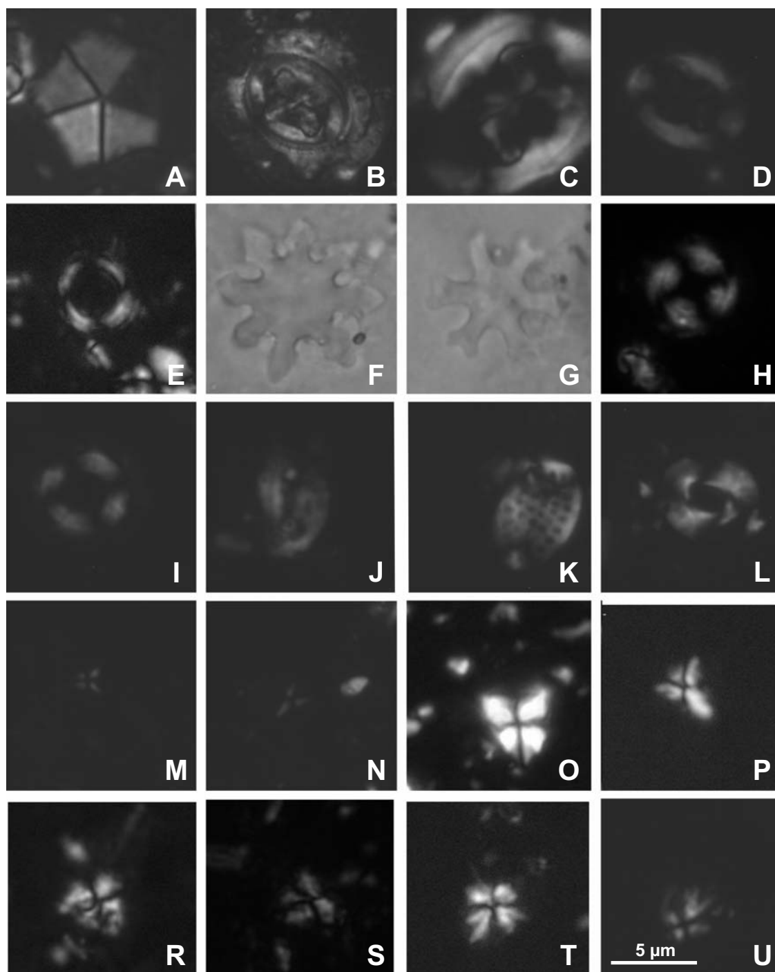
Text-fig. 6. Calcareous nannoplacton LM microphotographs of typical species, scale bar is the same for all photographs (Oszczypko and Oszczypko-Clowes 2010). A – Braarudosphaera bigelowii , Kremna Fm., sample WP242/1/2010. B – Chiasmolithus gigas , Kremna Fm., sample WP329/2010. C – Chiasmolithus grandis , Kremna Fm., sample WP330/B/2010. D – Chiasmolithus solitus , Kremna Fm., sample WP330/B/2010. E – Coronocyclus nitescens , Poprad Sandstone Mb. of the Magura Fm., sample BW 505-1. F – Discoaster binodosus , Kremna Fm., sample WP330/C/2010. G – Discoaster deflandrei , Kremna Fm., sample 104b/2010. H – Ericsonia formosa , Kremna Fm., sample 9/07/N. I – Ericsonia robusta , Kremna Fm., sample WP917/2/2011. J – Helicosphaera compacta , Poprad Sandstone Mb. of the Magura Fm., sample BW 505-2. K – Ponthosphaera multipora , Kremna Fm., sample H 1. L – Reticulofenestra dictyoda , Kremna Fm., sample WP79/2007. M , N – Sphenolithus calyculus , Kremna Fm., sample WP330/C/2010. O – Sphenolithus conicus , Kremna Fm., sample 104b/2010. P – Sphenolithus delphix , Bukry, Magura Fm., sample BW 1. R , S – Sphenolithus disbelemnus , Kremna Fm., sample WP633/2011. T , U – Sphenolithus dissimilis , Kremna Fm., sample 104c/2010.
