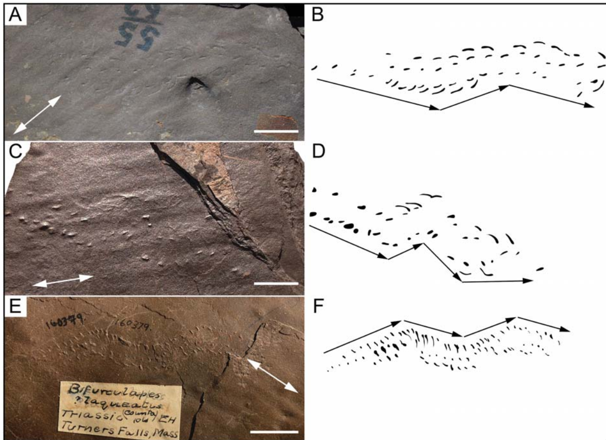
Text-fig. 2. Bifurculapes laqueatus Hitchcock, 1858 exhibiting evidence of trackmaker interaction with flowing water. A, B – Photograph and interpretive drawing of trackway on ACM ICH 55/62. C, D – Photograph and interpretive drawing of trackway on ACM ICH 305. E, F – Photograph and interpretive drawing of trackway on YPM IP 160379. The lines with double arrowheads in the photographs indicate the orientation of the long axes of the current lineations; the arrows in the interpretive drawings indicate the direction of travel for the trackmaker. Scale bars are 10 mm
