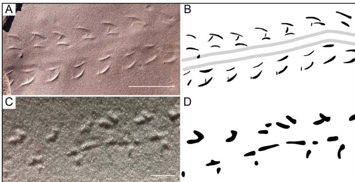
Text-fig. 3. Fossil and modern trackways for comparison. A, B – Photograph and interpretive drawing of Bifurculapes laqueatus Hitchcock, 1858 on ACM ICH 300. C, D – Photograph and interpretive drawing of an experimentally produced trackway made by a cricket ( Acheta domestica Linnaeus, 1758) subaerially in fine-grained sand. Scale bars are 10 mm
