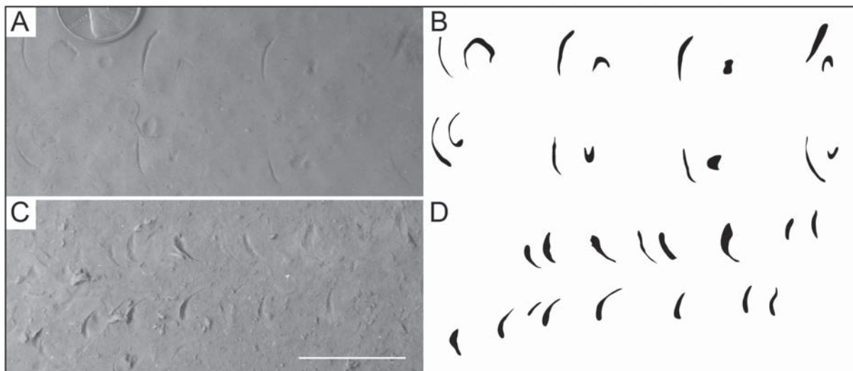
Text-fig 4. Experimentally produced aquatic insect trackways for comparison to Bifurculapes laqueatus Hitchcock, 1858. A, B – Photograph and interpretive drawing of a trackway produced by the giant water bug (Belostomatidae) Belostoma flumineum Say, 1832. C, D – Photograph and interpretive drawing of a trackway made by the whirligig beetle (Gyrinidae) Dineutus discolor Aubé, 1838. Coin in A is 19.05 mm; scale bar in C is 10 mm
