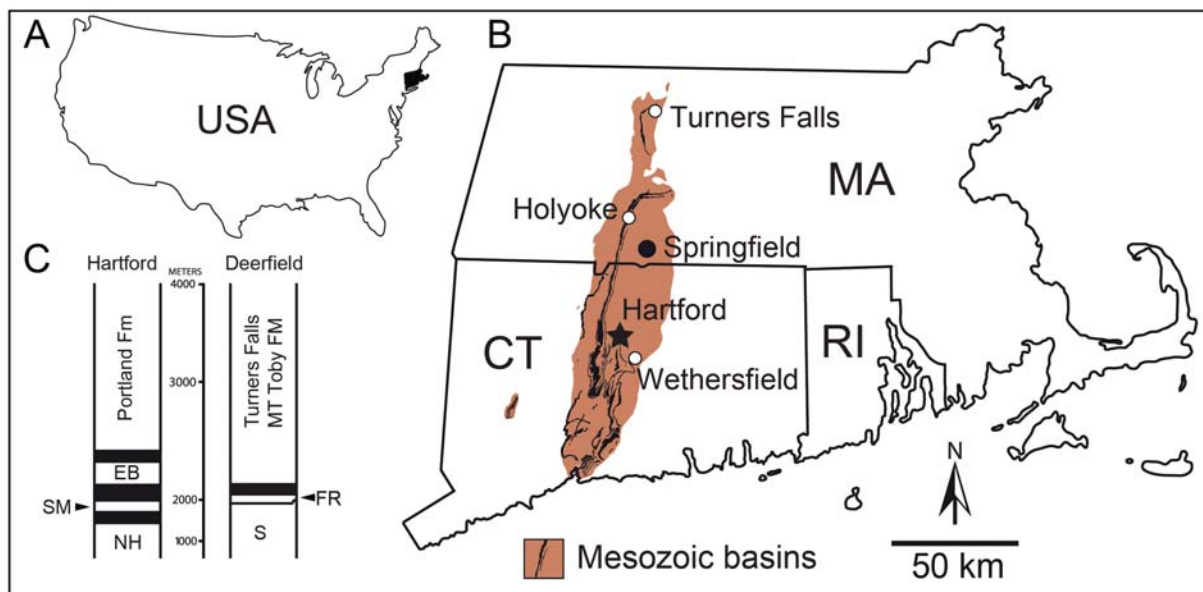
Text-fig. 1. Geological context of the Bifurculapes specimens illustrated in Text-fig. 2. A – Map of the contiguous 48 United States, showing southern New England shaded in black. B – Map of southern New England with lower Mesozoic rocks shaded. Sedimentary rocks are brown and igneous rocks are black. Turners Falls, Holyoke, and Wethersfield are locations from which Bifurculapes laqueatus Hitchcock, 1858 has been recovered regionally. Abbreviations: CT, Connecticut; MA, Massachusetts; RI, Rhode Island. C – Simplified stratigraphic columns of the Hartford and Deerfield basins. Abbreviations: EB, East Berlin Formation; FR, Fall River beds; NH, New Haven Formation; S, Sugarloaf Formation; SM, Shuttle Meadow Formation
